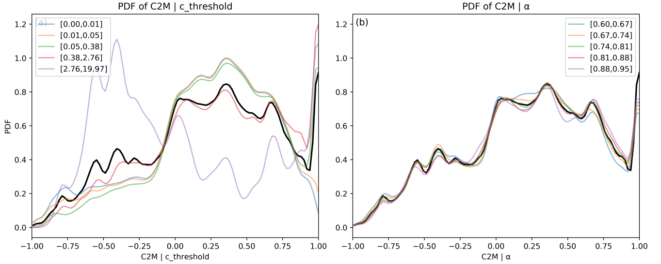
Figure 12. Shifts in C_{2M} Probability Distribution Function (PDF) depending on c\_threshold (a) and \alpha (b) range values, within irrigation reservoirs. The unconditional PDFs of the DROP model output C_{2M} , obtained when all input parameters are randomly sampled, are displayed in black. The conditional PDFs are shown in color depending on the parameter value range.
