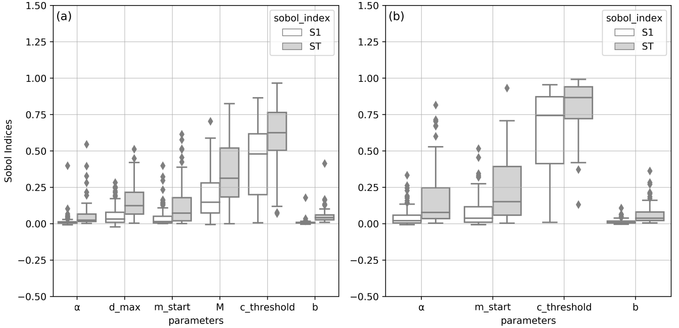
Figure 9. Distribution of first (S1) and total (ST) order Sobol indices on the modelled reservoirs for each parameter : (a) in irrigation and (b) in non-irrigation reservoirs
