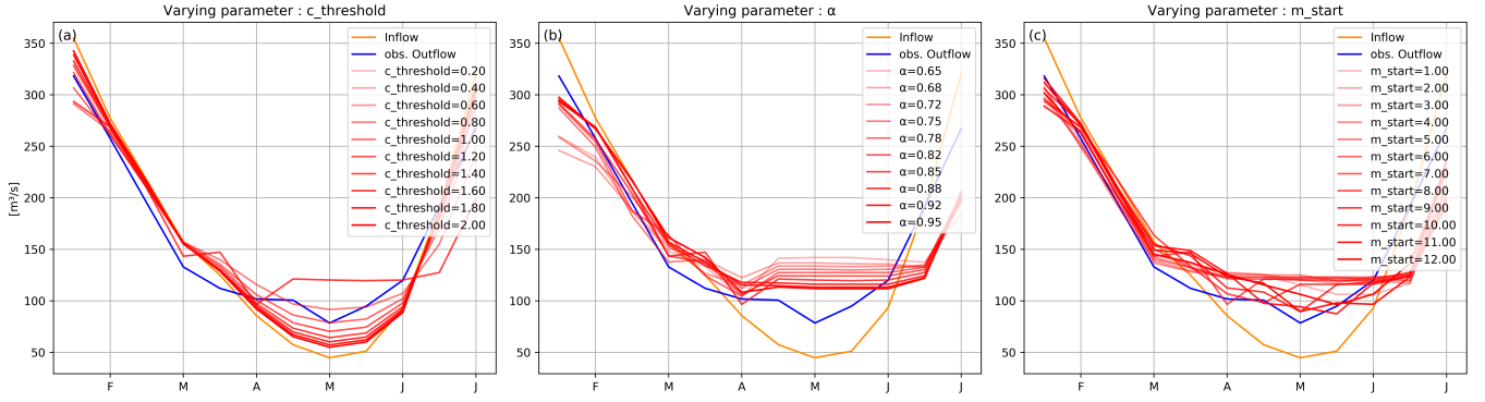
Figure 8. An example of the seasonal pattern sensitivity of the 'Alcantara II' hydroelectricity reservoir outflow to three of the DROP model parameters : (a) c_{\text{threshold}} , (b) \alpha and (c) m_{\text{start}} . The remaining parameters were set at default values (see Table 2).
