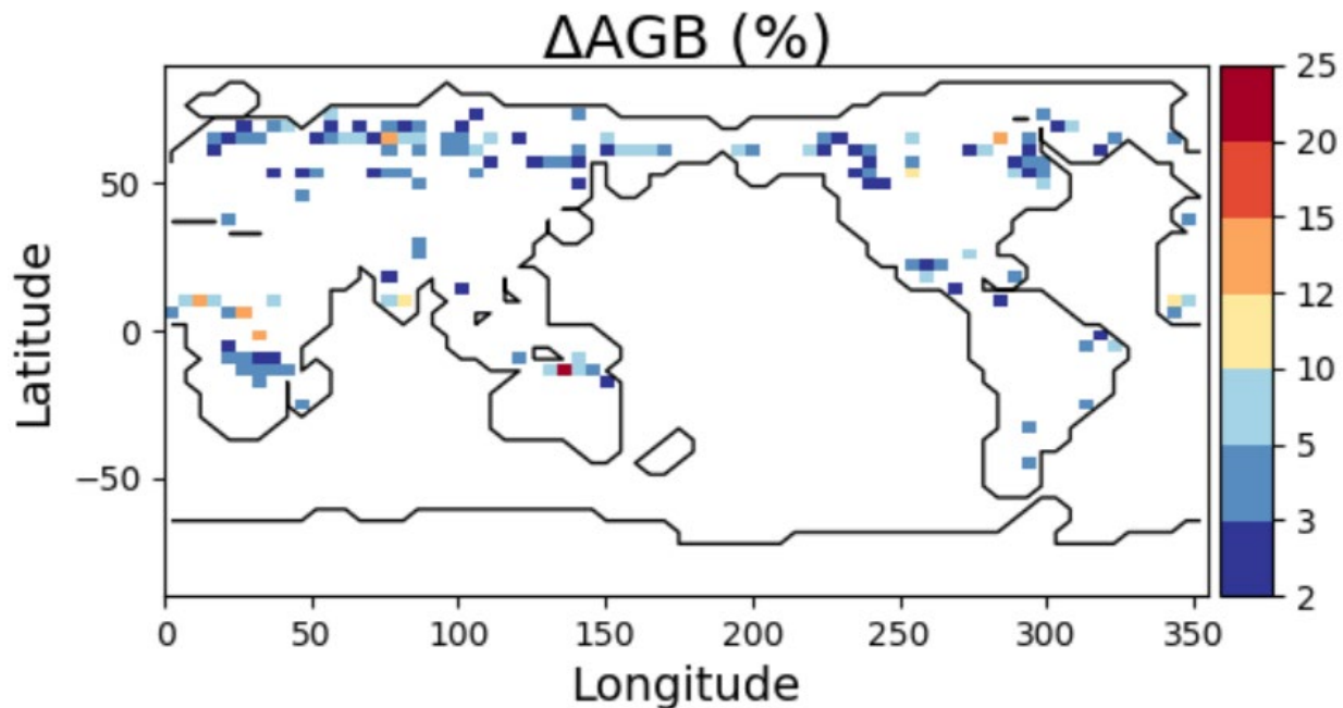
Figure R2. Percent increase of AGB using 10-min time step explicit solve
