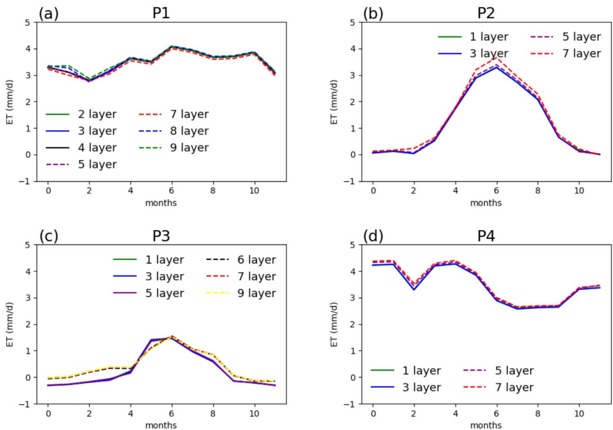
Figure R3. Evapotranspiration from single point simulations at selected locations (P1 – P4) at year 100 of the simulations.
