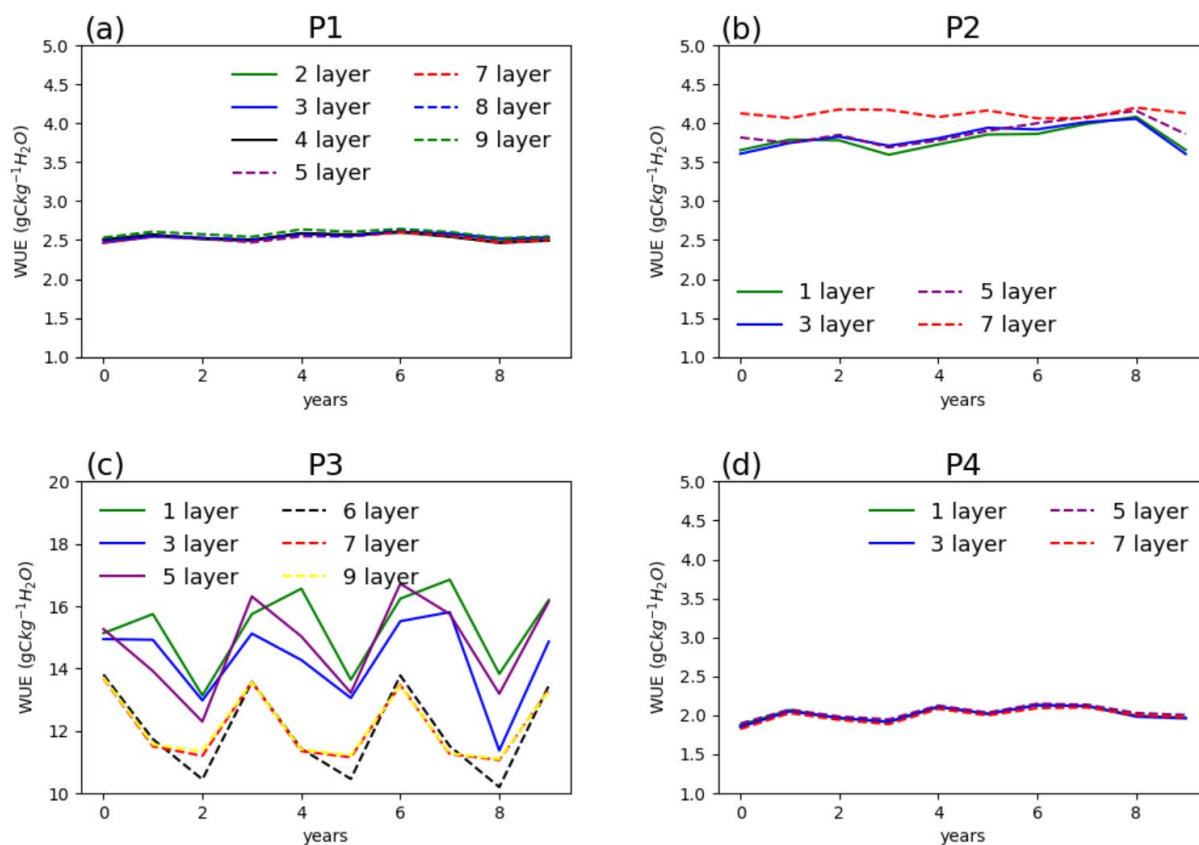
Figure R4. Annual water use efficiency (WUE) from single point simulations at selected locations (P1 – P4) during the last 10 years of the simulations.
