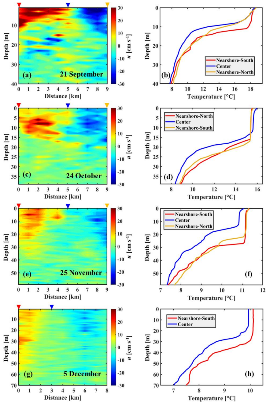
540 Figure 13. Left column: Contour plots of the measured horizontal velocity along Transect T2 (for location, see Figure 1b). Right column: Measured temperature profiles at the locations marked by corresponding colored triangles above panels in the left column: (a) and (b) 21 September 2019; (c) and (d) 24 October 2019; (e) and (f) 25 November 2019; (g) and (h) 5 December 2019. Note that all panels in the left column are plotted with the same range to highlight the seasonal change; the range of the x -axis in the right column changes with time. Colorbars show the range of horizontal velocities.
