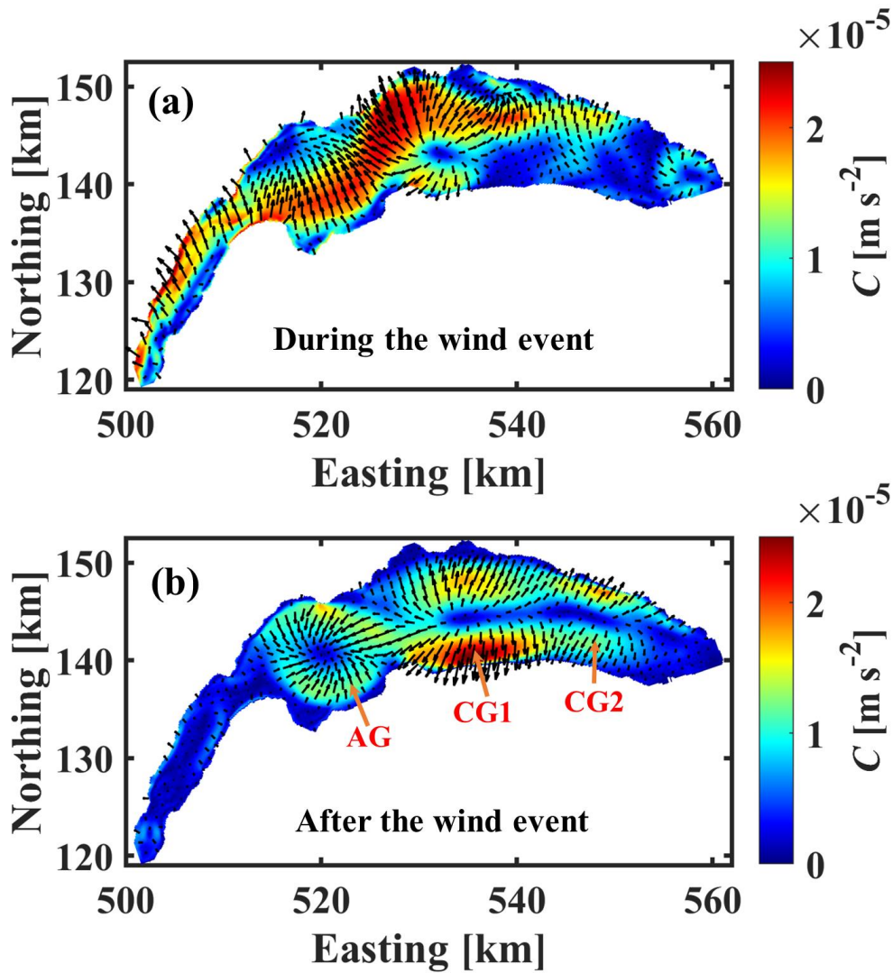
Figure 14. (a) Contribution of Coriolis term C (strength as indicated by color contours, and orientation, by arrows) to the vertically (upper 5 m of the water column) and temporally (65 h) averaged horizontal momentum equation (Eq. (6)): (a) during and (b) after the Bise event that occurred in September 2019. After the wind event, convergence can be seen at gyre AG, and divergence in the CG1 gyre area.
