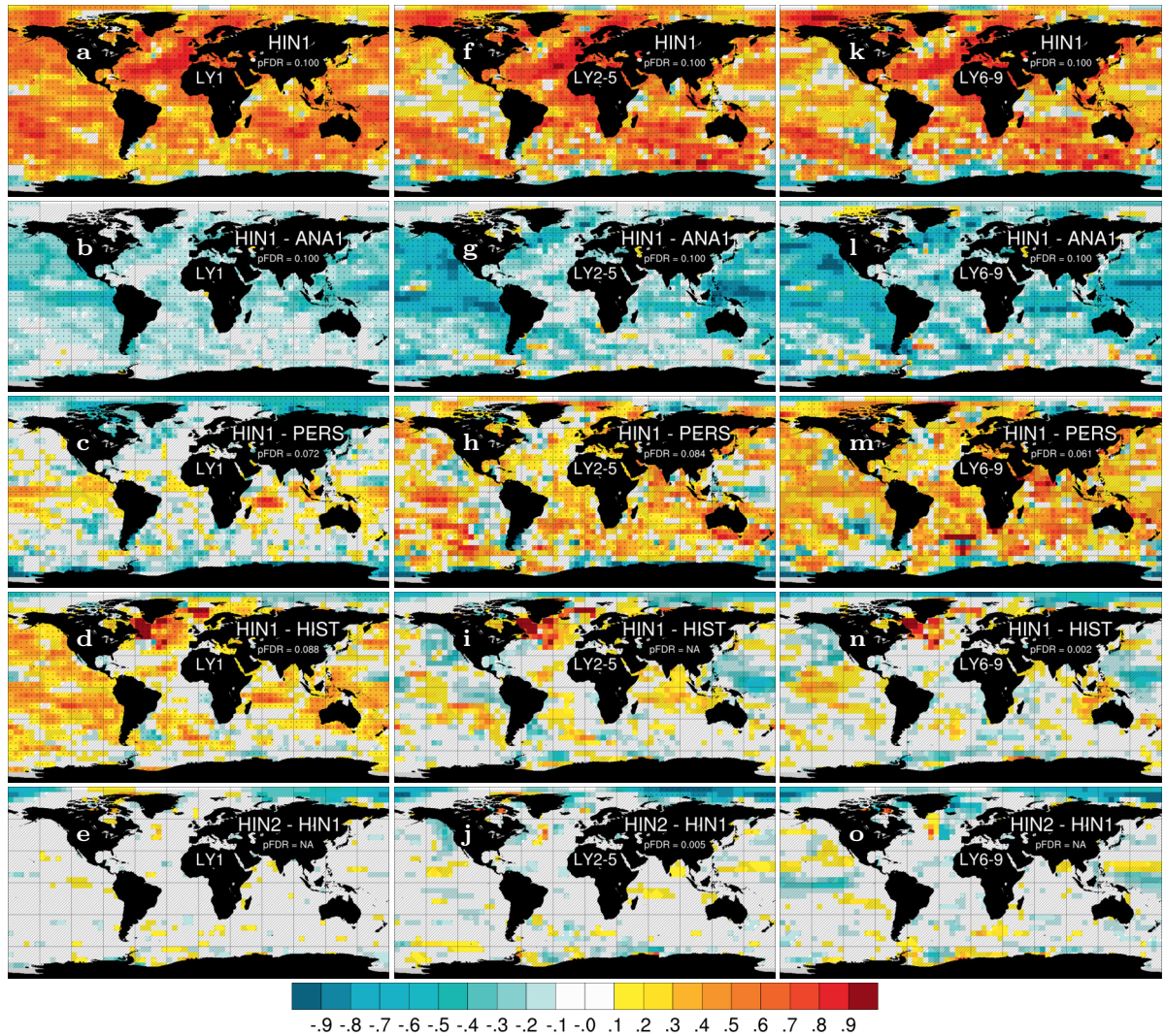
Figure D3: Original version showing ACC for 0-300 m ocean temperature.
