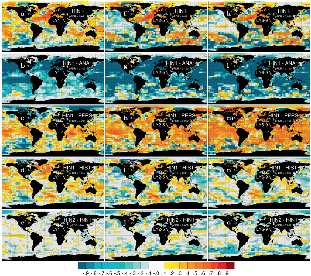
Figure D3: Alternative version showing MSSS for 0-300 m ocean temperature. The MSSS calculation follows Yeager et al. (2018).
