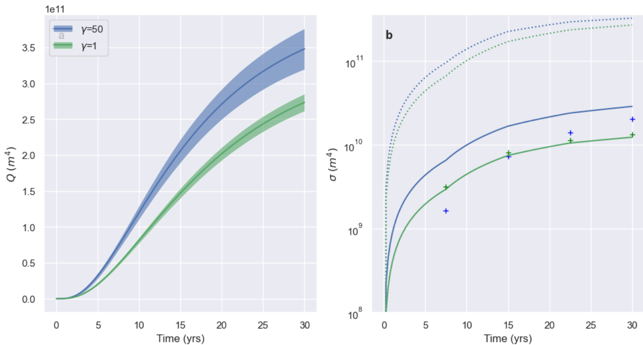
Figure 6. (a) Paths of Q_T^{IS} in \gamma_{50} experiment (blue) and \gamma_1 experiment (green). Shading shows the 1- \sigma uncertainty interval for each trajectory calculated by projecting the Hessian-based (posterior) uncertainty along the linearised trajectory. (b) Uncertainties in the time-dependent experiments over time. Dashed lines: prior uncertainties projected along the linearised Q_T^{IS} trajectory. Solid lines: Hessian-based posterior uncertainties projected along the linearised trajectory. Markers: Standard deviation of Q_T^{IS} from sampling the posterior density. In both panels, green corresponds to \gamma_{50} , and blue to \gamma_1 .
