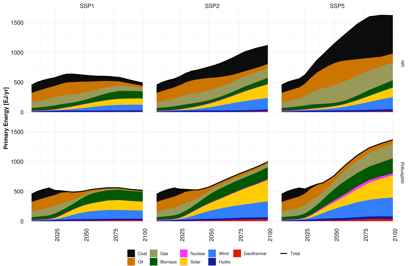
895 Figure 7: Primary energy mixes by carrier for the NPi and pkBudg900 (1.5°C) scenario of SSP1, SSP2 and SSP5.
