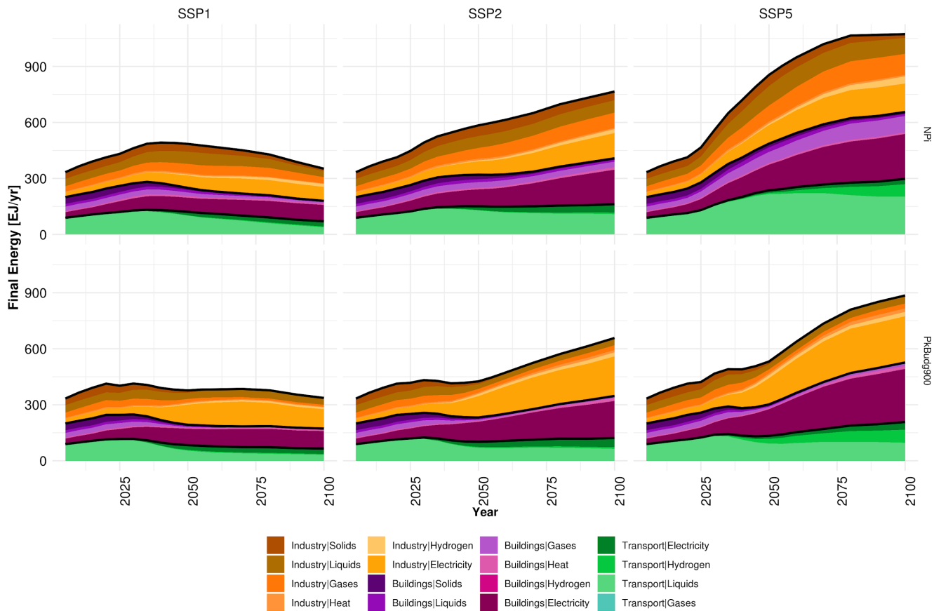
Figure 8: Final energy mixes for sectors by carrier for the NPI and pkBudg900 (1.5°C) scenario of SSP1, SSP2 and SSP5
