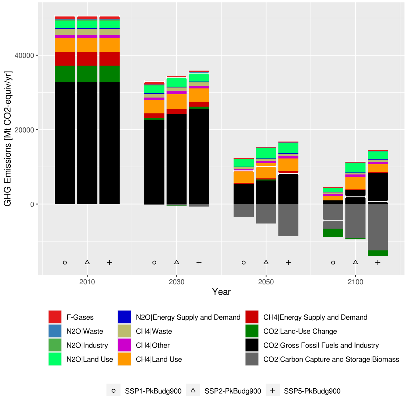
860 Figure 5: Global GHG emissions by type for the 1.5°C scenarios (pkBudg900) based on SSP1, SSP2, and SSP5. The white line shows net GHG emissions.
