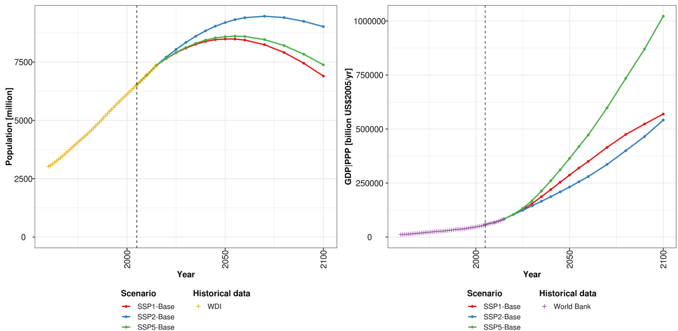
150 Figure 2: Global population and GDP trajectories for 2005 to 2100 for SSP1, SSP2 and SSP5, compared to historical data from the World Development Indicator (WDI) and (World Bank, 2012).
