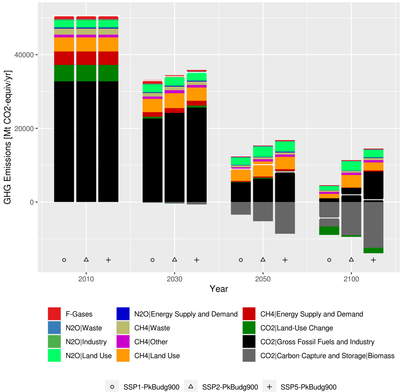
880 Figure 5: Global GHG emissions by type for the 1.5°C scenarios (pkBudg900) based on SSP1, SSP2, and SSP5. The white line shows net GHG emissions.
