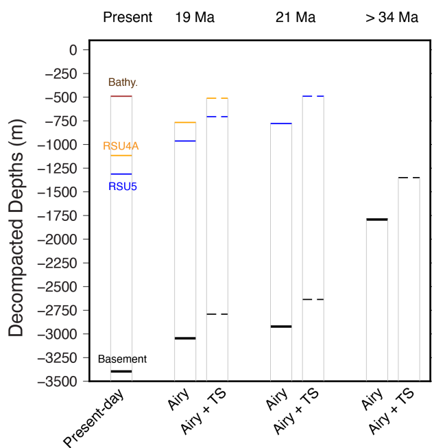
Figure 8. Backtracking steps for Western Ross Sea DSDP 270 well site. For present-day: present-day depths of basement (black), Ross Sea unconformity 5 (blue), Ross Sea Unconformity 4A (orange) and bathymetry (brown); at time of RSU4A (19 Ma), at time of RSU5 (21 Ma) and at time before glacial sediment deposition (> 34 Ma). For each time step, two backtracking are shown, one accounting for Airy isostatic correction only, and one accounting for Airy isostatic correction and thermal subsidence (dashed). Table 1 in Appendix A.
