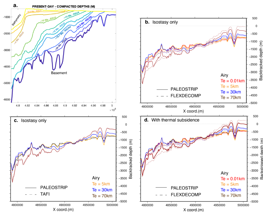
Figure 6. 2D transect BGR80-007 case study: a. Input present-day depths (m) of bathymetry (yellow), and the nine seismic unconformities, amongst which, the mid-Miocene Ross Sea Unconformity 4 (RSU4) and basement (thick blue line). Layout is from PALEOSTRIP Plot GUI. Comparison of backtracked basement depths for different but spatially uniform lithospheric elastic thicknesses ( T_e ): b. between PALEOSTRIP finite difference isostasy and Flex-Decomp (Kusznir et al., 1995) Fast Fourier Transform (wavenumber-based) isostasy model; c. between PALEOSTRIP finite difference isostasy and TAFI (Jha et al., 2017) Green’s function spectral isostasy model; d. Same as b. but accounting for thermal subsidence correction using an age of Rift = 85 Ma and a uniform \beta = 2 .
