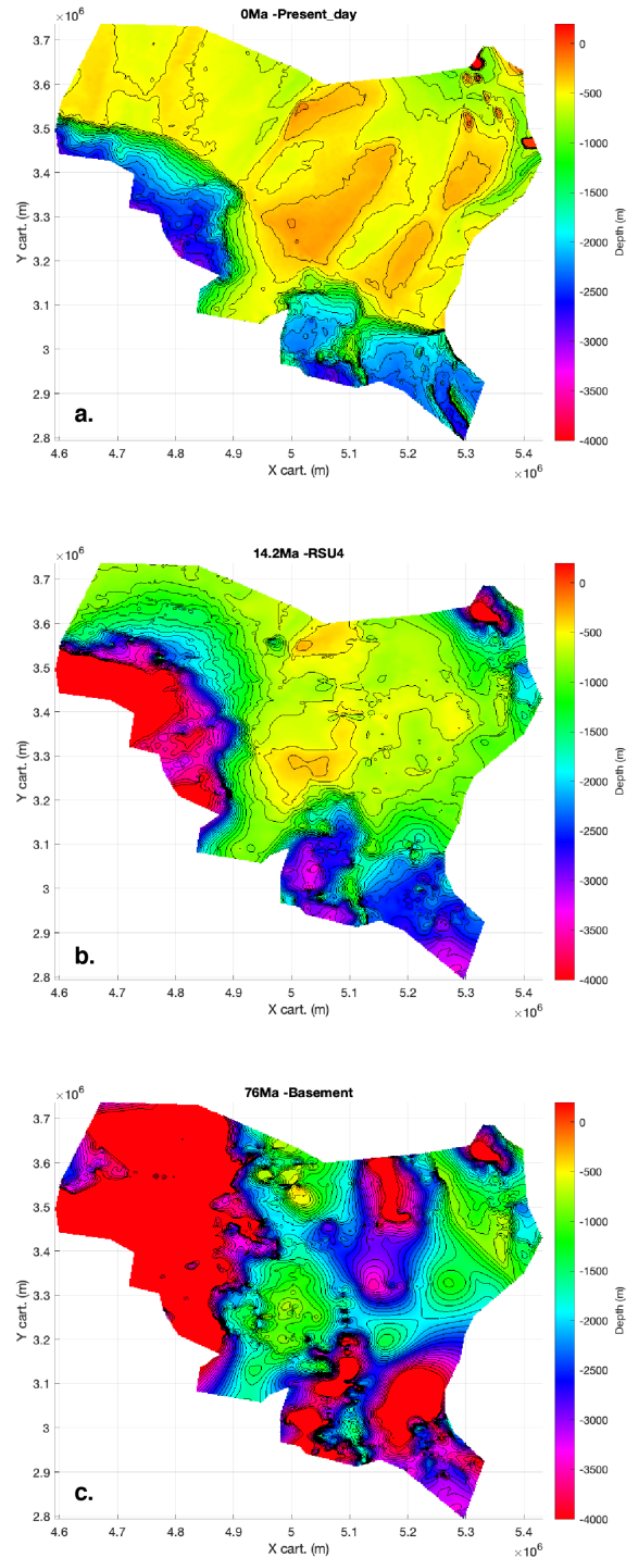
Figure 9. Initial input present-day depths (m): a. bathymetry, b. mid-Miocene unconformity RSU4 and c. basement. Layout is from PALE-OSTRIP plotting GUI. Colorscale is saturated below -4000 meters and above 200 meters.
