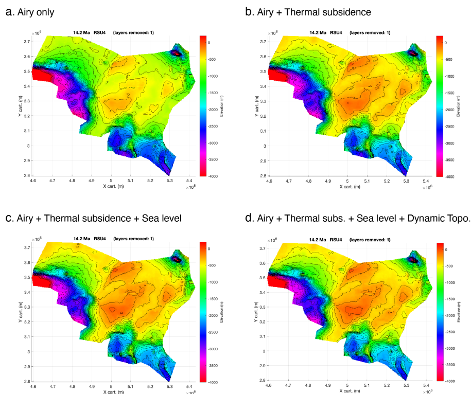
Figure 10. Backtracked Mid-Miocene bathymetries at about 14 Ma: a. corrected only for Airy isostasy; b. same as a. but including thermal subsidence correction with a spatially uniform \beta = 2.1 and the end of rifting sets at 76 Ma; c. same as b. but including eustatic sea level correction based on Miller et al. (2020) \delta^{18}O -derived reconstruction; d. same as c. but including dynamic topography correction based on Müller et al. (2018a) geodynamical model M1 (following Hochmuth et al., 2020). Colorscale is the same as in Fig. 9. For all parameters used in those example see Table 1.
