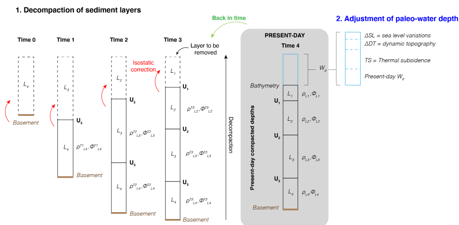
Figure 2. Backstripping/Backtracking procedure: sediment layers L are separated by well-defined seismic or lithological unconformities U . All the sediment layers have different lithological properties defined by their porosity \phi and density \rho . Those two properties changes during the decompaction process, departing from present-day depth of sediment layers, as buried sediments are unloaded from the upper sediment layers (isostatic correction). At this point, the procedure differs: if the aim is backstripping, then the depth of the sediment layers at each time step is adjusted with prescribed time-history of water depth changes (Eq. 1), if the aim is backtracking, the water depth at each time step is calculated using time-varying thermal subsidence model (Eq. 3). PALEOSTRIP computes backtracking.
