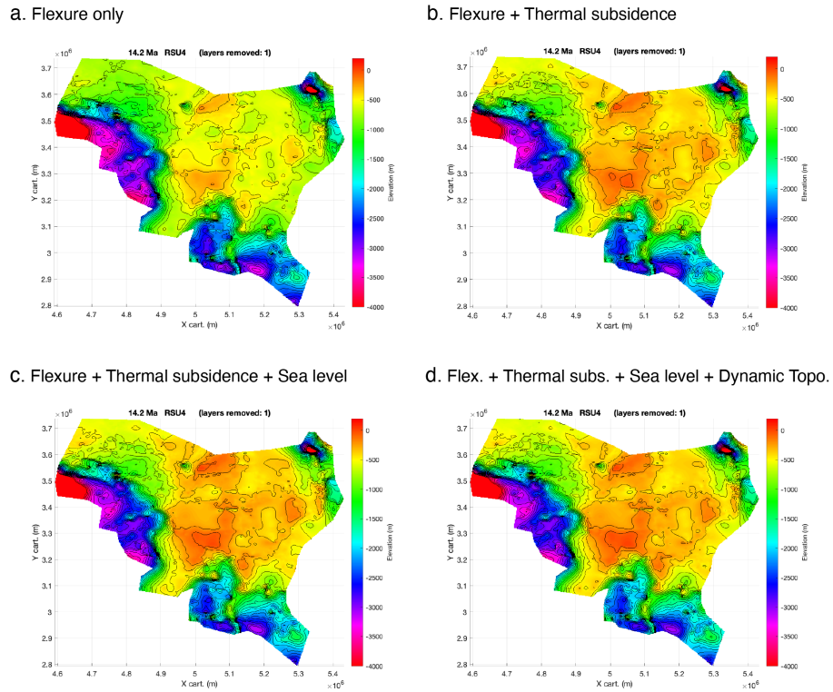
Figure 11. Backtracked Mid-Miocene bathymetries at about 14 Ma. Same as Fig. 10 but using flexural isostasy with spatially variable lithospheric effective elastic thickness from Chen et al. (2018). Layout is from PALEOSTRIP plotting GUI and the colorscale is the default colorscale impemented within PALEOSTRIP and has been saturated below -4000 meters and above 200 meters for the need of this figure. The island located on the uppermost right corner is the only location with elevation above sea level. For all parameters used in those example see Table 1 in Appendix A.
