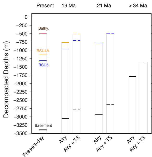
Figure 8. Backtracking steps for Western Ross Sea DSDP 273270 well site. For present-day: present-day depths of basement (black), Ross Sea unconformity 5 (blue), Ross Sea Unconformity 4A (orange) and bathymetry (brown); at time of RSU4A (19 Ma), at time of RSU5 (21 Ma) and at time before glacial sediment deposition (> 34 Ma). For each time step, two backtracking are shown, one accounting for Airy isostatic correction only, and one accounting for Airy isostatic correction and thermal subsidence (dashed). Table 1 in Appendix A.
