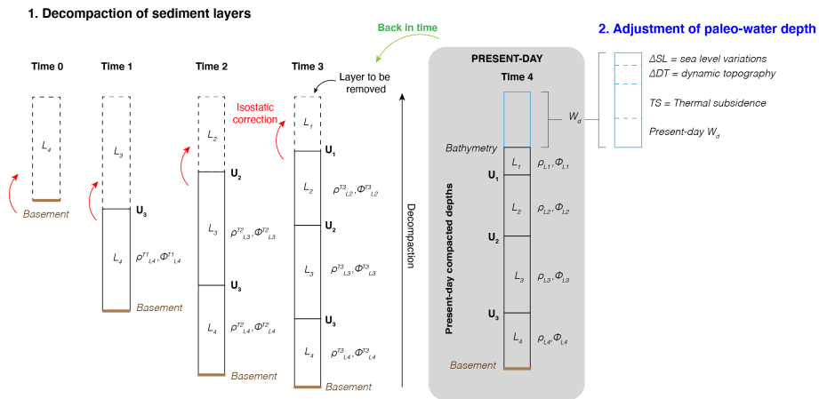
Figure 2. Backstripping /Backtracking procedure: sediment layers L are separated by well-defined seismic or lithological unconformities U . All the sediment layers have different lithological properties defined by their porosity \phi and density \rho . Those two properties changes during the decompaction process, departing from present-day depth of sediment layers, as buried sediments are unloaded from the upper sediment layers (isostatic correction). At this point, the procedure differs: if the aim is backstripping, then the depth of the sediment layers at each time step is adjusted with prescribed time-history of water depth changes (Eq. 1), if the aim is backtracking, The water depth at each time step is calculated using time-varying thermal subsidence model (Eq. 3). PALEOSTRIP computes backtracking.
