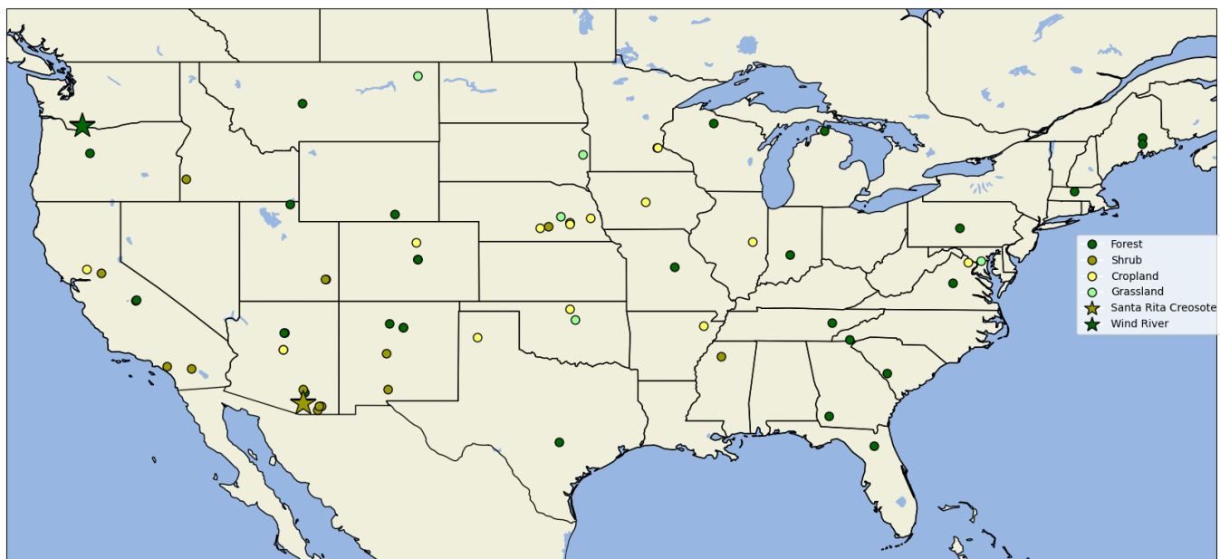
Figure 4. Map showing the location of CRNS sites from the COSMOS network across CONUS. The colours are representative of the land cover types obtained from the ESA CCI global database and the stars highlight the location of the two sites processed above (i.e., Santa Rita Creosote and Wind River).
