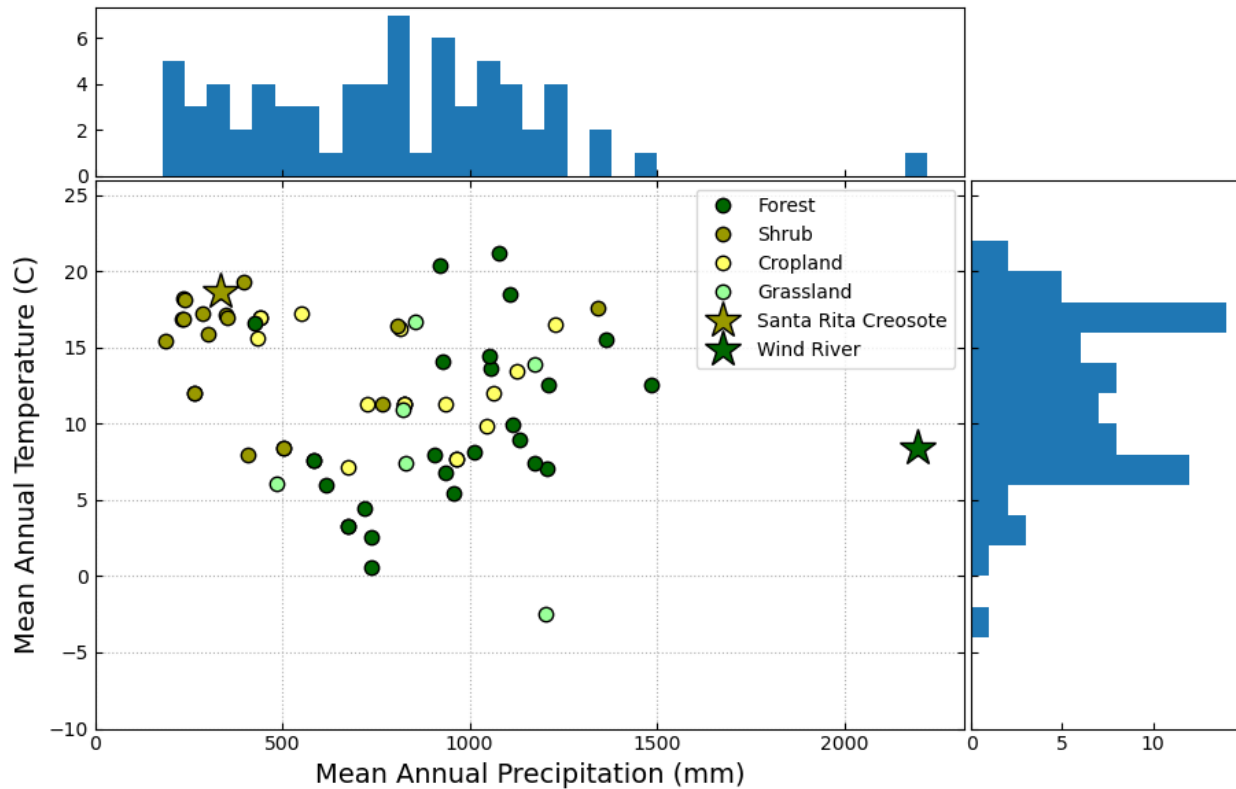
Figure 5. Scatter-histogram showing the Continental USA CRNS sites and some of their climatological characteristics. The units for the histograms are number of sites for each bin. The colours represent land use types which has been identified from ESA CCI Land Use global data set. The stars highlight the location of the two sites processed above (i.e., Santa Rita Creosote and Wind River).
