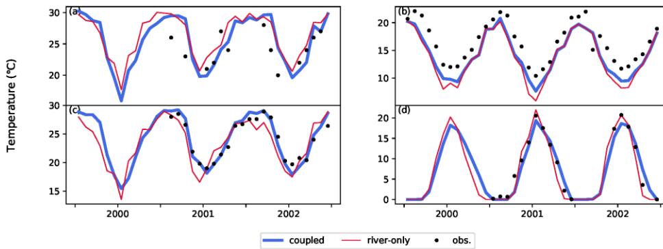
Figure 7: Timeseries of monthly mean values of river temperature (°C). Black dots show the observed values, and blue (red) line shows values simulated-calculated by the “coupled” (“river-only”) modelsimulation . (a) 00MS13SM2000 station in Rio Santa Maria, (b) Hamilton traffic bridge station in the Waikato River, (c) Puerto Libertad station in the Parana River, and (d) Neva River station in the Neva River. Station codes in GEMS are BRA01900, NZL00013, ARG00001, and RUS00014, respectively.
