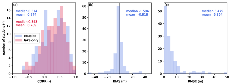
560 Figure 8: Comparison between reproducibility indices of lake surface elevation. Bars are the histogram of each index, and written values show the associated median and mean values. Blue (red) bars and writing show the results of the “coupled” (“lake-only”) simulation. (a) CORR, (b) BIAS (m), and (c) RMSD (m).
