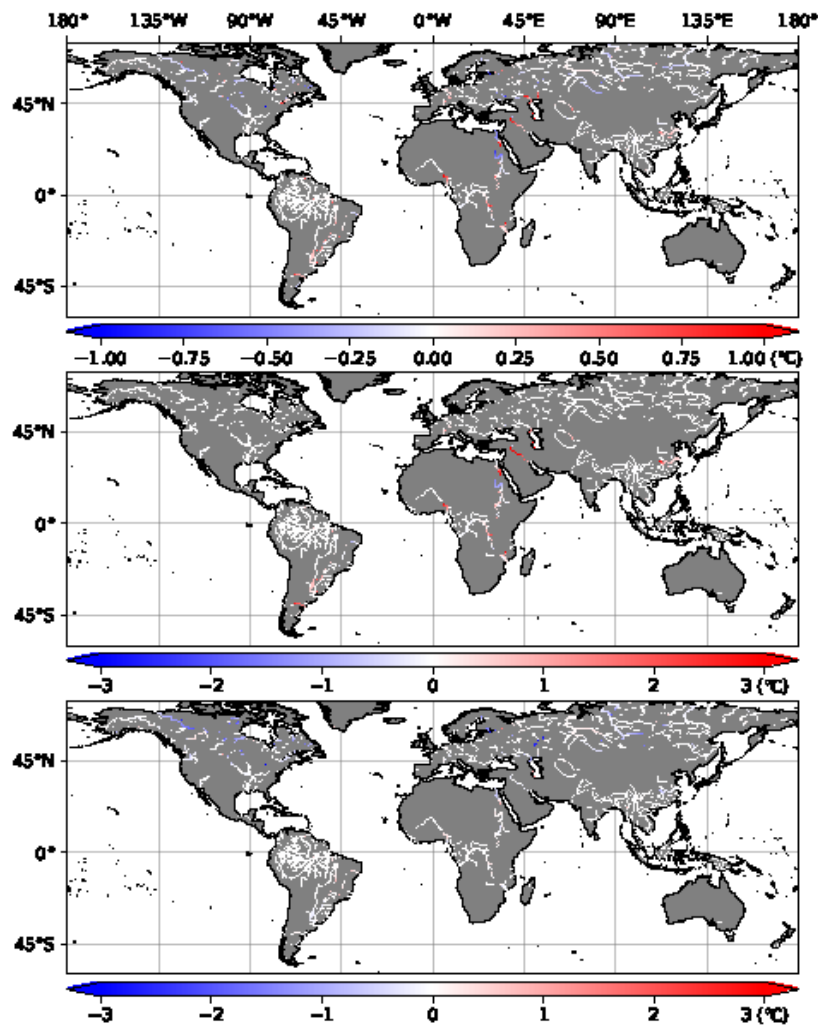
645 Figure 13: Global distribution of the effect of introducing lakes on river water temperature, calculated by subtracting the simulated value of the “river-only” experiment that does not consider lakes from the “coupled” experiment that does (°C). Red color indicates that lakes cause an increase in river water temperature. (a) Annual mean of climatological monthly temperature, (b) minimum, and (c) maximum.
