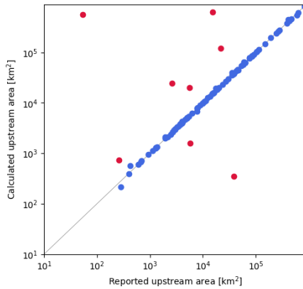
385 Figure 3: Comparison between calculated upstream area (km 2 ) in the river–lake network developed in this study (vertical) and reported values registered in GRanD (horizontal). Red dots indicate the reservoirs whose areas (km 2 ) differ by more than a factor of 2 or 0.5 as listed in Table 2 Table 2 .
