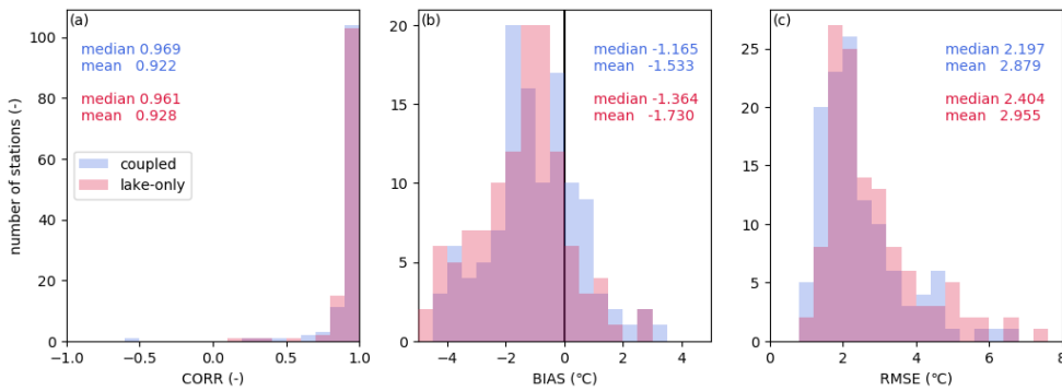
600 Figure 10: Comparison of reproducibility indices for lake surface temperature. Bars indicate the histogram of each index, and characters do the media and mean value of them. Blue (red) bars and characters indicate the result of “coupled” (“lake-only”) simulation. (a) CORR (-), (b) BIAS (°C), and (c) RMSD (°C).
