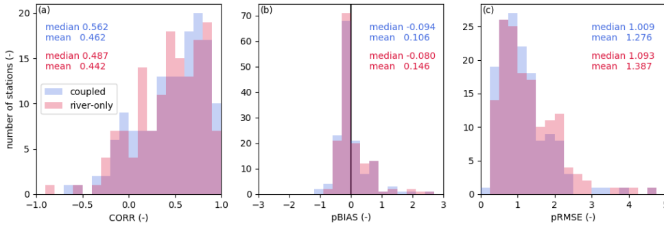
Figure 4: Comparison between reproducibility indices of river discharge: bars are the histograms of each index, and the numbers indicate the associated median and mean values. Blue (red) bars and written values show the results of the “coupled” (“river-only”) simulation. (a) CORR, (b) pBIAS, and (c) pRMSE.
