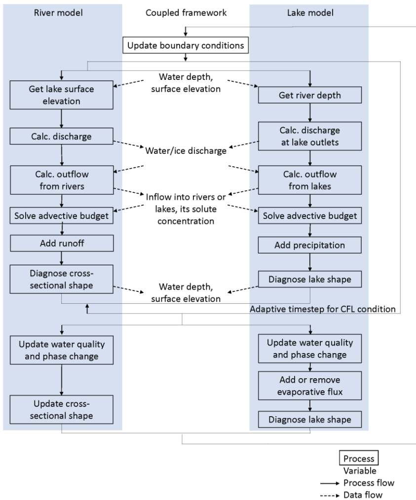
355 Figure 2: Flowchart of the calculation of T-ChoirTCHOIR. The solid (dashed) arrows indicate the order of the calculations (data exchange). The arrow branches indicate that each process can be computed in parallel, but the data exchange takes place at the same time.
