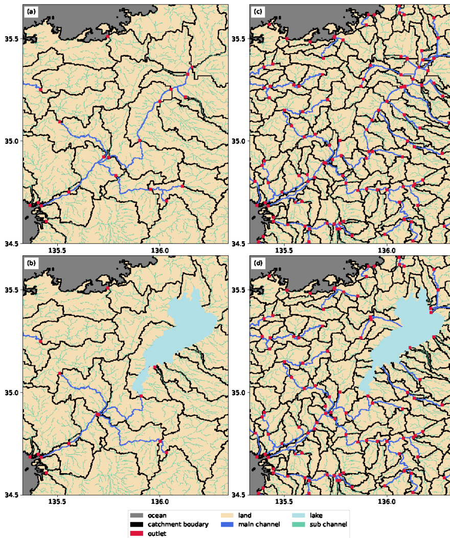
Figure 1: Example of upscaled river-lake network dataset. Figures show results under four different configurations for Lake Biwa and Yodo River basin in Japan, (a) 15' without lakes, (b) 15' with lakes, (c) 6' without lakes, and (d) 6' with lakes.
