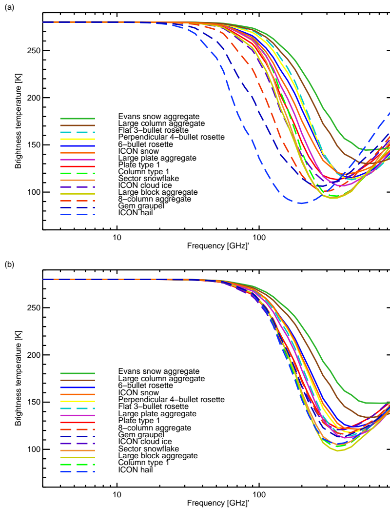
Figure 12. Brightness temperatures from a standard snow or ice cloud; details as Fig. 9a but exploring different PSDs: (a) Heysmsfield et al. (2013, H13); (b) McFarquhar and Heysmsfield (1997, MH97).
