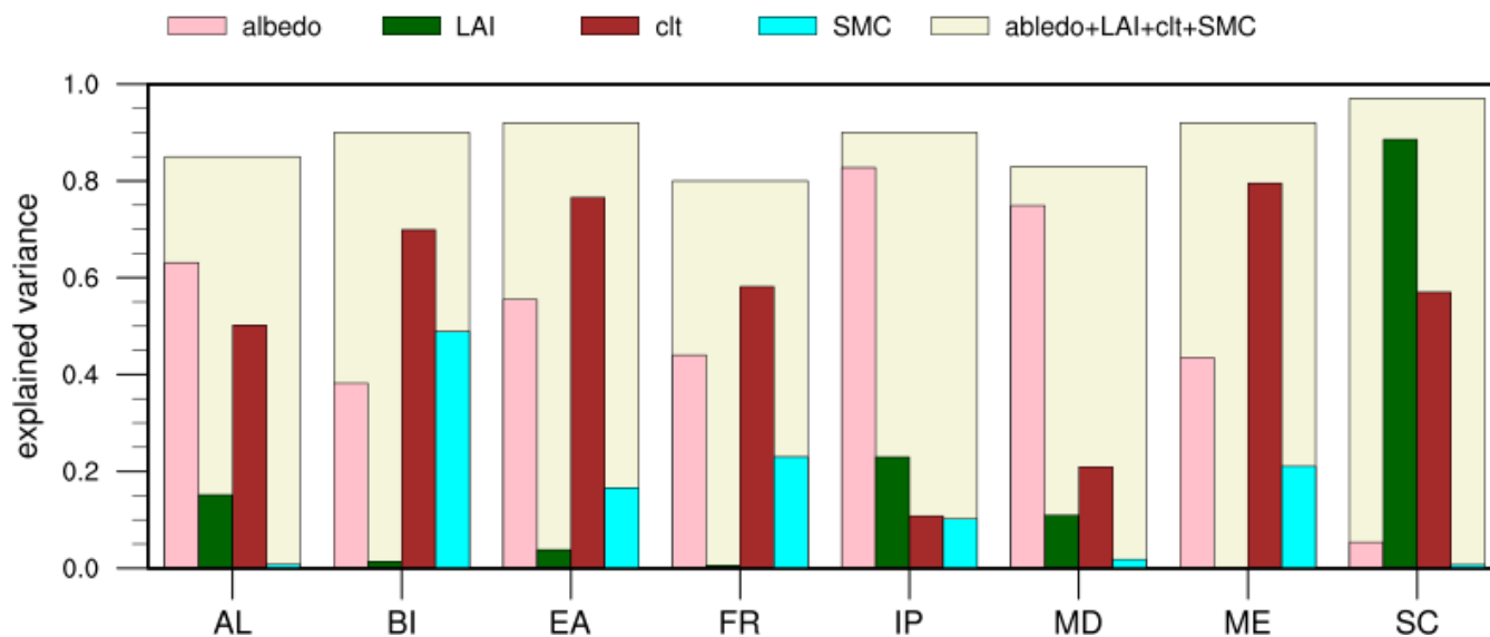
750 Figure 10: The fraction of inter-model variance in AAST response (FOREST minus GRASS) explained by mean summer changes in albedo, leaf area index (LAI), cloud fraction (clt), soil moisture content (SMC) or all combined (albedo+LAI+clt+SMC). Bars represent the coefficient of determination ( R^2 ) values derived from linear regression analysis applied over each sub-region. Alps (AL), British Isles (BI), Eastern Europe (EA), France (FR), Iberian Peninsula (IP), Mediterranean (MD), Mid-Europe (ME), Scandinavia (SC).
