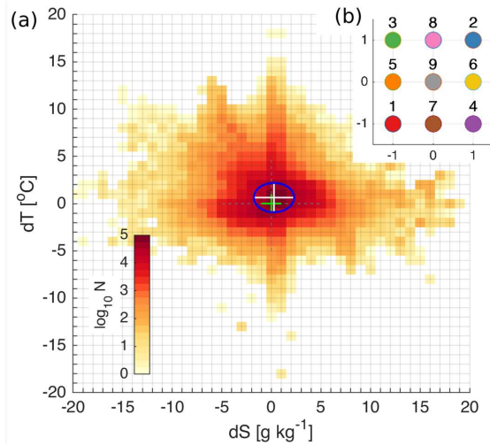
150 Figure 2. Logarithmic distribution of the number of salinity and temperature error pairs (model minus observation) in the 2-dimensional error space (a). Error bins have a resolution of 1 °C for temperature and 1 g kg -1 for salinity. The bias is shown with the center of the white cross and the standard deviations with the major semi-axes of the blue ellipse. The green cross shows the center of the coordinate axes. Coordinates of initial centroids of K-means in the normalized 2-dimensional error space (b).
