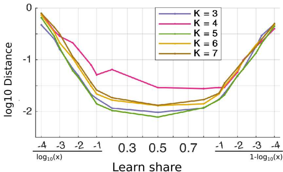
Figure 8. The average normalized distance of shifts of predicting centroids relative to learned centroids as function of the share of the learning dataset. Averaging has been done from 30 trials. Different lines correspond to different numbers of initial clusters, K=3-7 . The share of the learning dataset in the ranges of 10^{-4} -0.1 and 0.9-0.9999 are shown in logarithmic scale.
