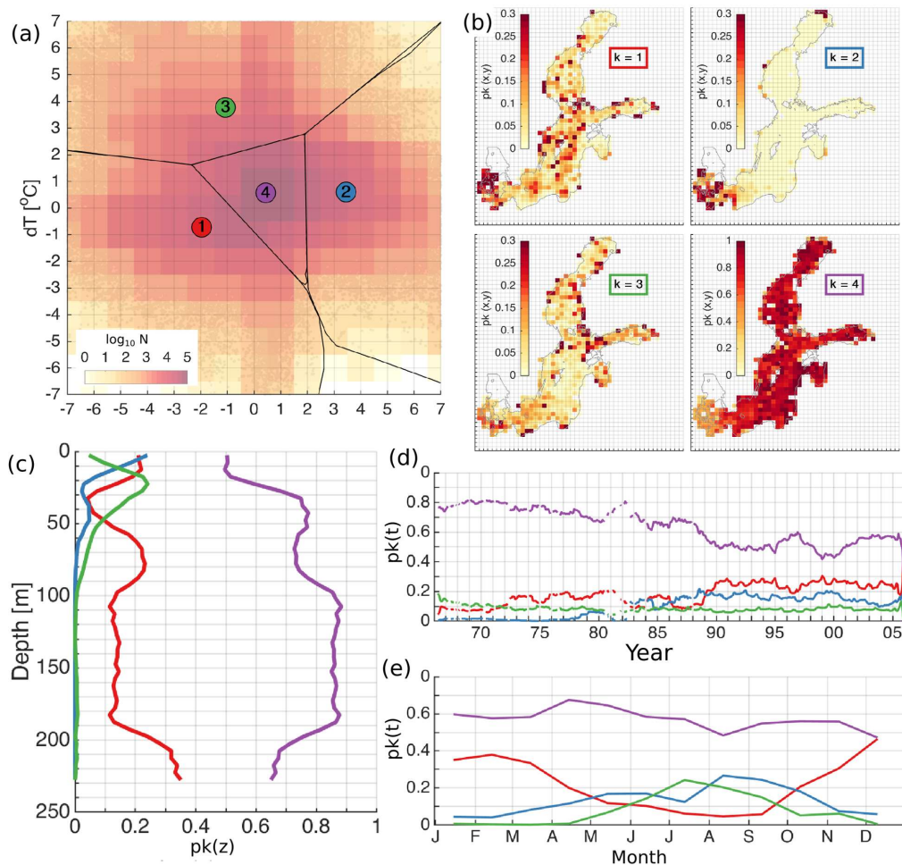
225 Figure 5. The distribution of the error clusters for K=4 (a). The colormap shows the logarithmic distribution of the number of salinity and temperature error pairs (model minus observation) in the 2-dimensional error space (a). Error bins have a resolution of 1\text{ }^{\circ}\text{C} for temperature and 1\text{ g kg}^{-1} for salinity (a). The spatial (b), vertical (c), temporal (d) and seasonal (e) distribution of the share of error points belonging to the four different clusters (b). The share is calculated as explained in Section 2.4. The horizontal bins have a resolution of 25\times 25\text{ km} (b), vertical bins have a resolution of 5\text{ m} (c), temporal and seasonal bins have monthly 230 resolution (d,e). The lines (d) have been smoothed using a running mean with a 12-point window size. Line colors correspond to the colors of the clusters on (a).
