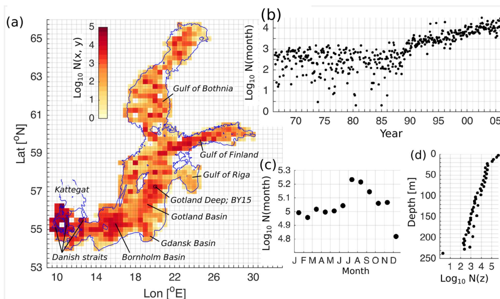
Figure 1: Spatial (a), temporal (b), seasonal (c) and vertical (d) distribution of the number of measurements in the dataset. The horizontal bins have a resolution of 25x25 km (a), temporal and seasonal bins have monthly resolution (b,c), and vertical bins have a resolution of 5 m (d).
