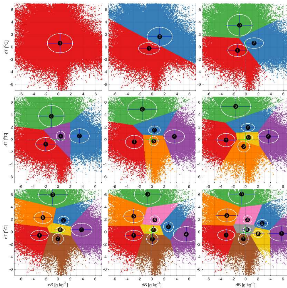
195 Figure 3. The distribution of clusters in the error space for a different number of predefined clusters, K=1-9 . The numbers of the clusters correspond to the numbers of the clusters in Table 1. The biases are marked with the center of the ellipsoid and the standard deviations with the major semi-axes. The error space has been zoomed in for better visualization of the clusters. The full range of error space and distribution of the clusters is shown in Fig. A1 in Appendix A.
