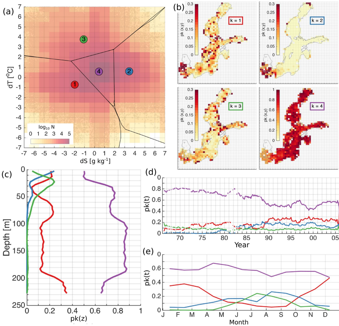
240 Figure 5. The distribution of the error clusters for K=4 (a). The colormap shows the logarithmic distribution of the number of 245 salinity and temperature error pairs (model minus observation) in the 2-dimensional error space (a). Error bins have a resolution of 1^{\circ}\text{C} for temperature and 1\text{ g kg}^{-1} for salinity (a). The spatial (b), vertical (c), temporal (d) and seasonal (e) distribution of the share of error points belonging to the four different clusters (b). The share, p(k) represents the share of the error points belonging to the cluster k , is calculated as explained in Section 2.4. The horizontal bins have a resolution of 25 \times 25\text{ km} (b), vertical bins have a resolution of 5\text{ m} (c), temporal and seasonal bins have monthly resolution (d,e). The lines (d) have been smoothed using a running mean with a 12-point window size. Line colors correspond to the colors of the clusters on (a).
