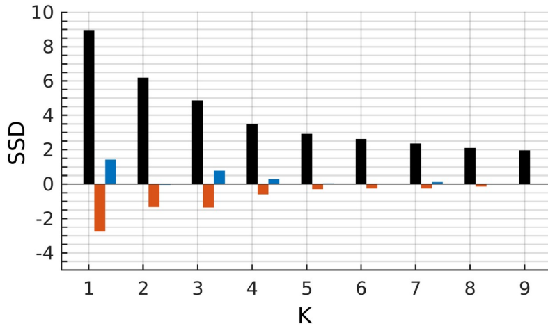
220 Figure 4. Sum of square distances (black bars) between normalized pairs of error points and their designated centroids for different numbers of initial centroids. The first (red bars) and the second (blue bars) order forward differences calculated from the sum of square distances.
