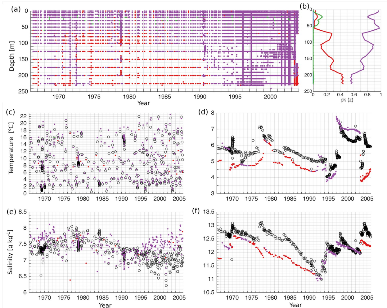
Figure 6 Hovmöller diagram of the distribution of error points of K=4 at the BY15 monitoring station (a). Vertical distribution of the share of error points belonging to the four different clusters (b). The share, p(k) represents the share of the error points belonging to the cluster k , is calculated as explained in Section 2.4. Time series of observed (black circles) and simulated (color dots) temperature (c,d) and salinity (e,f) on the surface (c,e) and bottom (d,f) at the BY15. Colors of dots and lines correspond to the colors of the clusters on Fig. 5a.
