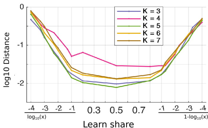
295 Figure 8. The average normalized distance of shifts of predicting centroids relative to learned centroids as function of the share of the learning dataset. Averaging has been done from 30 trials. Different lines correspond to different numbers of initial clusters, K=3-7 . The share of the learning dataset in the ranges of 10^{-4}-0.1 and 0.9-0.9999 are shown in logarithmic scale.
