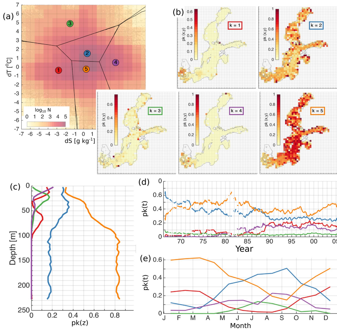
420 Figure B2. The distribution of the error clusters for K=5 (a). The colormap shows logarithmic distribution of the number of salinity and temperature error pairs (model minus observation) in the 2-dimensional error space (a). Error bins have a resolution of 1\text{ }^{\circ}\text{C} for temperature and 1\text{ g kg}^{-1} for salinity (a). The spatial (b), vertical (c), temporal (d) and seasonal (e) distribution of the 425 share of error points belonging to the four different clusters (b). The share, p(k) represents the share of the error points belonging to the cluster k , is calculated as explained in Section 2.4. The horizontal bins have a resolution of 25\times 25\text{ km} (b), vertical bins have a resolution of 5\text{ m} (c), temporal and seasonal bins have monthly resolution (d,e). The lines (d) have been smoothed using a running mean with a 12-point window size. Line colors correspond to the colors of the clusters on (a).
