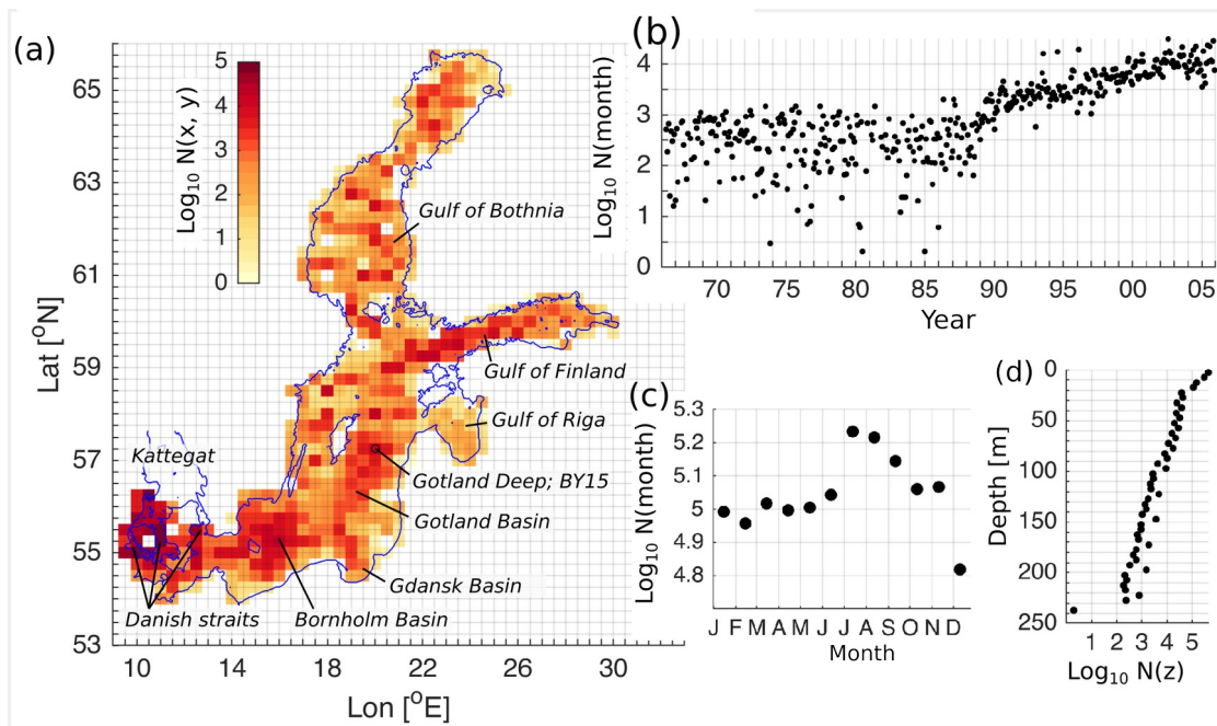
120 Figure 1: Spatial (a), temporal (b), seasonal (c) and vertical (d) distribution of the number of measurements in the dataset. The horizontal bins have a resolution of 25x25 km (a), temporal and seasonal bins have monthly resolution (b,c), and vertical bins have a resolution of 5 m (d).
