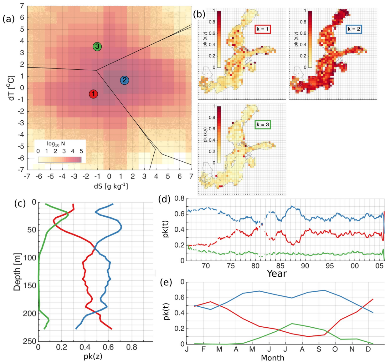
410 Figure B1. The distribution of the error clusters for K=3 (a). The colormap shows logarithmic distribution of the number of 415 salinity and temperature error pairs (model minus observation) in the 2-dimensional error space (a). Error bins have a resolution of 1^{\circ}\text{C} for temperature and 1\text{ g kg}^{-1} for salinity (a). The spatial (b), vertical (c), temporal (d) and seasonal (e) distribution of the share of error points belonging to the four different clusters (b). The share, p(k) represents the share of the error points belonging to the cluster k , is calculated as explained in Section 2.4. The horizontal bins have a resolution of 25 \times 25\text{ km} (b), vertical bins have a resolution of 5\text{ m} (c), temporal and seasonal bins have monthly resolution (d,e). The lines (d) have been smoothed using a running mean with a 12-point window size. Line colors correspond to the colors of the clusters on (a).
