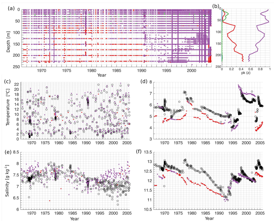
Figure 6 Hovmöller diagram of the distribution of error points of K=4 at the BY15 monitoring station (a). Vertical distribution of the share of error points belonging to the four different clusters (b). The share, p(k) represents the share of the error points belonging to the cluster k , is calculated as explained in Section 2.4. Time series of observed (black circles) and simulated (color dots) temperature (c,d) and salinity (e,f) on the surface (c,e) and bottom (d,f) at the BY15. Colors of dots and lines correspond to the colors of the clusters on Fig. 5a.
