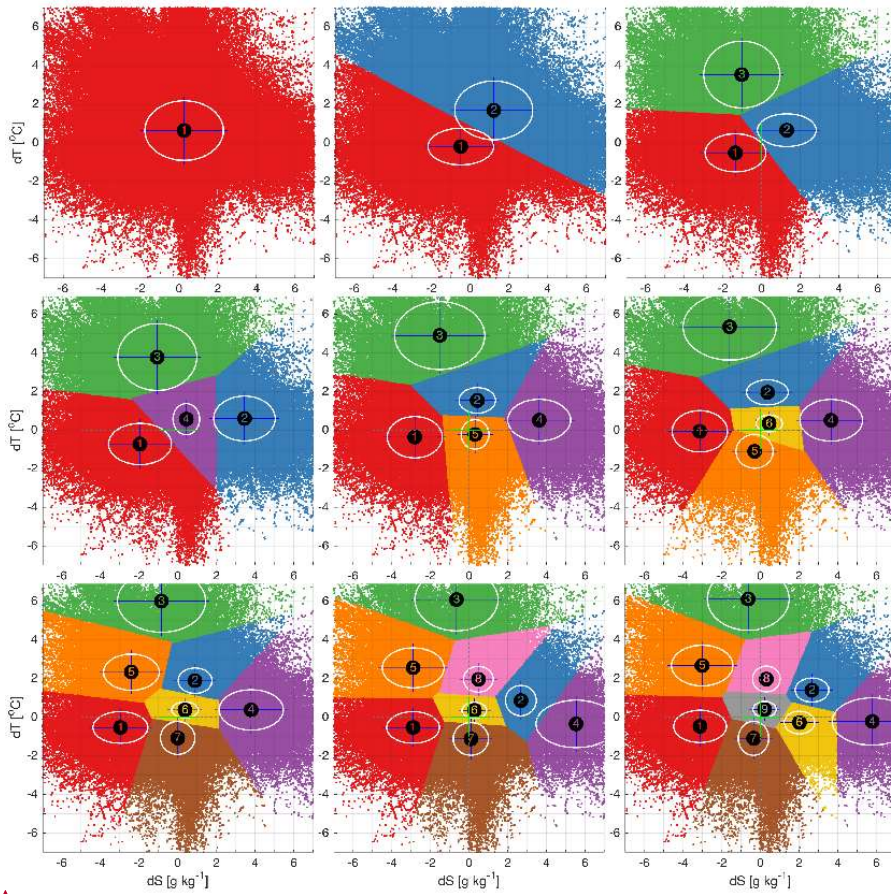
Figure 3. The distribution of clusters in the error space for a different number of predefined clusters, K=1-9 . The numbers of the clusters correspond to the numbers of the clusters in Table 1. The biases are marked with the center of the ellipsoid and the standard deviations with the major semi-axes. The error space has been zoomed in for better visualization of the clusters. The full range of error space and distribution of the clusters is shown in Fig. A1 in Appendix A.
