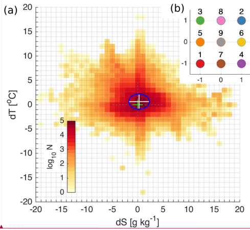
Figure 2. Logarithmic distribution of the number of salinity and temperature error pairs (model minus observation) in the 2-dimensional error space (a). Error bins have a resolution of 1^{\circ}\text{C} for temperature and 1 \text{ g kg}^{-1} for salinity. The bias is shown with the center of the white cross and the standard deviations with the major semi-axes of the blue ellipse. The green cross shows the center of the coordinate axes. Coordinates of initial centroids of K-means in the normalized 2-dimensional error space (b).
