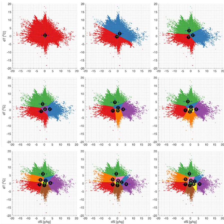
415 Figure A1. The distribution of clusters in the error space for a different number of predefined clusters, K=1-9 . The numbers of the clusters correspond to the numbers of the clusters in Table 1. The locations of the centroids are marked with cluster numbers and the standard deviations with the whiskers.
