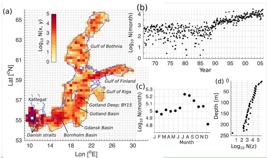
125 Figure 1: Spatial (a), temporal (b), seasonal (c) and vertical (d) distribution of the number of measurements in the dataset. The horizontal bins have a resolution of 25x25 km (a), temporal and seasonal bins have monthly resolution (b,c), and vertical bins have a resolution of 5 m (d).
