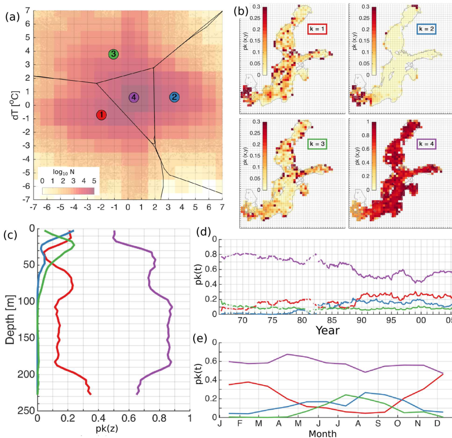
265 Figure 5. The distribution of the error clusters for K=4 (a). The colormap shows the logarithmic distribution of the number of salinity and temperature error pairs (model minus observation) in the 2-dimensional error space (a). Error bins have a resolution of 1 °C for temperature and 1 g kg -1 for salinity (a). The spatial (b), vertical (c), temporal (d) and seasonal (e) distribution of the share of error points belonging to the four different clusters (b). The share, p(k) represents the share of the error points belonging 270 to the cluster k , is calculated as explained in Section 2.4. The horizontal bins have a resolution of 25x25 km (b), vertical bins have a resolution of 5 m (c), temporal and seasonal bins have monthly resolution (d,e). The lines (d) have been smoothed using a running mean with a 12-point window size. Line colors correspond to the colors of the clusters on (a).
