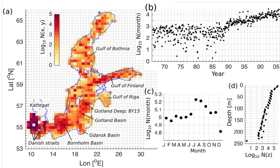
140 Figure 1: Spatial (a), temporal (b), seasonal (c) and vertical (d) distribution of the number of measurements in the dataset. The horizontal bins have a resolution of 25x25 km (a), temporal and seasonal bins have monthly resolution (b,c), and vertical bins have a resolution of 5 m (d).
