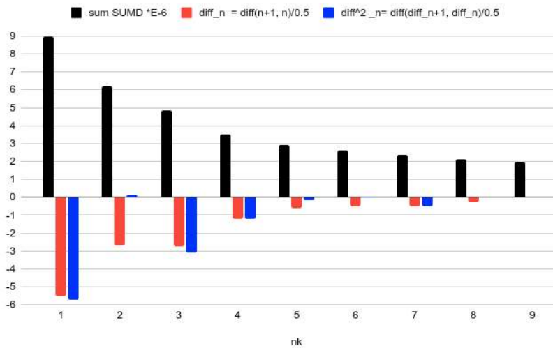
Figure 4. Sum of square distances (black bars) between normalized pairs of error points and their designated centroids for different numbers of initial centroids. The first (red bars) and the second (blue bars) order forward differences calculated from the sum of square distances.
