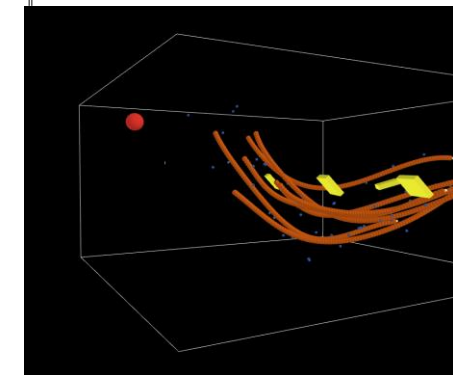
Figure 2. Structural form traces (orange point streams) estimated from dip data (yellow cuboids) using spatial agents. Red sphere is an interrogator agent. Blue dots are simulated Bézier control points with added random noise. See Appendix A for details.¶
