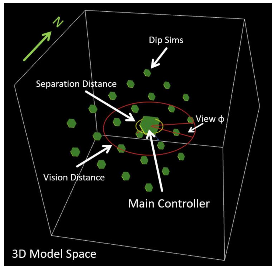
Figure 7. Components of the spatial agent-based model (SABM).
