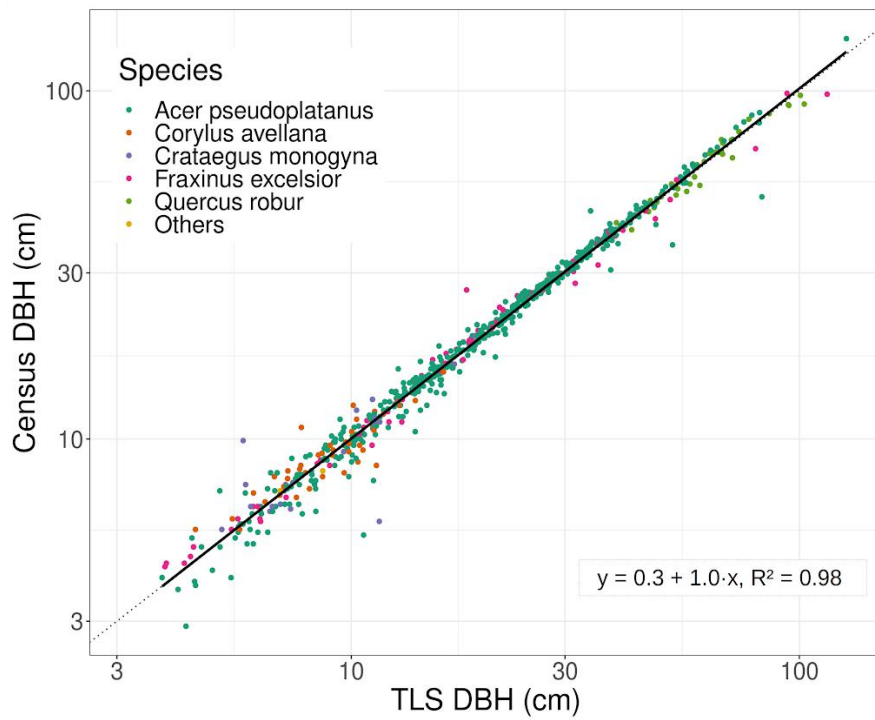
Figure S1: Comparison between field inventoried and TLS-derived DBH.
