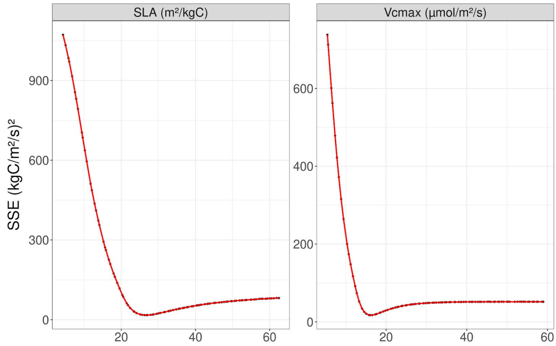
Figure S3: Univariate model sensitivity to the calibrated parameters (SLA, left and Vcmax, right), illustrated for the IC-TLS configuration around the posterior median (SLA = 26.9 m 2 /kgC, Vcmax = 16.7 µmol m -2 s -1 ). The y-axis is the sum of squared estimates of errors (SSE).
