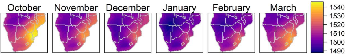
395 Figure 2: Mean monthly geopotential height at 850 hPa in ERA5 for the period 1986-2005.
