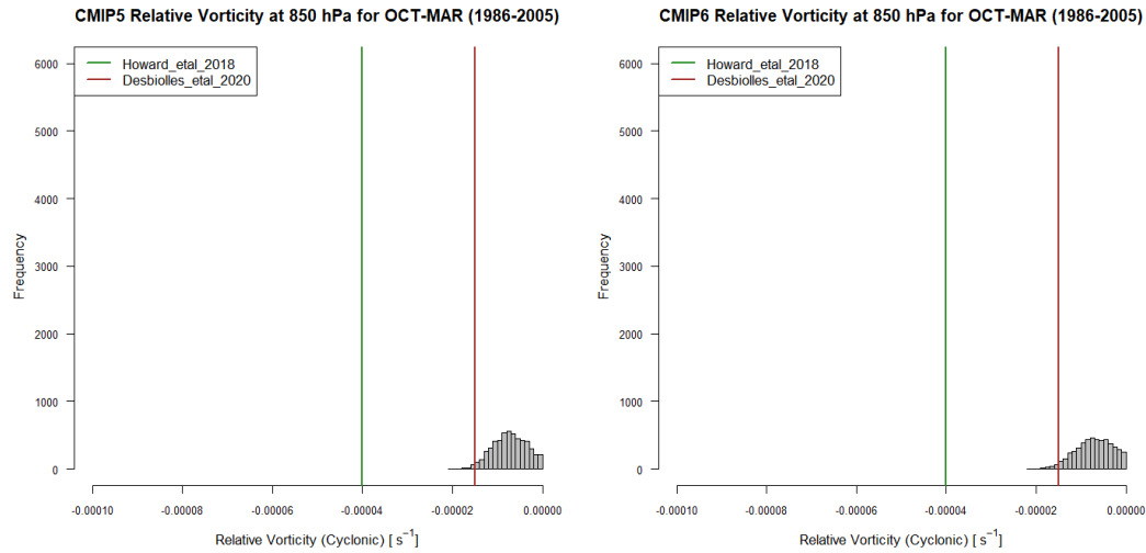
Figure 8: Histogram of relative vorticity for months Oct-Mar during 1986-2005 at 850 hPa for CORDEX-Africa at 0.22° (upper left), for CORDEX-Africa 0.44° (upper right), for CMIP5 (lower left), and for CMIP6 (lower right). Pixels used are enclosed by the region from 14 °E to 25 °E and from 11 °S to 19 °S. For all histograms mean monthly u and v values are used.
