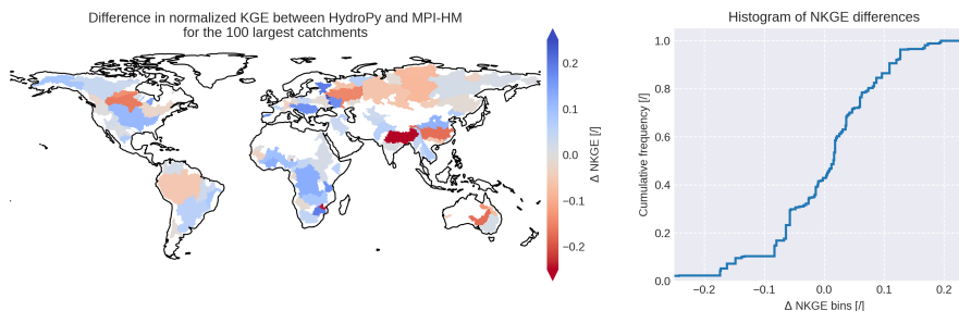
Figure 12. Spatial distribution (left) and cumulative histogram (right) of NKGE differences for river discharge between HydroPy and MPI-HM.
