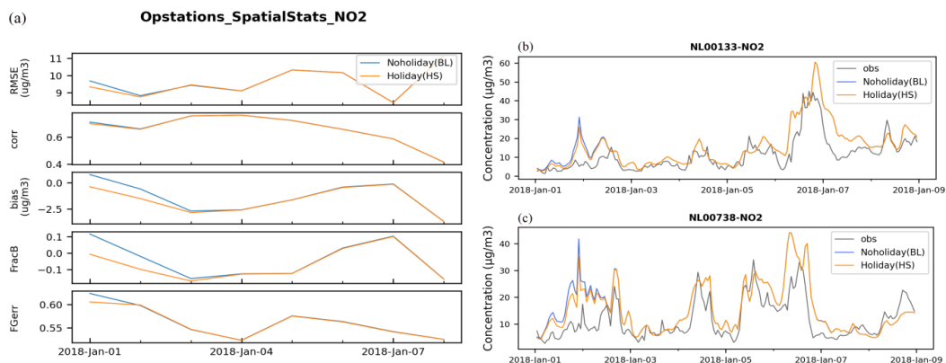
Figure 3. (a): SILAM daily-mean spatial scores for New Year holiday (whole Europe), (b, c): Time series of the modelled and observed concentrations for two stations in the Netherlands.
