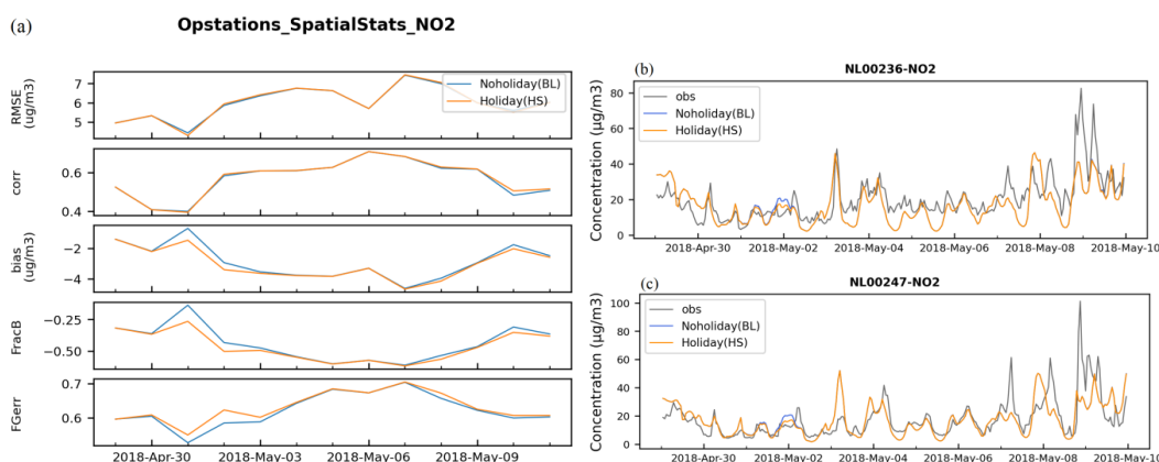
Figure 5. (a): SILAM daily-mean spatial scores for May vacations (whole Europe), (b, c): Time series of the modelled and observed concentrations for two stations in the Netherlands.
