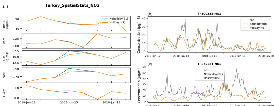
Figure 6. (a) : SILAM daily-mean spatial scores for Ramadan (only stations in Turkey), (b, c) : Time series of the modelled and observed concentrations for two Turkish stations.
