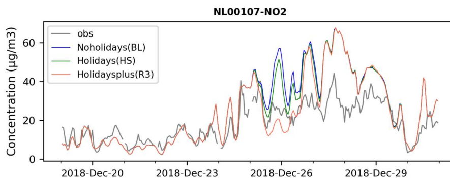
Figure 7. Time series of the modelled (BL and HS runs without and with accounting official holiday, respectively, and Holidaysplus (R3) run with 80% reduction of emission), and observed concentrations for the selected station.
