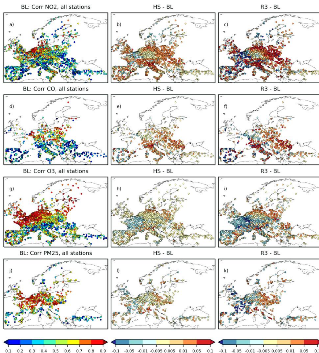
Figure 8. Maps of the temporal correlation coefficient of hourly \text{NO}_2 , \text{CO} , \text{O}_3 , and \text{PM}_{2.5} concentrations for the EEA stations during the Christmas holidays (21-31 December 2018).
