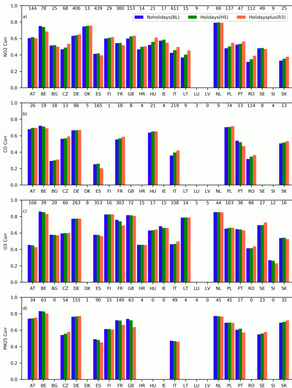
Figure 9. Country-wise median change of temporal correlation coefficient during two weeks of Christmas holidays (21-31 December 2018). The numbers at the top of each panel shows the number of stations that reported data for the period.
