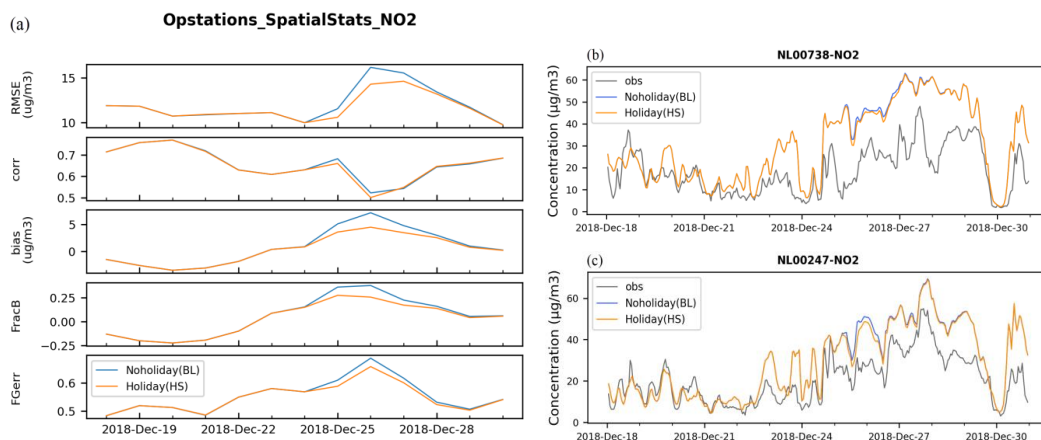
Figure 2. (a): SILAM daily-mean spatial scores for Christmas (whole Europe), (b, c): Time series of the modelled and observed concentrations for two stations in the Netherlands.
