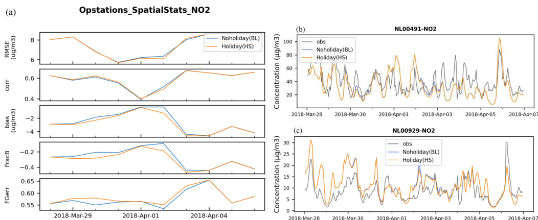
Figure 4. (a): SILAM daily-mean spatial scores for Easter (whole Europe), (b, c): Time series of the modelled and observed concentrations for two stations in the Netherlands.
