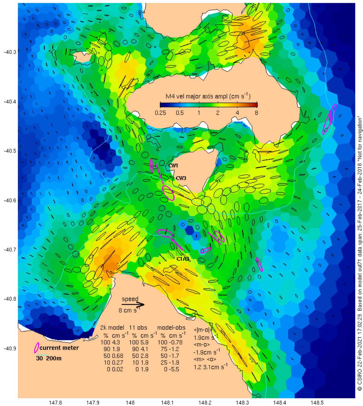
455 Figure 14 Amplitude of the M4 major axis velocity for the Banks Strait region, otherwise like Fig. 5.
