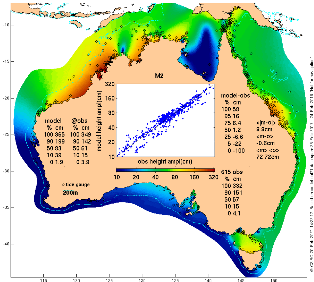
Figure 3 M2 height amplitude as a colour-fill map (the model) and points (observations), and inset as a quantity-quantity plot. Statistics listed are percentiles (“%”) of 1) at left, the model height field at all grid points, 2) the model at observation sites (hereafter m), 3) model error m-o and 4) the observed values o (of which there are 615 within the area shown). At right are 1) \langle |m-o| \rangle , the mean of the absolute value of model error m-o, 2) \langle m-o \rangle , the mean error, and 3) \langle m \rangle and \langle o \rangle which are the means of m and o. A log scale is used, starting at 10cm, so not all points can be shown.
