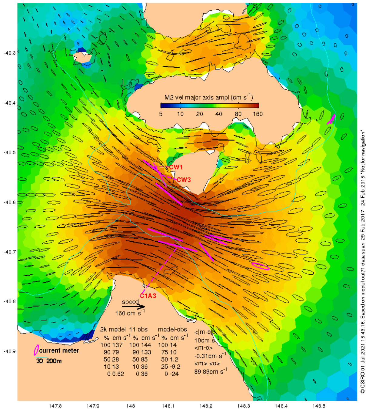
360 Figure 7 Amplitude of the M2 major axis velocity for Banks Strait, otherwise like Fig. 5.
