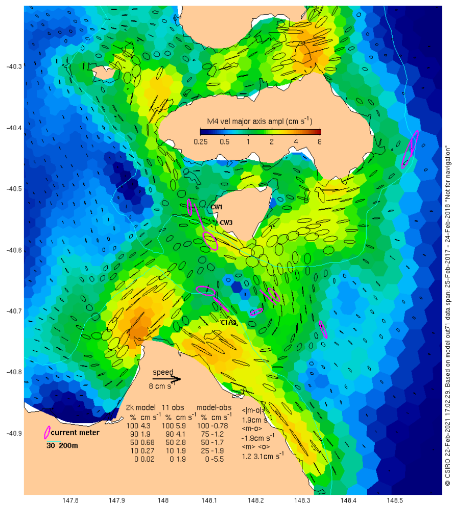
Figure 1413 Amplitude of the M4 major axis velocity for the Banks Strait region, otherwise like Fig. 5.
