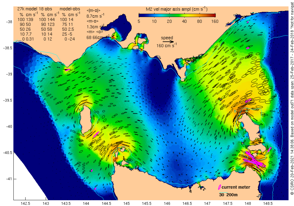
365 Figure 6 Amplitude of the M2 major axis velocity for Bass Strait, otherwise like Fig. 5, except that percentiles of the model at the locations of the observations are not listed.
