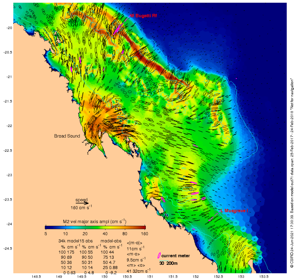
410 Figure 11 Amplitude of the M2 major axis velocity for the Southern Great Barrier Reef region, otherwise like Fig. 5.
