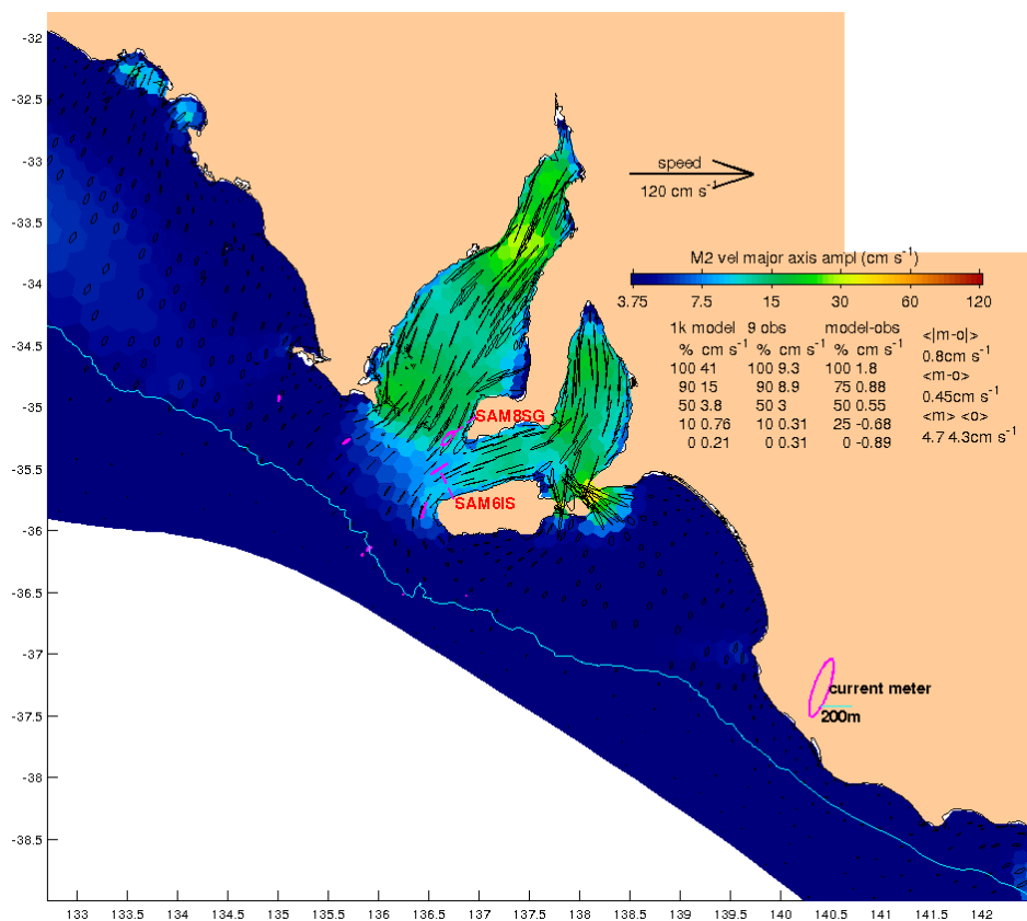
Figure 1342 Amplitude of the M2 major axis velocity for the South Australia region, otherwise like Fig. 5.
