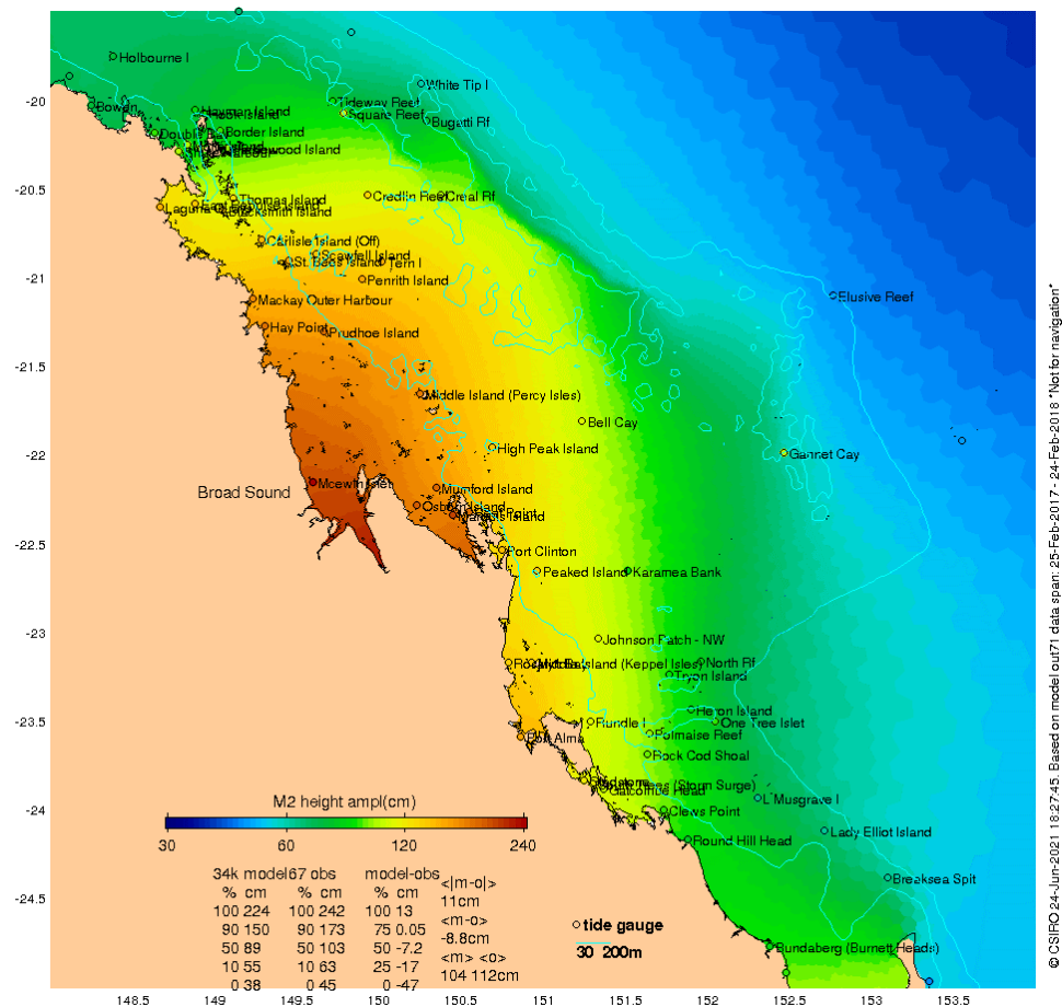
Figure 12 Amplitude of the M2 height for the Southern Great Barrier Reef region, otherwise like Fig. 3.
