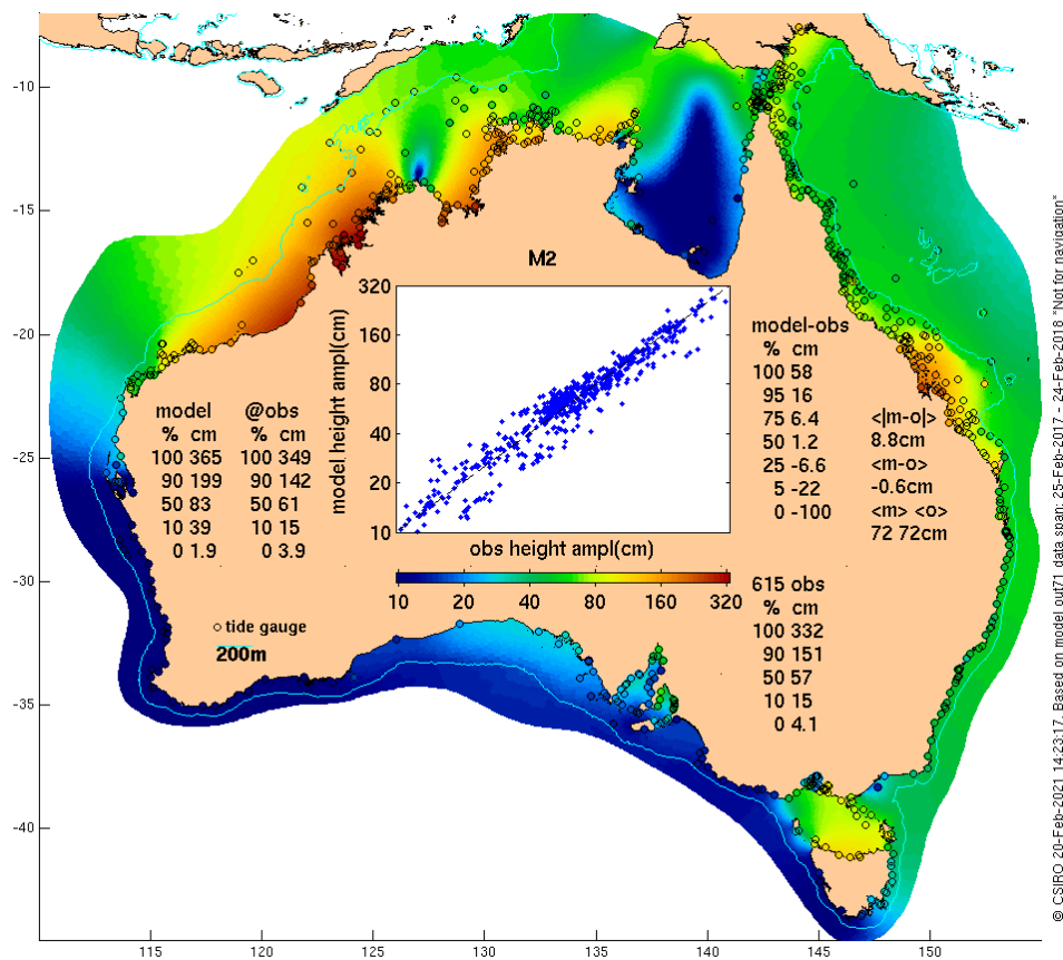
Figure 3 M2 height amplitude as a colour-fill map (the model) and points (observations), and inset as a quantity-quantity plot. Statistics listed are percentiles ('%') of 1) the whole model height field, 2) m=model at validation sites, 3) model error m-o and 4) o=observed values. \langle|m-o|\rangle is the Mean of the Absolute value of m-o. \langle m-o \rangle is the mean error, or bias. \langle m \rangle and \langle o \rangle are the mean modelled and observed amplitudes. A log scale is used, starting at 10cm, so not all points can be shown.
