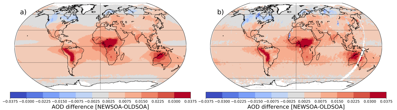
Figure S7: Differences between NEWSOA and OLDSOA as collocated to MODIS (a) and AATSR (b).
