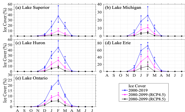
Figure 13. Projected monthly ice cover in the five lakes in the late century (2080-2099) in RCP 4.5 (pink) and RCP 8.5 (black) in comparison to the present-day conditions (2000-2019) (blue). Vertical error bars indicate the range of the three individual GLARM projections.
