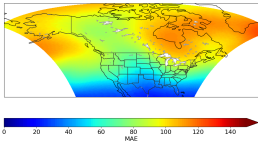
(e) MAE: Regular emulator
