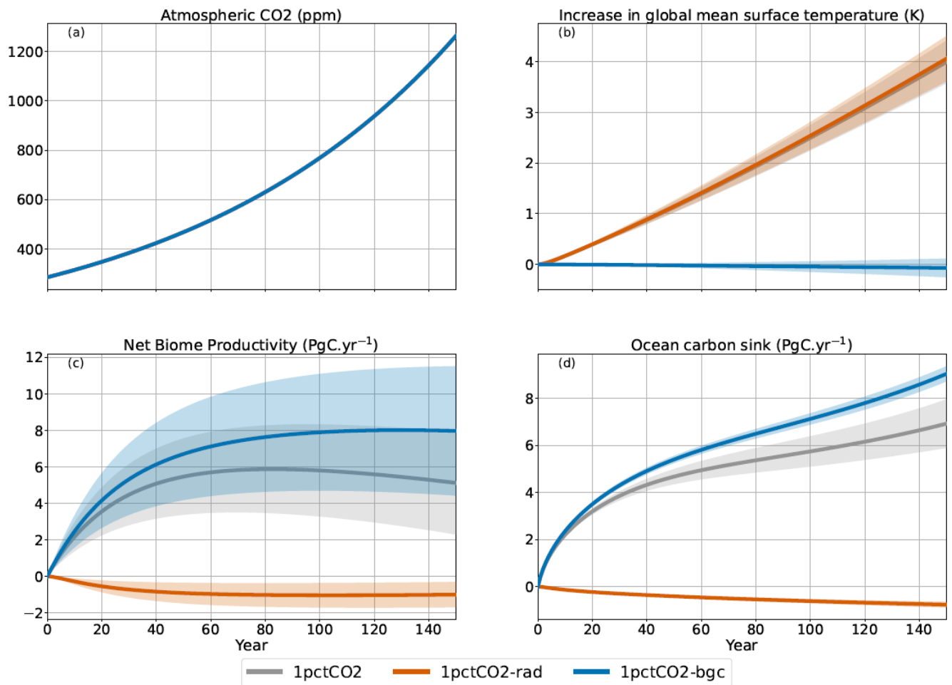
1160 Figure 5: Experiments with 1% increase in the atmospheric CO 2 . The plain lines are the averages, and the shaded areas represent \pm 1 standard deviation ranges.
