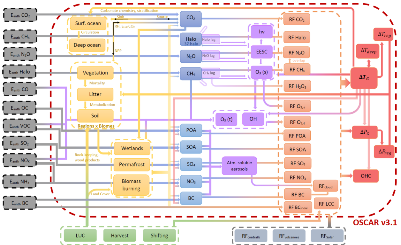
1125 Figure 1: Conceptual figure of OSCAR v3.1. The central box with red dashed lines illustrates the framework of OSCAR v3.1, taking as inputs anthropogenic emissions (dark grey boxes), land use and land cover change (green boxes) and additional radiative forcings (light grey boxes). The components of OSCAR v3.1 are organized in this figure by category: ocean carbon, land carbon and other land processes are in yellow boxes, while atmospheric concentrations are in blue boxes, atmospheric chemistry in purple boxes, radiative forcings in orange boxes and climate system in red boxes. The complete description of OSCAR v2.2 is in (Gasser et al., 2017), while the update to OSCAR v3.1 is described in (Gasser et al., 2020).
