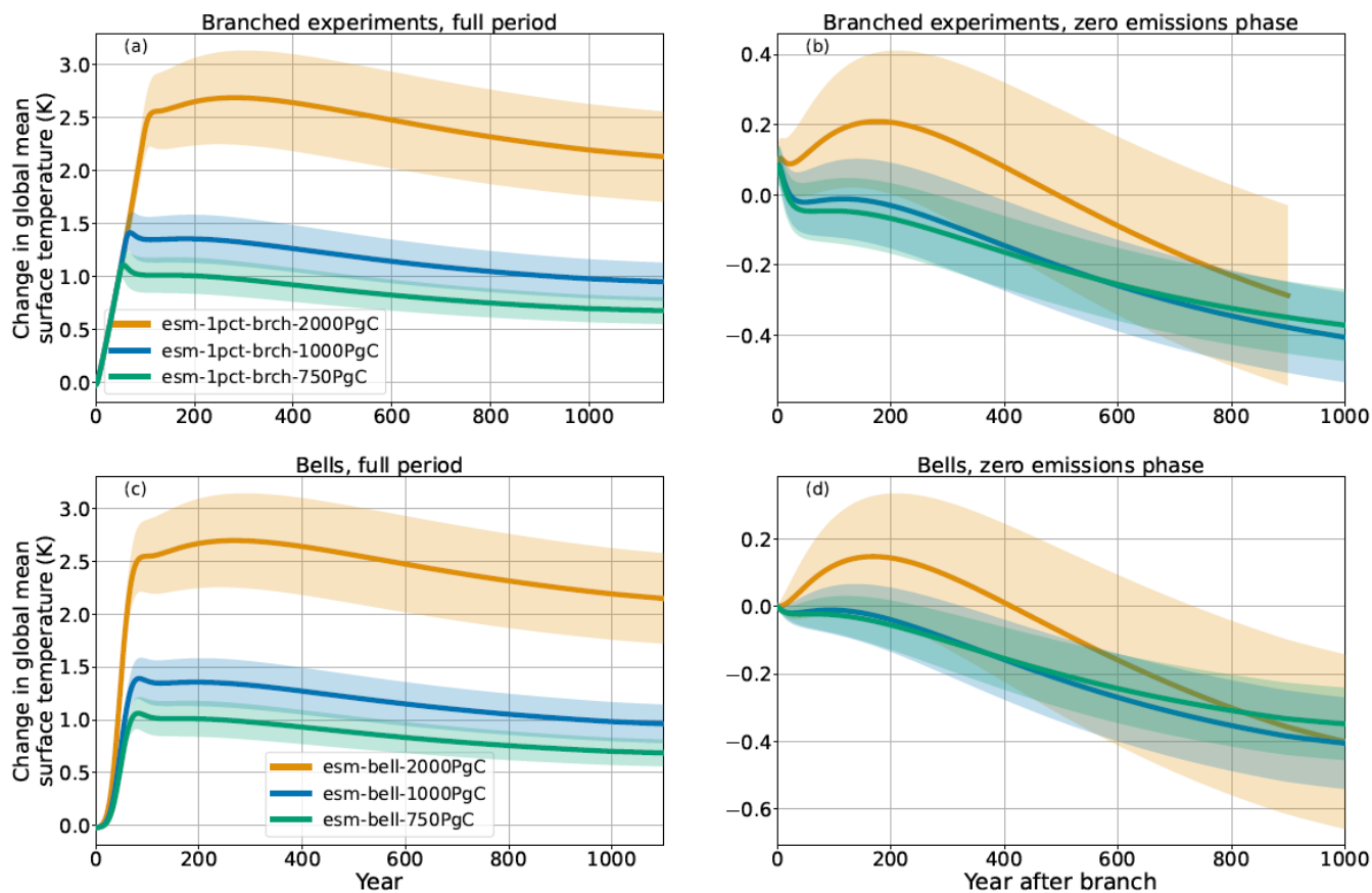
Figure 8: Change in global mean surface temperature for branched experiments (top panels) and bells experiments (bottom panels). The results over the zero-emission phase are shifted along the time axis so that t = 0 corresponds to the time of cessation of emission. The lines are the averages, and the shaded areas represent \pm 1 standard deviation ranges.
