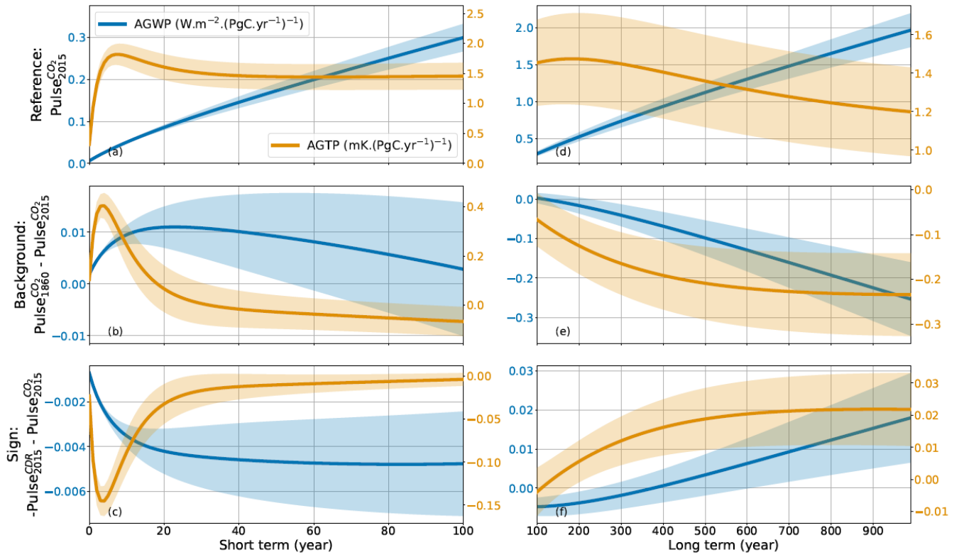
1185 Figure A. 2: AGWP (blue) and AGTP (orange) of CO 2 for 100PgC of CO 2 emissions under actual environmental conditions. The dependency of this reference to a change of background is on the second line. The dependency to the sign of the pulse, emissions or removal, is on the third line. The lines are the averages, and the shaded areas represent \pm 1 standard deviation ranges.
