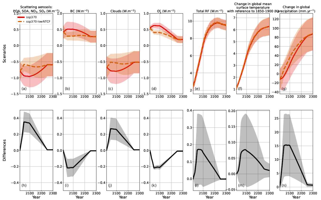
1215 Figure A. 8: Effect of lower NTCF emissions in the SSP3-7.0. Extensions are shown only up to 2300. The lines are the averages, and the shaded areas represent \pm 1 standard deviation ranges.
