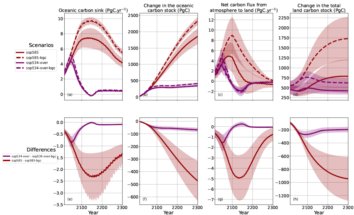
1190 Figure A. 3: Effect of climate change on the carbon cycle in the scenarios ssp534-over and ssp585 . The net flux from atmosphere from land is the sum of the land carbon sink, CO 2 emissions from land-use and land-cover change, and CO 2 and CH 4 emissions from permafrost. The changes in the total land carbon stock include those in the permafrost. Note that the increased uncertainty in the ocean sink before 2250 is an artefact of our exclusion procedure (see text on post-processing) that cannot capture the Monte Carlo members that already started diverging. Extensions are shown only up to 2300. The lines are the averages, and the shaded areas represent \pm 1 standard deviation ranges.
