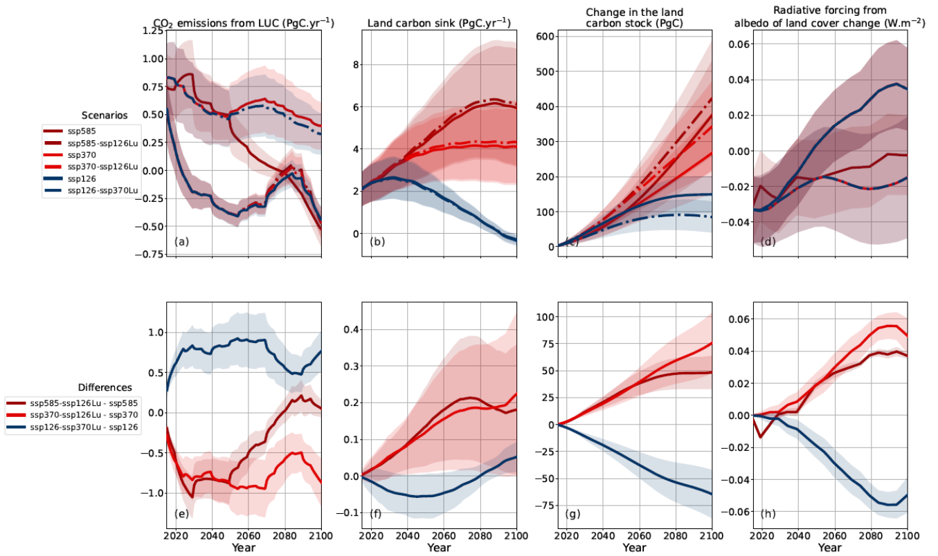
1210 Figure A. 7: Effect of alternative land-use and land-cover change drivers in the scenarios ssp126 , ssp370 and ssp585 . Here, the changes in the land carbon stock does not include the changes in the permafrost. The lines are the averages, and the shaded areas represent \pm 1 standard deviation ranges.
