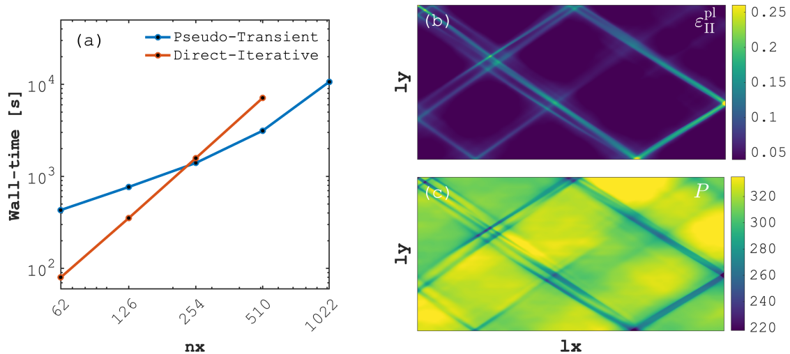
Figure 15. Performance comparison between the pseudo-transient and direct-iterative method resolving 2D shear band formation out of a random noise cohesion field. (a) Wall-time in seconds as function of numerical grid resolution in x -direction ( \sqrt{n_{\text{dof}}} ). Panels (b) and (c) depict total accumulated plastic strain \varepsilon_{II}^{\text{pl}} and pressure [MPa], respectively, from the 1022 \times 1022 resolution 2D PT GPU simulation.
