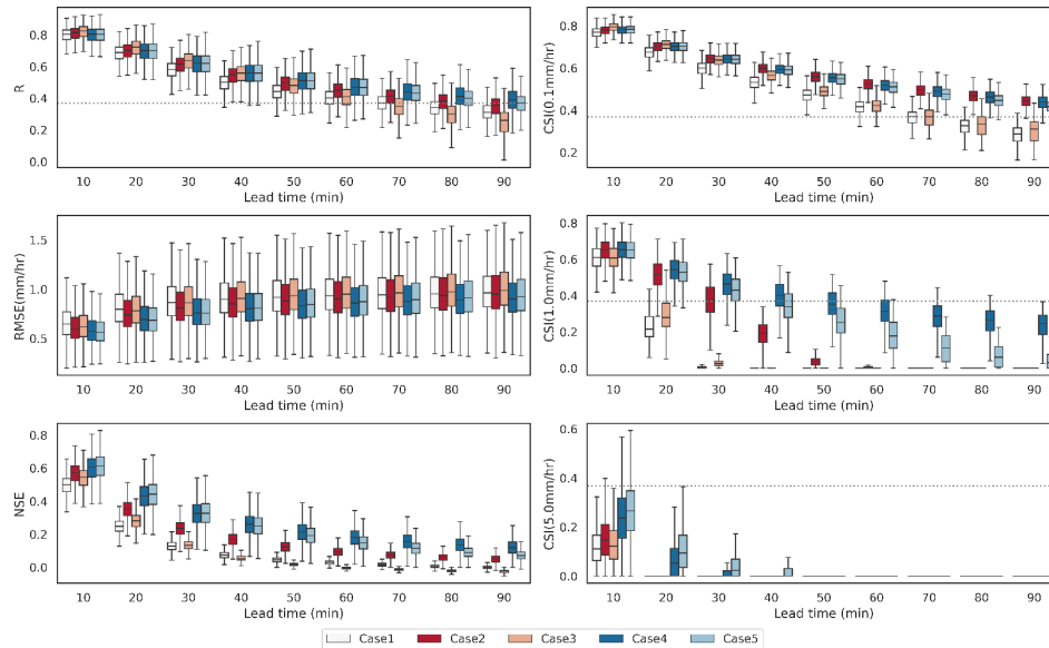
250 Figure 8: Box plot of the verification metrics of model predictions at lead time up to 90 min over all grid cells from the Andong Dam Basin. (a) R, (b) NSE, (c) RMSE, and (d, e, f) CSI at intensity thresholds of 0.1, 1.0, and 5.0 mm h -1 , respectively. Grey dotted line represents the predictability threshold ( 1/e \approx 0.37 ).
