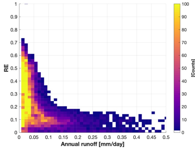
325 Figure 3. Plot of relative norm-2 error (RE) of surrogate models for the validation simulations vs. averaged annual runoff magnitude with all the grid cells from arid region.
