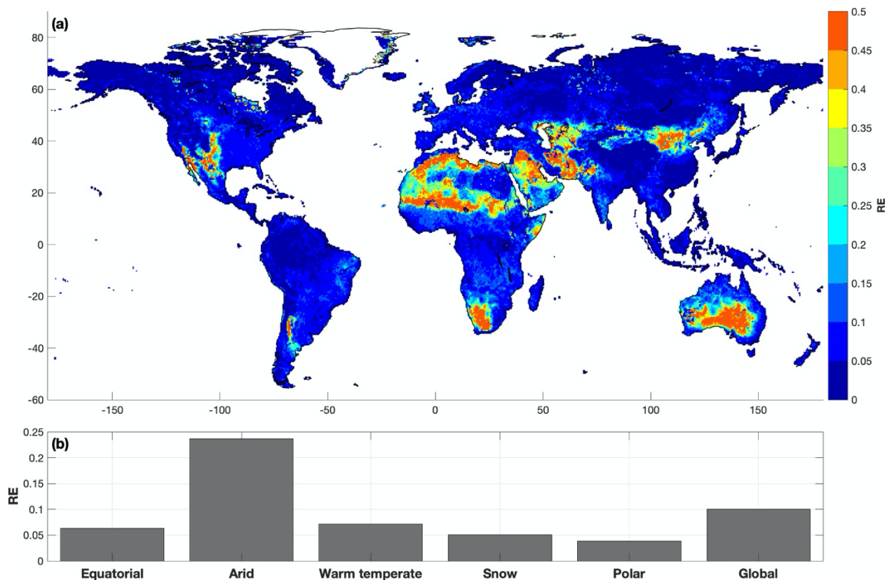
Figure 2. Relative norm-2 error of the surrogate models for the validation simulations. Subplot (a) shows the spatial distribution of the errors, and subplot (b) shows the average errors for the grid cells in each climate defined by Köppen climate classification.
