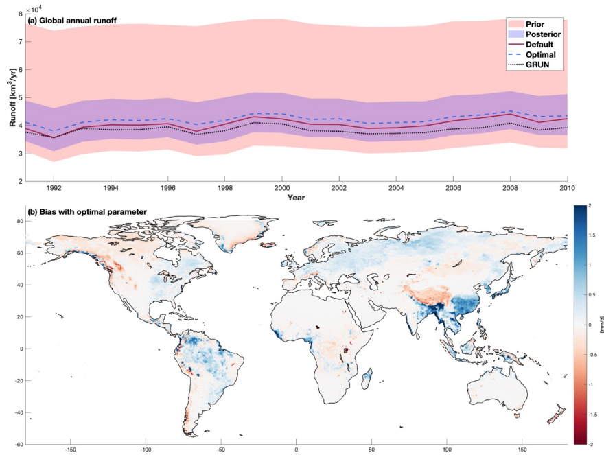
470 Figure 10. (a). Annual global runoff from default ELM simulation, optimal ELM simulation, and GRUN runoff dataset for the simulation period (1991-2010). The red and blue shade areas represent the uncertainties constructed from the simulations with parameter sampled on priors and posteriors, respectively. Subplot (b) shows the absolute difference of annual average runoff between ELM simulation with optimal parameter and GRUN runoff data.
