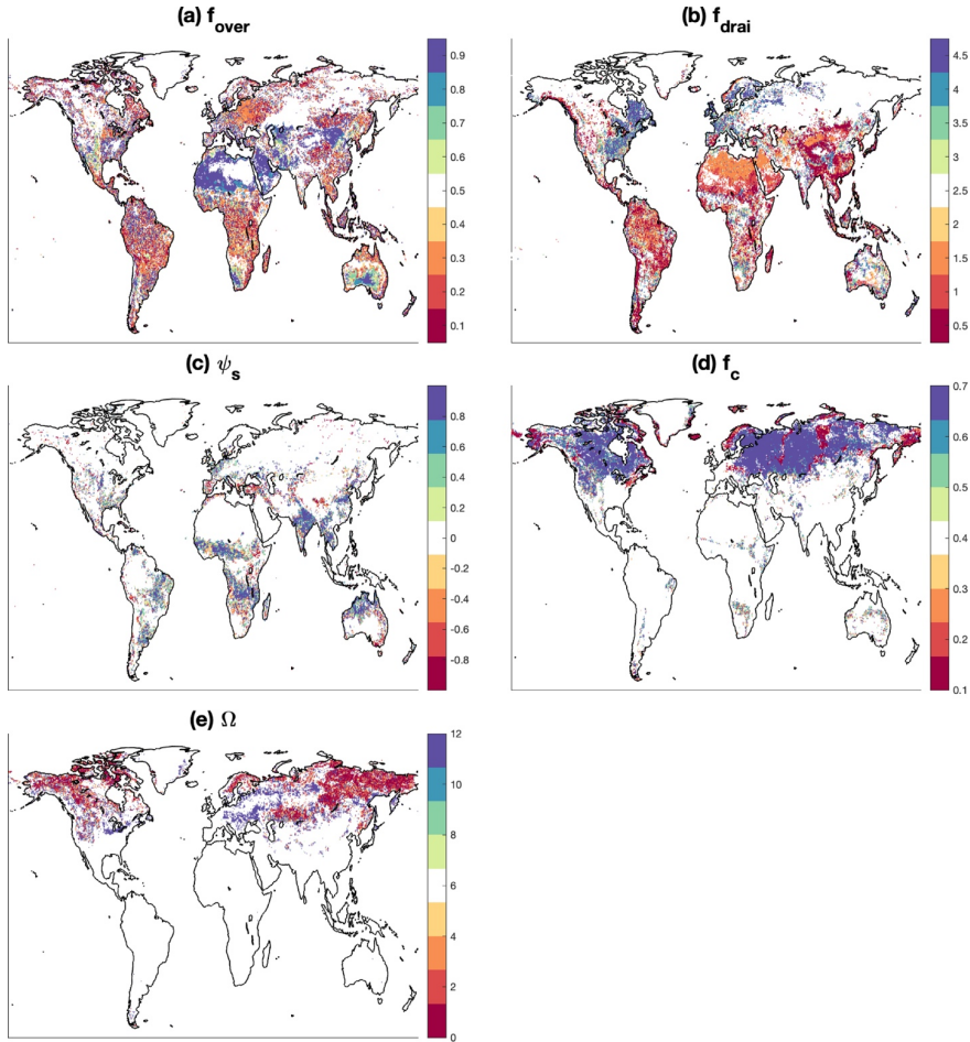
400 Figure 7. Optimal values for the sensitive parameters. The default values for the parameters are defined at the midpoint of the colormap. There are no certainty bounds for \psi_s from different grid cells because it is determined by the soil properties. Therefore, the values of \psi_s are scaled to [-1, 1] in subplot (c) for each grid cell with the corresponding upper bound
