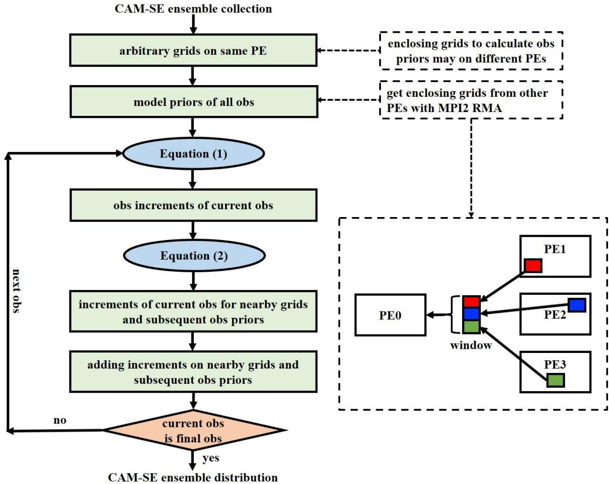
800 Figure 3. Schematic of the implementation of the parallel EAKF algorithm with CAM-SE. The implementation is also based on the two-step method of EAKF. In CAM-SE, the grid points are decomposed onto the analysis PEs via an arbitrary way. Therefore, the computation of the forward observation operator may need to obtain values from other PEs, which is realized through the MPI2 RMA technique. The lower-right dashed rectangular illustrates an example of grabbing data from PEs 1 – 3 to PE0 via a virtual window of RMA. When the observations at a given time are available, the prior ensembles for all observations are computed. The 805 observational increments of an observation regress not only on the nearby model states, but also on the subsequent observation prior ensembles.
