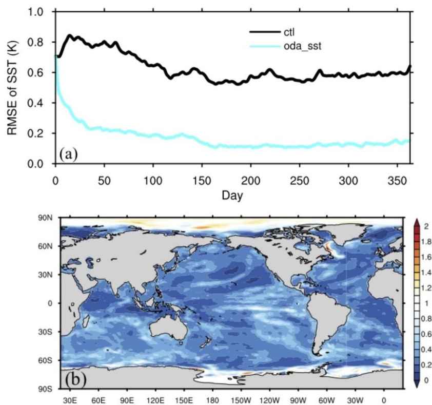
825 Figure 8. a) Time series of RMSE of SST from ctrl and oda_sst, and b) the distribution of the RMSE ratio (oda_sst/ctrl) of SST. The RMSE ratio is calculated with the data of the first three months excluded.
