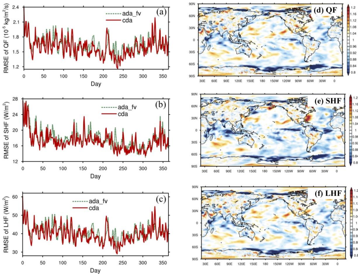
840 Figure 12. Time series of RMSEs of (a) water vapor flux QF, (b) sensible heat flux SHF, and (c) latent heat flux LHF from ada_fv and cda , the distribution of the RMSE ratio ( cda/ada_fv ) of (d) water vapor flux QF, (e) sensible heat flux SHF, and (f) latent heat flux LHF. The RMSE ratios are calculated with the data of the first month excluded.
