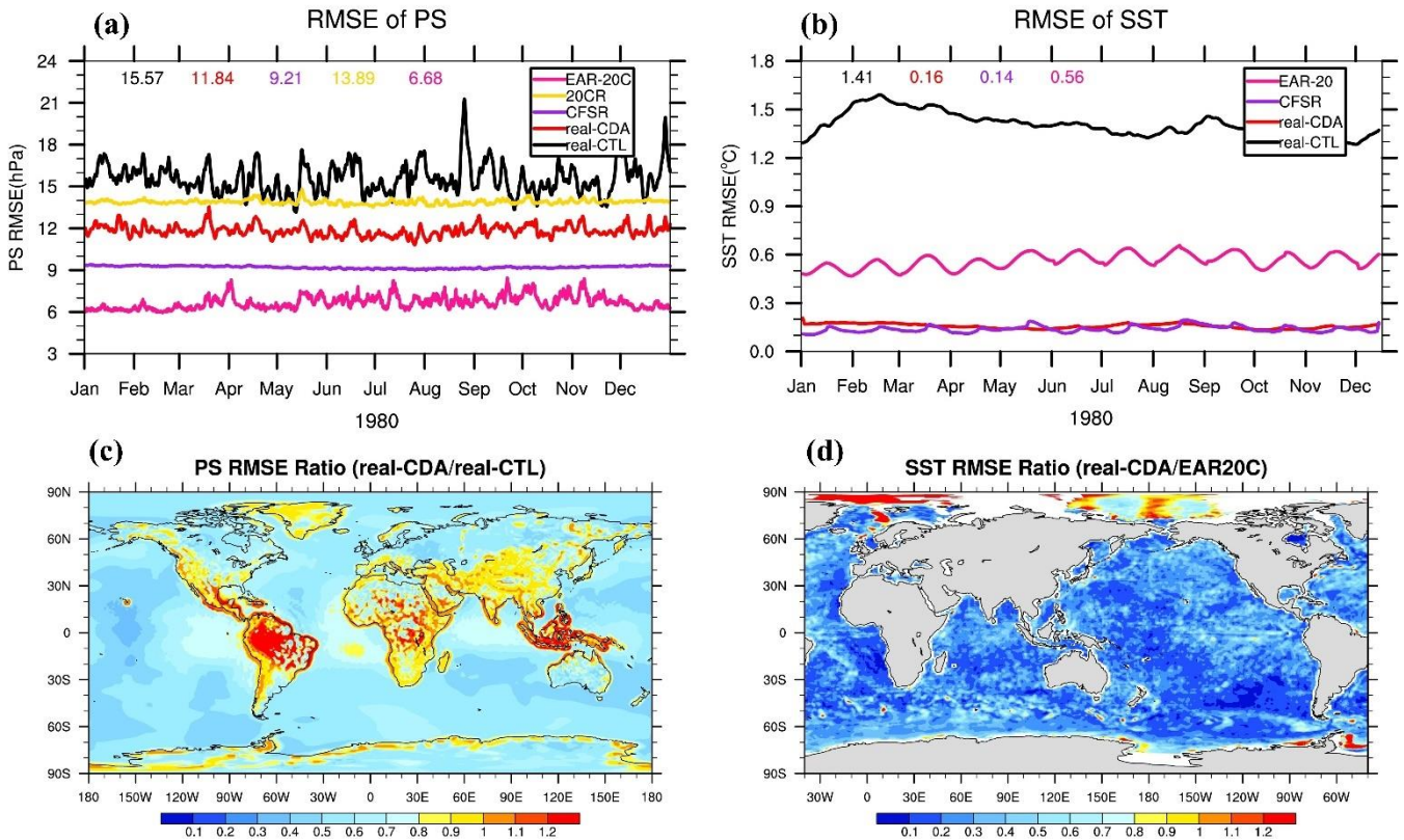
845 Figure 13. Time series of RMSE of a) Ps and b) SST from the real observation assimilating experiment and RMSE ratio distributions of Ps (real-CDA/real-CTL) and SST (real-CDA/EAR20C) in 1980. The number in a/b are RMSEs of the mean value corresponding to each product.
