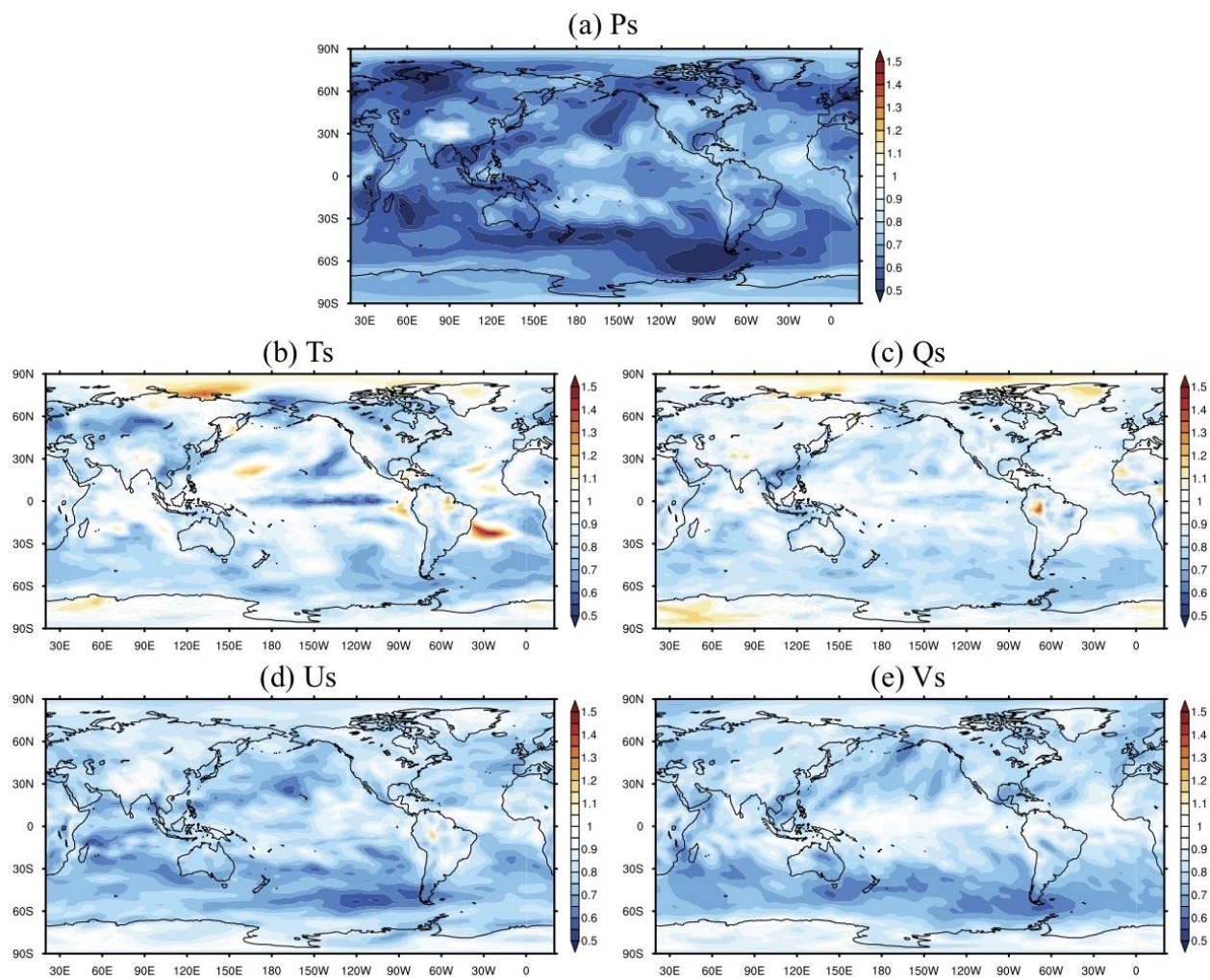
Figure 5. The distribution of the RMSE ratio (ada_fv/ctl) of (a) surface pressure Ps, (b) surface temperature Ts, (c) surface specific humidity Qs, (d) surface zonal wind Us, and (e) surface meridional wind Vs. The RMSE ratios are calculated with the data of the first month excluded.
