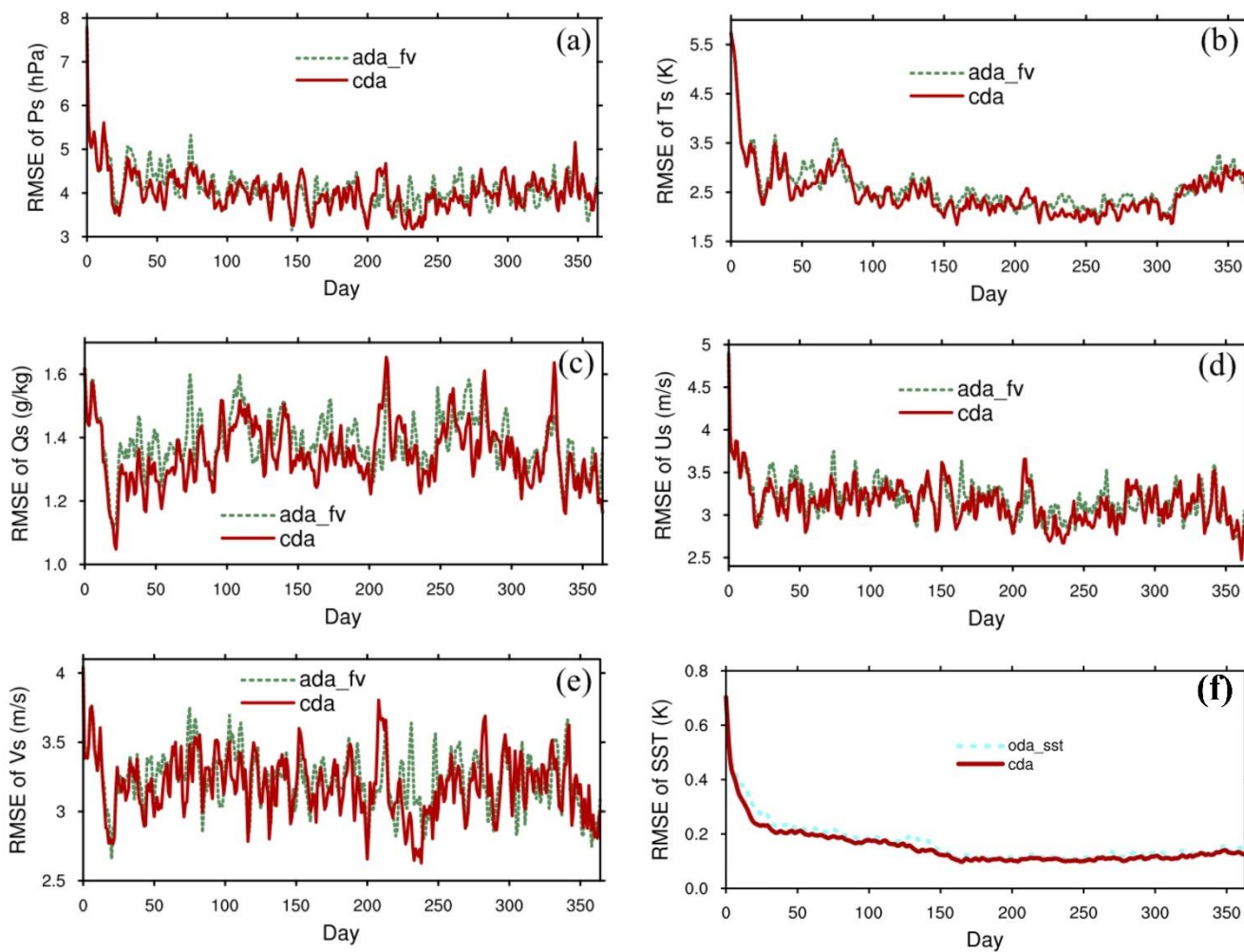
835 Figure 11. Time series of RMSEs of (a) surface pressure P_s , (b) surface temperature T_s , (c) surface specific humidity Q_s , (d) surface zonal wind U_s , (e) surface meridional wind V_s and (f) SST from ada_fv/oda and cda .
