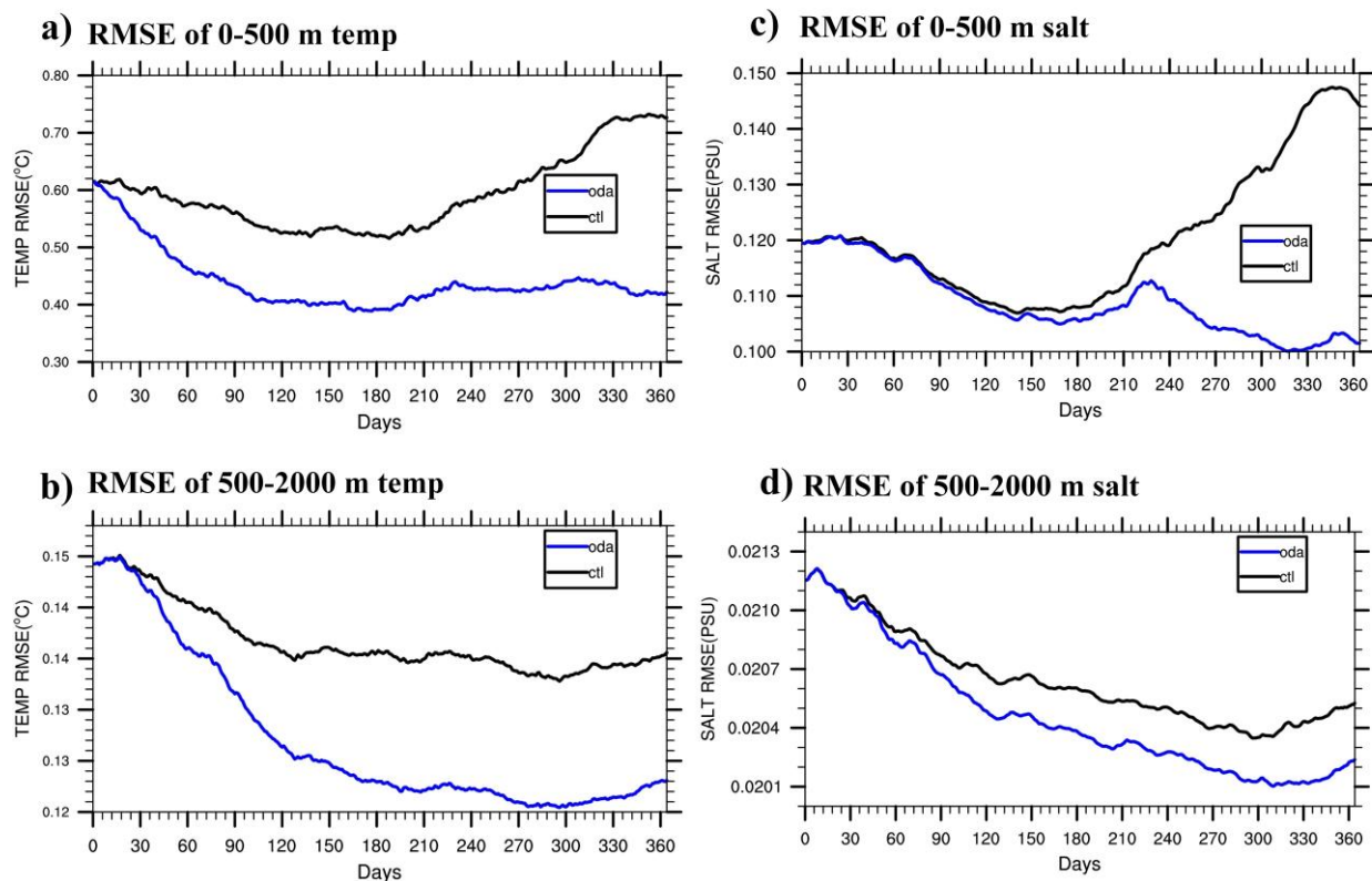
830 Figure 10. Time series of RMSEs of a) 0-500 m, b) 500-2000 m ocean temperature and c) 0-500 m, d) 500-2000 m ocean salinity from ctl (black line) and oda (blue line).
