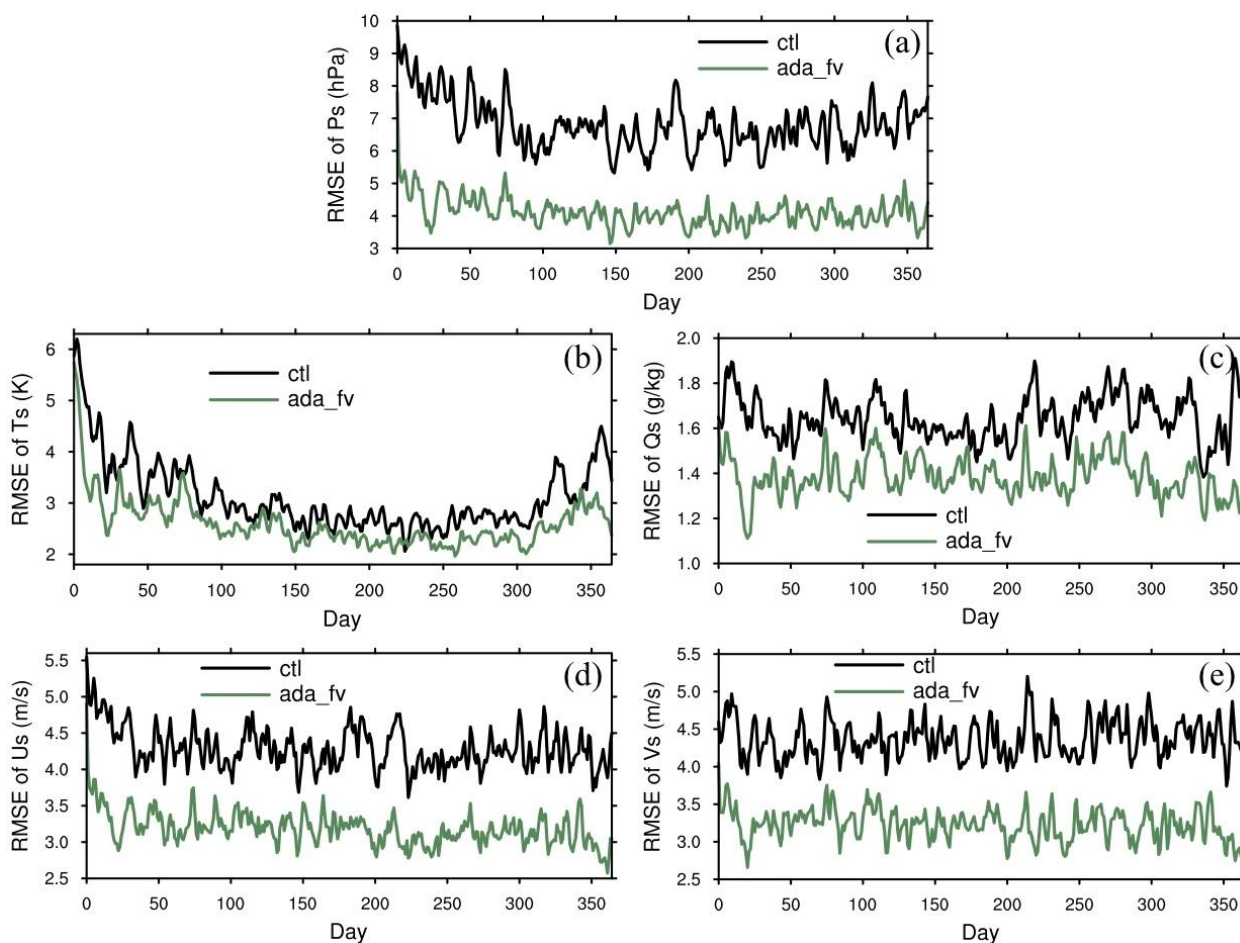
Figure 4. Time series of RMSEs of (a) surface pressure P_s , (b) surface temperature T_s , (c) surface specific humidity Q_s , (d) surface zonal wind U_s , and (e) surface meridional wind V_s from ctl and ada_fv.
