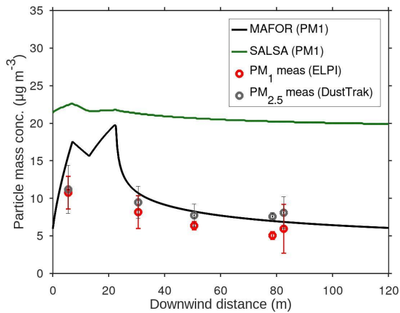
Figure 12. Comparison of total particle mass and black carbon concentrations in the “Urban Case” simulation: a) modelled particulate matter (PM 1 ) from MAFOR and SALSA together with measured PM 1 from ELPI (assuming particle density of 1000 kg m -3 ) and PM 2.5 from DustTrak (error bars represent 1σ standard deviation); b) modelled BC from MAFOR and SALSA together with measured BC from aethalometer (AE22, Magee Scientific; error bars represent 1σ standard deviation). Measurement data was obtained with the mobile lab Sniffer at location points A–E. Note that point E was excluded from the M–O comparison.
