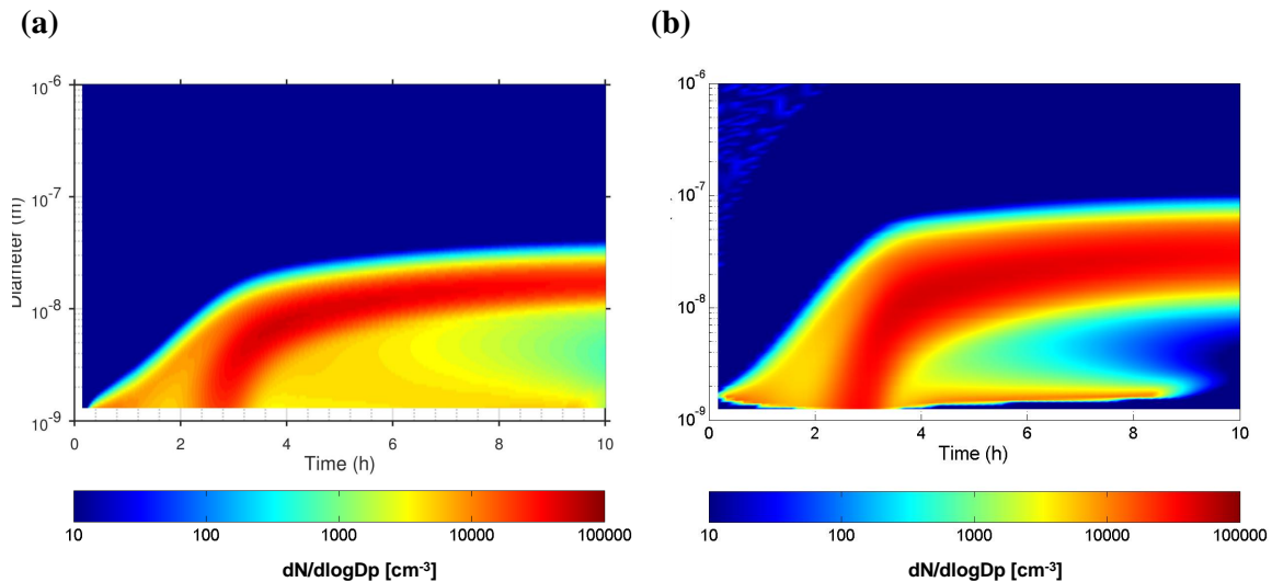
Figure 15. Evolution of the modelled particle number size distribution in a 10-h simulation to compare the performance of the nucleation code M2018 in a) MAFOR v2.0, to that in b) AEROFOR. New particles were inserted at 1.0 and 1.5 nm diameter, respectively, in MAFOR and AEROFOR. The first particle formation after 15 min is due to ion-induced nucleation, the main particle burst after 2 h is due to neutral nucleation. Final mean D_p was 18 and 22 nm, respectively, in MAFOR and AEROFOR simulations. Details on the configuration of the numerical experiment are given in Appendix H.
