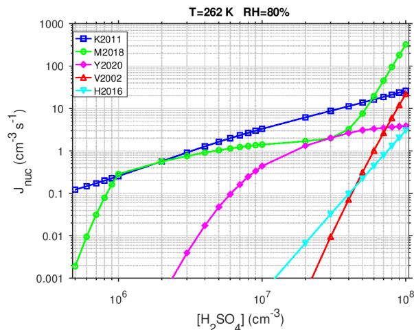
Figure 2. Predicted nucleation rate J_{\text{nuc}} ( \text{cm}^{-3} \text{ s}^{-1} ) as function of the concentration of \text{H}_2\text{SO}_4 (at T = 262 \text{ K} and \text{RH} = 80\% ) calculated with different parameterizations for particle formation through sulphuric acid: combined activation and IMN (K2011), neutral and ion-induced BHN (M2018), TIMN at \text{NH}_3 = 1 \times 10^5 \text{ cm}^{-3} (Y2020), THN at \text{NH}_3 = 2 \times 10^6 \text{ cm}^{-3} (H2016) and classical BHN (V2002).
