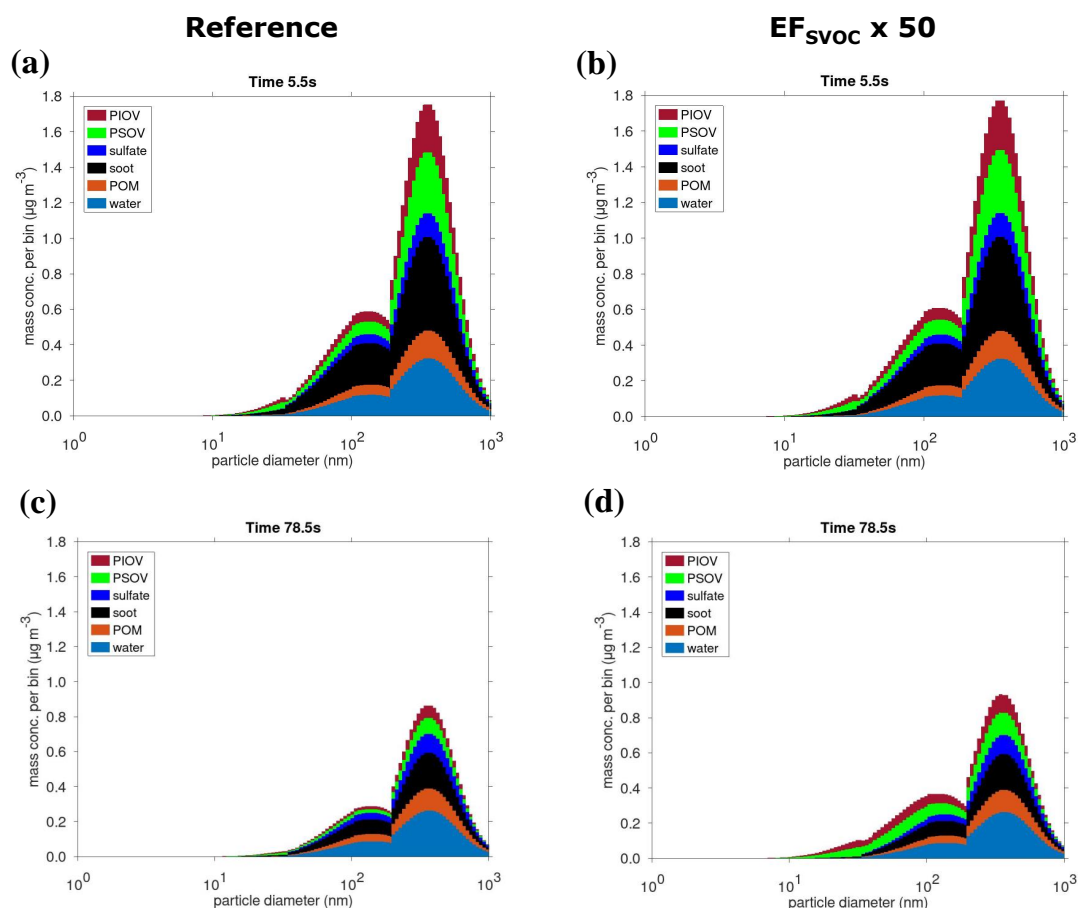
Figure 14. Aerosol chemical composition obtained from the MAFOR model, given as mass concentration per size bin, in the “Urban Case” scenario: a) reference simulation at point A; b) simulation EF_{\text{SVOC}} \times 50 at point A; c) reference simulation at point D; and d) simulation EF_{\text{SVOC}} \times 50 at point D.
