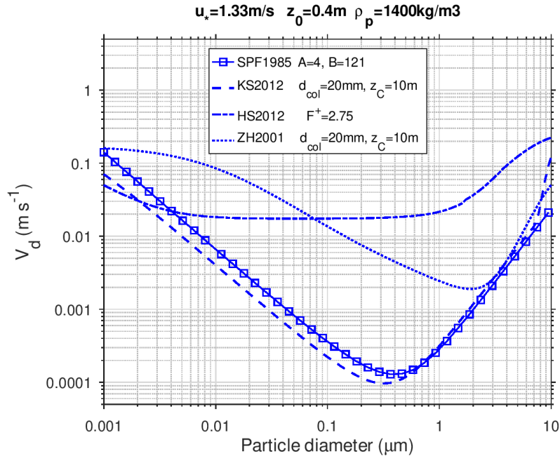
Figure 4. Dry deposition of particles over rough urban surface calculated with the SPF1985 scheme (solid line with squares), KS2012 scheme (lower dashed line), and HS2012 scheme (upper dashed line), and ZH2001 scheme (dotted line), using u^* = 1.33 \text{ m s}^{-1} , z_0 = 0.4 \text{ m} and average particle density of 1400 \text{ kg m}^{-3} . Specific parameter values are given in the legend.
