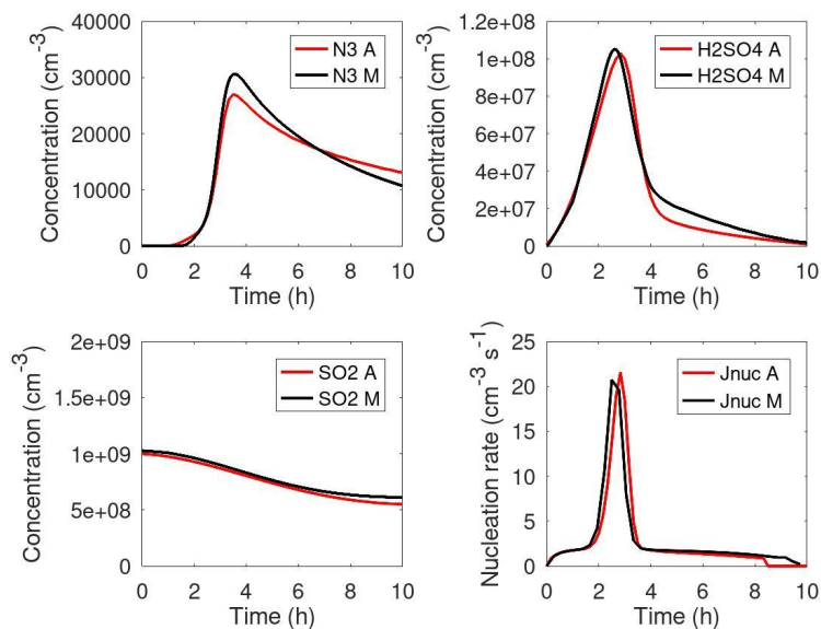
Figure H1. Comparison of modelled total particle number with diameter > 3 nm ( N_3 ), gas-phase concentrations of H_2SO_4 and SO_2 , and nucleation rate from MAFOR v2.0 (black lines) and AEROFOR (red lines) in a test of the new nucleation parameterization M2018 for new particle formation under clear-sky conditions ( T = 267 K, RH = 90\% ). The simulations started at 8 am local time.
