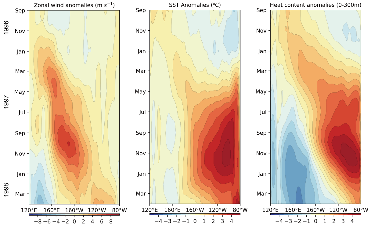
Figure 16. Longitude-time diagram of monthly surface zonal wind anomalies (left), SST anomalies (middle), and heat content (t300) anomalies (right) across the equatorial Pacific ( 2^{\circ}N - 2^{\circ}S , 120^{\circ}E - 80^{\circ}W ) from September 1996 to April 1998. Data are based on NCEP Global Ocean Data Assimilation System and ERA-5.
