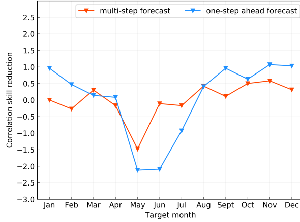
Figure 14. The decline of forecasting skills for ENSO in each target month using multi-step forecast strategy and one-step ahead forecast strategy.
