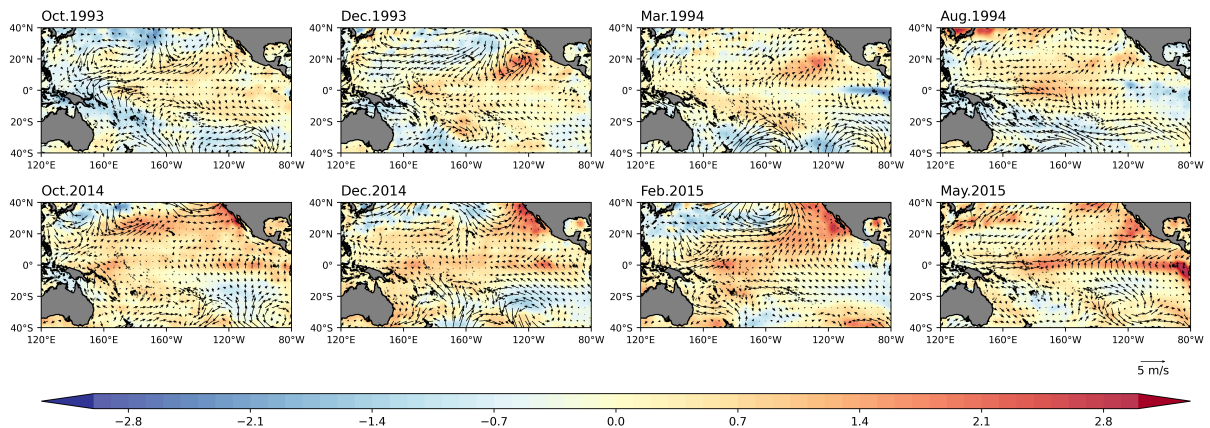
Figure 17. The SST and 10-m wind-vector anomalies for the different seasons before 1994/1995 CP Niño and 2015/2016 EP Niño.
