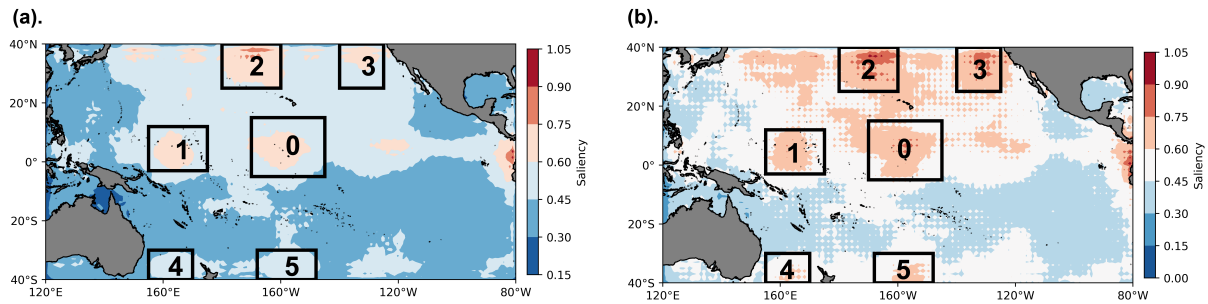
Figure 18. The composite saliency maps of surface (a) and subsurface (b) over 40^{\circ}N - 40^{\circ}S , 120^{\circ}E - 80^{\circ}W . The higher the saliency value, the more sensitive the area. Since the saliency map results obtained from the surface layer and the subsurface layer may affect each other, we first select six common areas with large values as candidates to perform sensitivity experiments. The six areas are the central equatorial Pacific (0), the western equatorial Pacific (1), the northern Central Pacific (2), the northeastern Pacific (3), the southwestern Pacific (4) and the southern Central Pacific (5).
