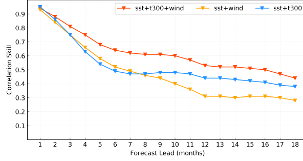
Figure 3. The correlation skill of Nino 3.4 index of ENSO-MC model with different predictors.
