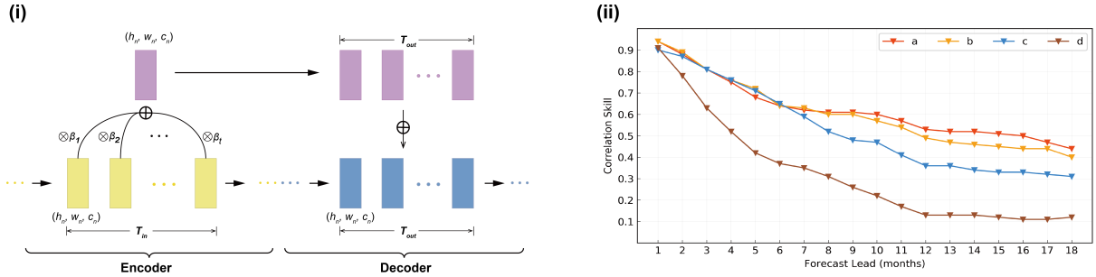
Figure 4. (i) The detailed structure of the skip-layer connection and attention mechanism between encoder and decoder at the n^{th} layer in ENSO-MC. (ii) The correlation skill of Nino 3.4 index of the forecast lead month in models with different structures: (a) ENSO-MC model of skip-layer connection with attention mechanism and states connection, (b) ENSO-MC model without attention mechanism, (c) ENSO-MC model without states connection, (d) ENSO-MC model without skip-layer connection.
