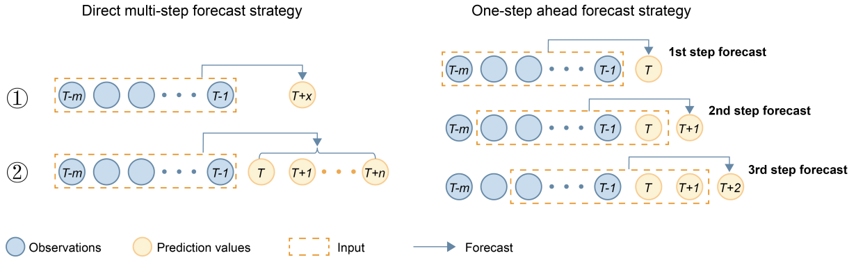
Figure 2. Two main strategies of multi-step forecasting for ENSO prediction, direct multi-step forecast strategy and one-step ahead forecast strategy. And direct multi-step forecast strategy has two methods, the second one is used in this paper.
