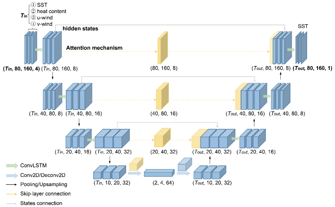
Figure 2 The encoder-decoder architecture of ENSO-MC for SST pattern sequence prediction. The encoder contains three ConvLSTM layers and each layer is followed by a pooling layer, and the last layer is a convolutional layer, which allows extracting spatial and temporal features. And the decoder comprises one deconvolutional layer, three ConvLSTM layers and three upsampling layer that restores the features to the same size as the initial spatial dimension ( 80 \times 160 ). The model uses skip-connection with attention mechanism and state-connection between the encoder and the decoder to improve forecasting skills. The input variables are the SST, heat content, zonal wind and meridional wind for T_{in} consecutive months over 40^{\circ}\text{N} - 40^{\circ}\text{S} , 120^{\circ}\text{E} - 80^{\circ}\text{W} ( 80 \times 160 , 1^{\circ} \times 1^{\circ} resolution) and each type of variable is input to the model as a channel. The output of the model is SST pattern sequence for the next T_{out} months.
