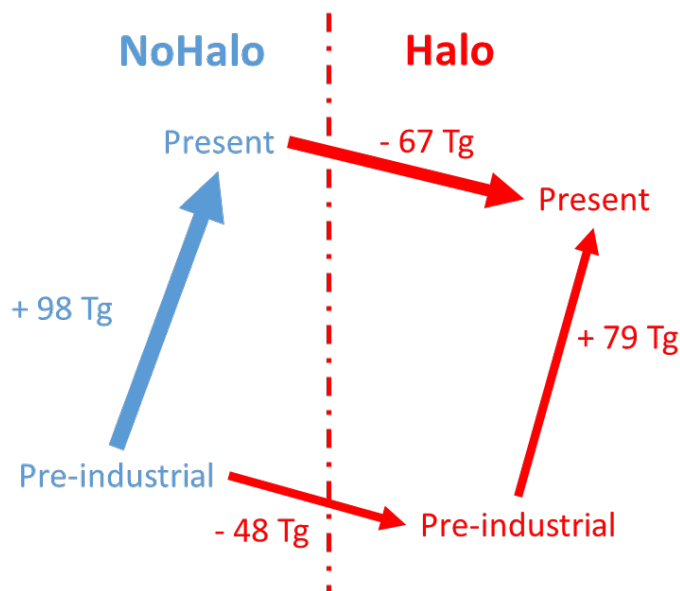
405 Figure 7: Schematic representation of the evolution of ozone mass budget changes between PI and PD, following the inclusion of halogen chemistry in LMDZ-INCA.
