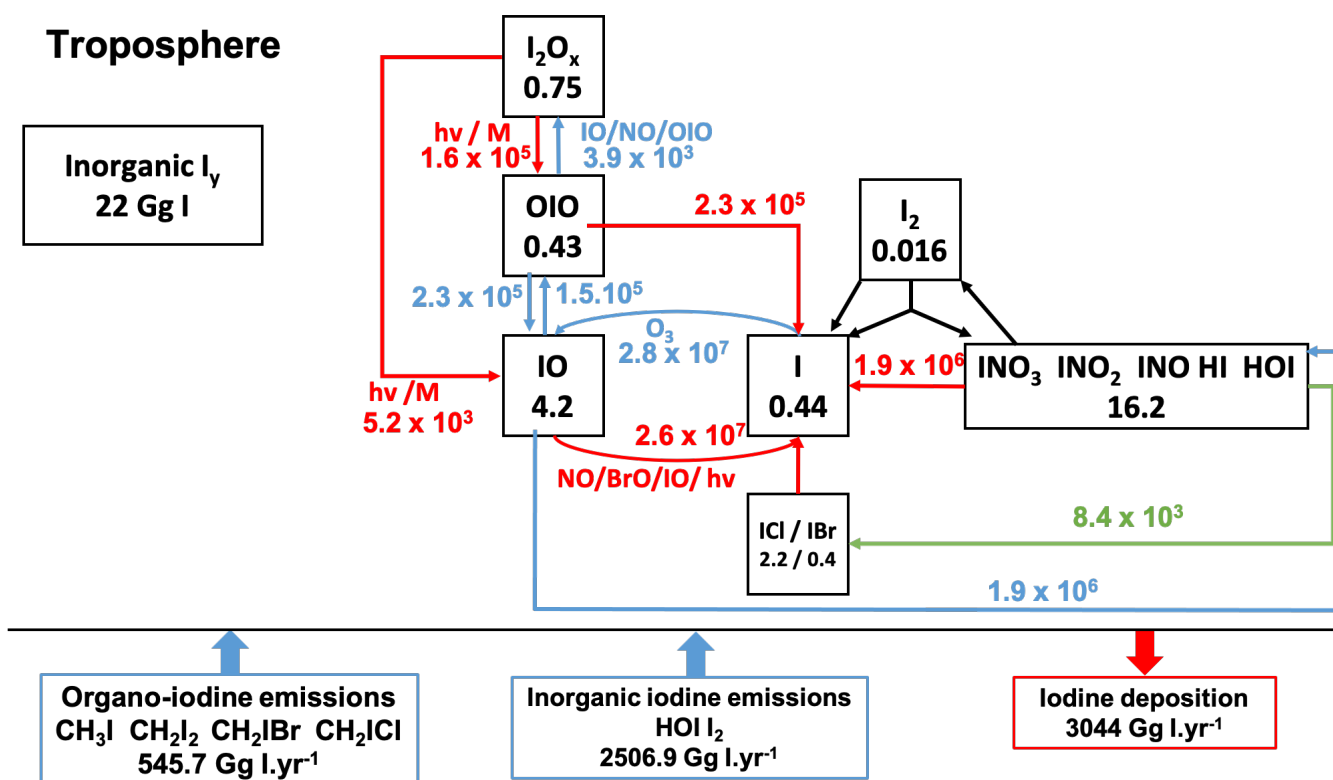
310 Figure 4: Iodine budget in the present-day reference simulation with simplified cycle of tropospheric \text{I}_y species. Heterogeneous reactions are shown in green. Photolysis reactions are in red. The numbers in the boxes represent the mass balance of the species families in \text{Gg I} .
