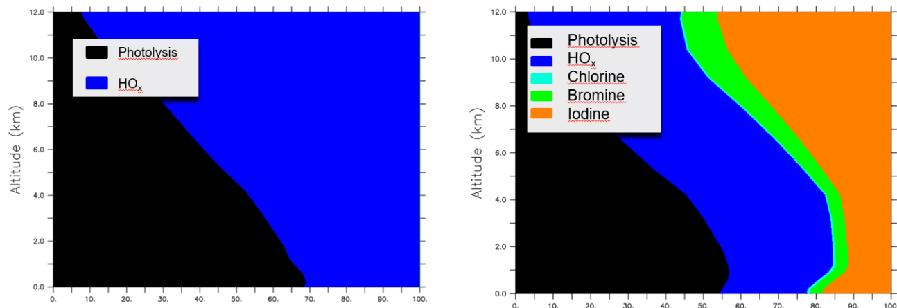
250 Figure 3: Contribution of the chemical ozone sinks as a function of the altitude without (left) and with (right) consideration of the chemistry of halogens in LMDZ-INCA.
