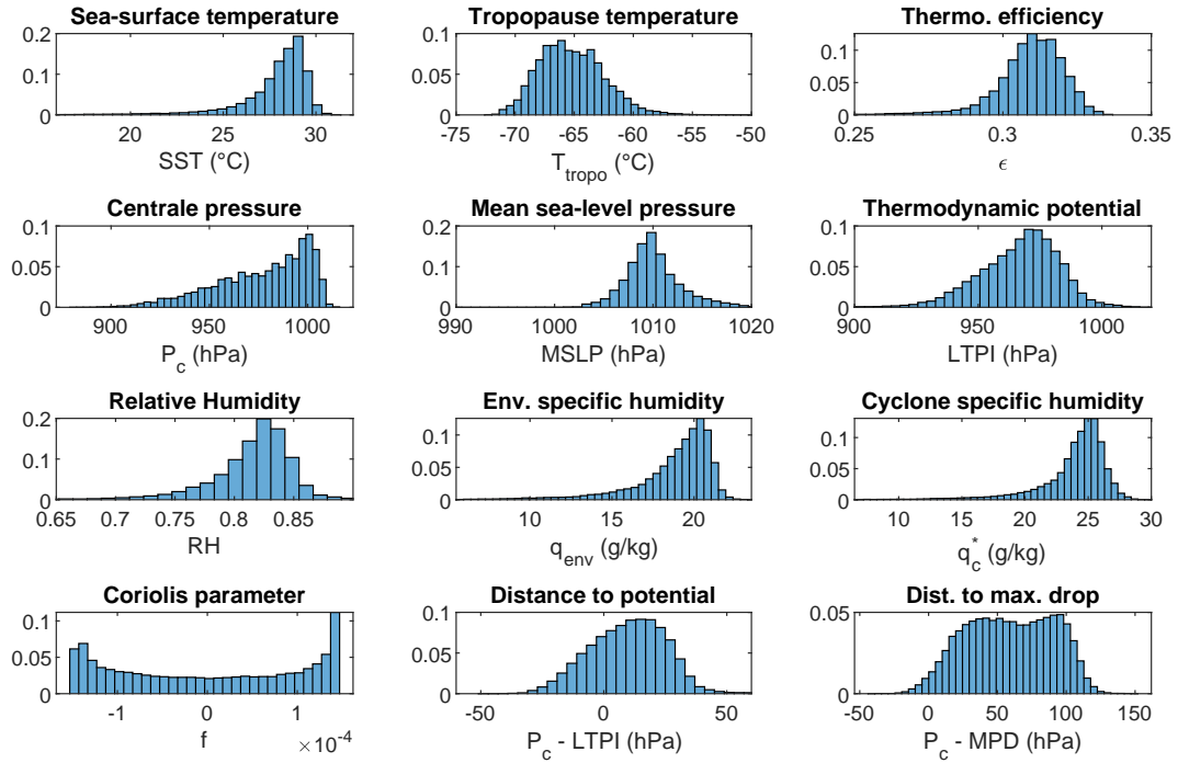
Figure 7. Empirical distribution of physical properties along tracks (IBTrACS and ERA-5), and distribution of instrumental variables of CATHERINA
