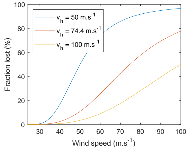
Figure 18. Fraction of property value lost as a function of wind speed, obtained using Equation (18) with different values of v_h . Source: Emanuel (2011).
