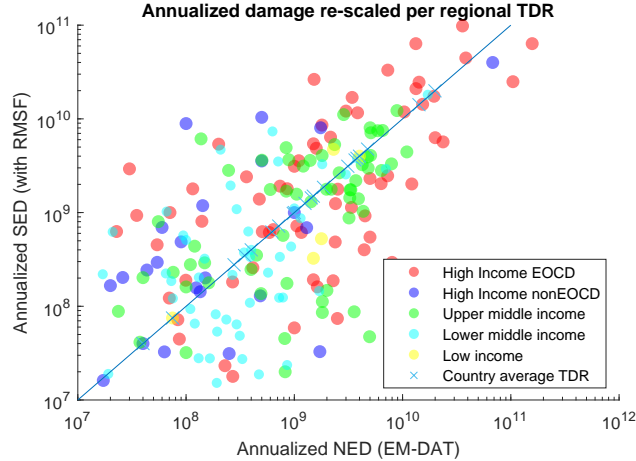
Figure 20. Estimated (RMSF) vs. reported damage. The filled dots represent individual year/country pairs with reported damage in EM-DAT. The small targets represent countries average and large targets income groups average. This distribution is obtained using a 0.25 x 0.25 resolution projection. Crosses correspond to country average (over all years).
