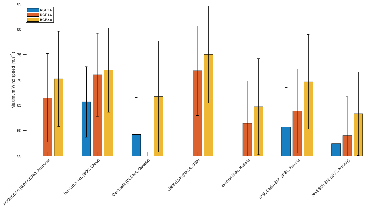
Figure 23. Average and standard deviation of maximum wind speed of tropical cyclones generated with the CMIP5 models after correction. Table A4 provide average value of maximum wind speed.
