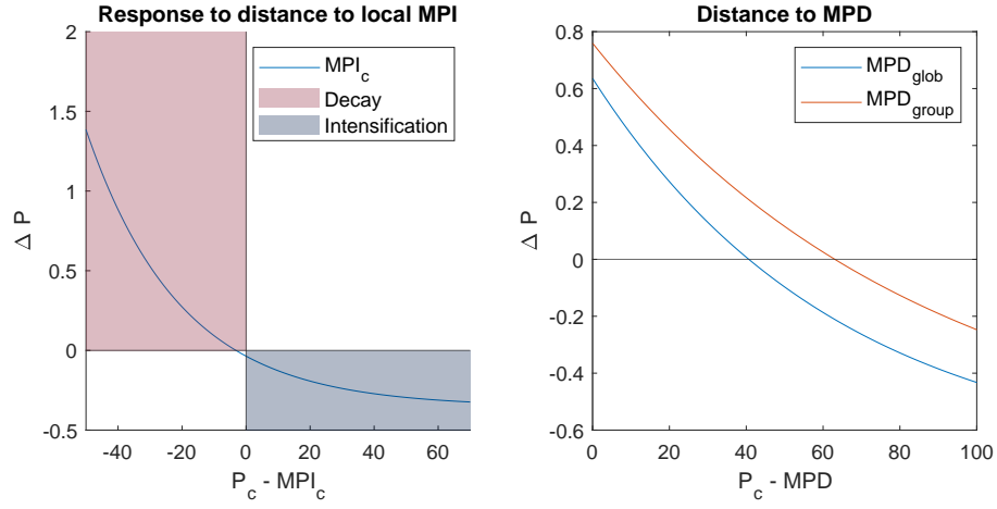
Figure 9. Response of the depression dynamics model to distance to thermodynamic potentials over intensification factor domains
