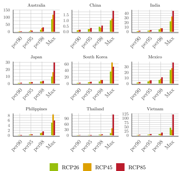
Figure 27. Damage cost channeled to excess spread (cost of debt) of different countries, basis points.
