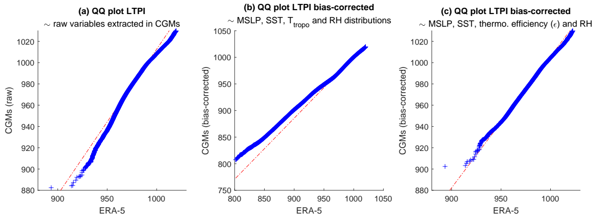
Figure 21. Bias correction module QQplots
