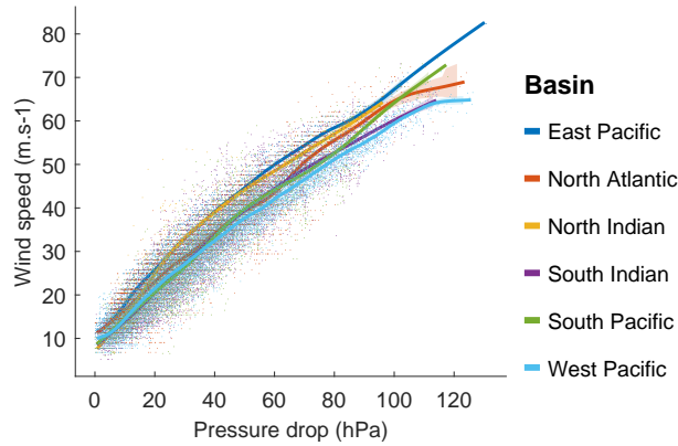
Figure 6. Maximum wind and pressure drop values from IBTrACS together with the fit of Equation (3). The coefficients a and b fitted per basin are provided in Table A2.
