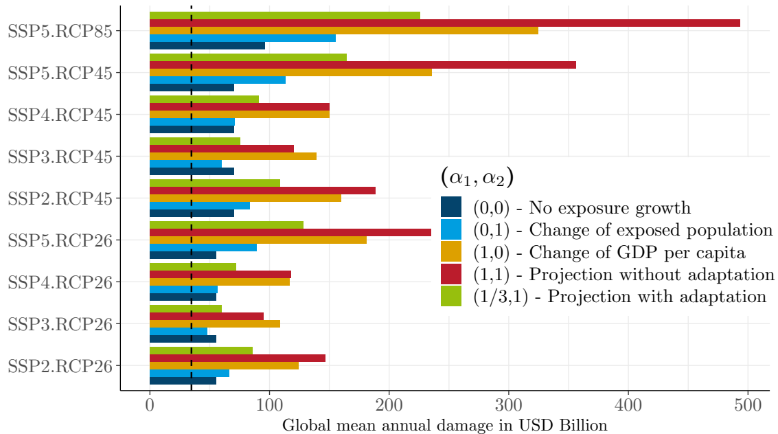
Figure 24. Simulated-expected Expected value of global annual damage (2014- in USD Billionsbillions) in historical-calibration-period different SSP-RCP and representative-concentration-pathways-between-2075-and-2100 exposure projection hypothesis configurations. The vertical dotted line corresponds to historical simulations with ERA5 data.
