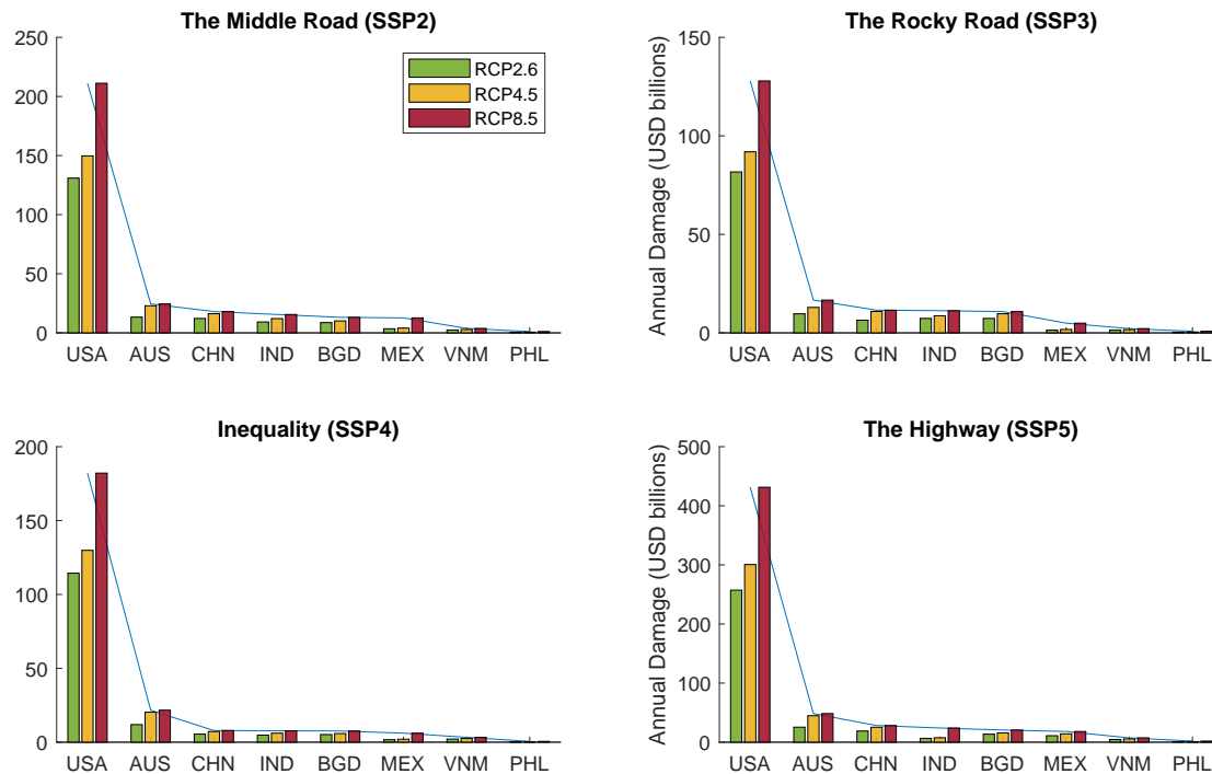
Figure 25. Annualized regional expected damage in SSP and RCP between 2070 and 2100 based on synthetic tracks produced with 7 climate models (with bias correction) over 300 representative years launched independently. The scale differs between SSPs.
