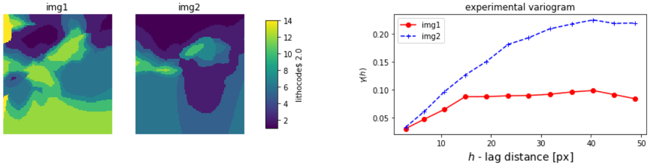
Figure 8. Example of experimental semi-variogram for two lithocode voxets, computed for the lithocode value of 2; the two first columns show an horizontal section for each voxet; the last column shows the two corresponding experimental semi-variogram.
