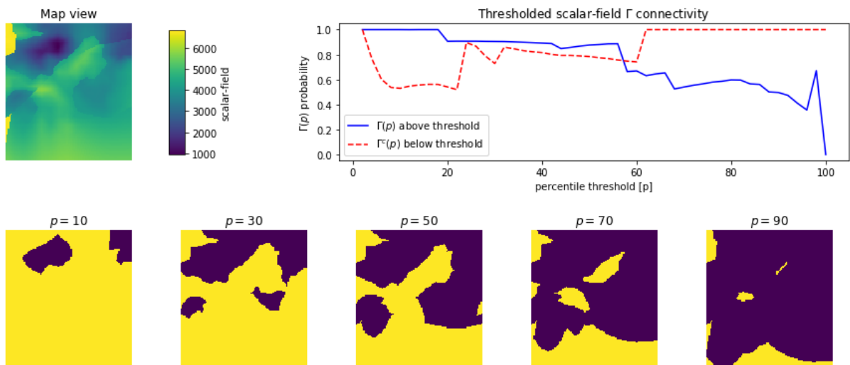
Figure 10. Illustration of a scalar-field voxel horizontal section (top left) and its global percolation metrics \Gamma(p) and \Gamma(p)^c = \Gamma^c(p) (top right) computed over the 2D sections; the bottom row displays horizontal sections of binary fields obtained by applying different percolation threshold p[\%] to the scalar-field 3D voxel; blue areas, above the percolation threshold p[\%] , contribute to \Gamma(p) ; yellow areas, below the percolation threshold, are used to compute \Gamma(p)^c = \Gamma^c(p) .
