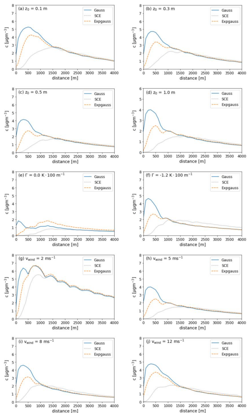
840 Figure D2: Comparison for ground-level concentration values depending on the distance to the source for different settings and initial profiles. Default input settings ( v_{\text{wind}} = 5 \text{ m s}^{-1} , v_{\text{exit}} = 10 \text{ m s}^{-1} , T_{\text{exh}} = 300 \text{ °C} , \Gamma = -0.65 \text{ K} \cdot 100 \text{ m}^{-1} , \phi = 0^\circ and z_{0, \text{land}} = 1 \text{ m} ) were used for all but one parameter. Panels (a)–(d) vary roughness lengths over land, panels (e) and (f) vary atmospheric stability. Panels (g)–(j) vary wind speed. Panel (h) represents full default conditions.
