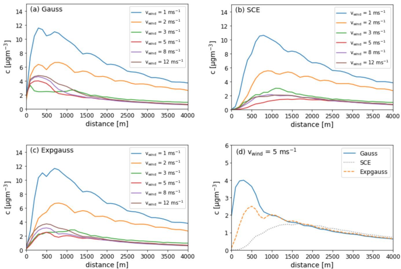
820 Figure 10: (a–c) Ground-level concentration profiles depending on the distance to the source for different wind speeds and initial emission distribution; (d) direct comparison of the effect of different emission distribution at v_{\text{wind}} = 5 \text{ m s}^{-1} .
