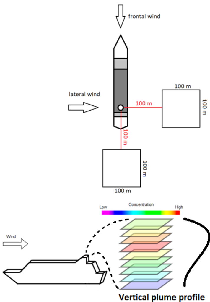
825 Figure A1: Scheme for deriving the vertical plume concentration profile from MITRAS. Concentration values are derived from mean column values of 100 m · 100 m horizontal and 10 m vertical size in a distance of 100 m downwind from the ship to include plume rise and obstacle-induced turbulence in the emission profile. Adjusted from Badeke et al. (2021).
