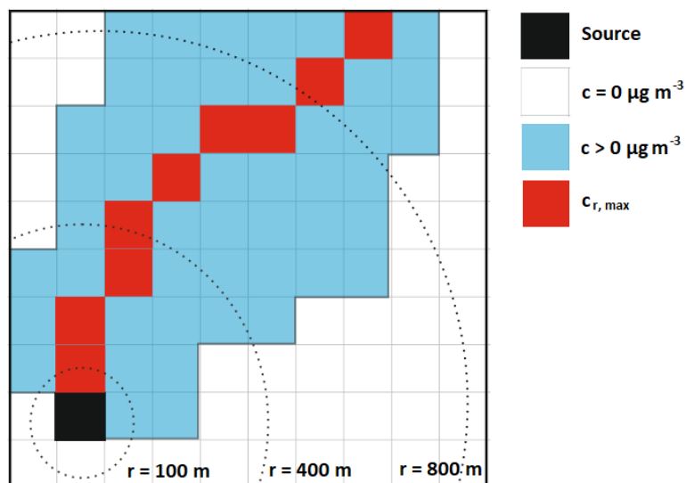
830 Figure A2: Scheme for deriving ground-level concentration versus distance plots. Top view of the lowest model layer grid. The grid has a resolution of 100 m · 100 m. Blue cells are affected by the plume concentration, while white cells are not. For every radius of r = 100 m to r = 4000 m a circular function is applied to determine the highest concentration value along the perimeter. This is exemplarily shown for r = 100 m, 400 m and 800 m. Red cells show the resulting path of highest ground-level concentration.
