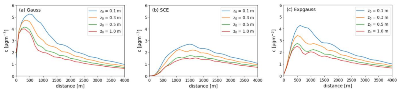
815 Figure 8: Ground-level concentration profiles depending on the distance to the source for different roughness lengths and initial emission distribution.
