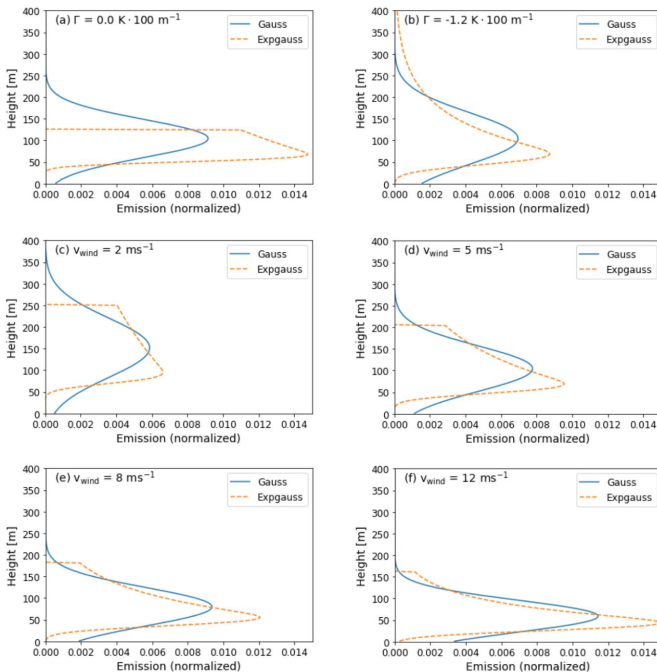
835 Figure D1: Initial EPISODE-CityChem emission profiles under default input settings ( v_{\text{wind}} = 5 \text{ m s}^{-1} , v_{\text{exit}} = 10 \text{ m s}^{-1} , T_{\text{exh}} = 300 \text{ }^\circ\text{C} , \Gamma = -0.65 \text{ K} \cdot 100 \text{ m}^{-1} , \phi = 0^\circ and z_{0, \text{land}} = 1 \text{ m} ) for all but one parameter. Panels (a) and (b) show effects of varying the stability while panels (c)–(f) show effects of varying the wind speed. Panel (d) represents full default conditions.
