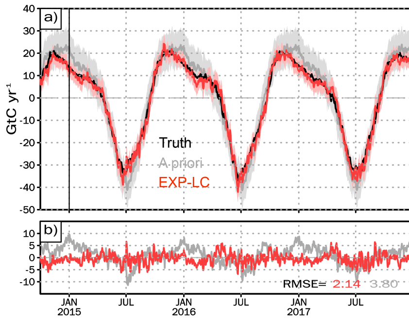
325 Figure 5: a) The global daily FTA of truth (black), a priori (gray), and analysis of EXP-LC (red). The vertical line on 1 January 2015 indicates the start of assimilation. Before 1 January 2015, the system spin-up lasted for three months. The gray and red shadings are the ensemble spread of the a priori and analysis, respectively. b) The difference compared with the truth. The RMSE at the right-bottom corner is the root-mean-square error of the analysis (red) and a priori (gray) calculated based on Eq. 12.
