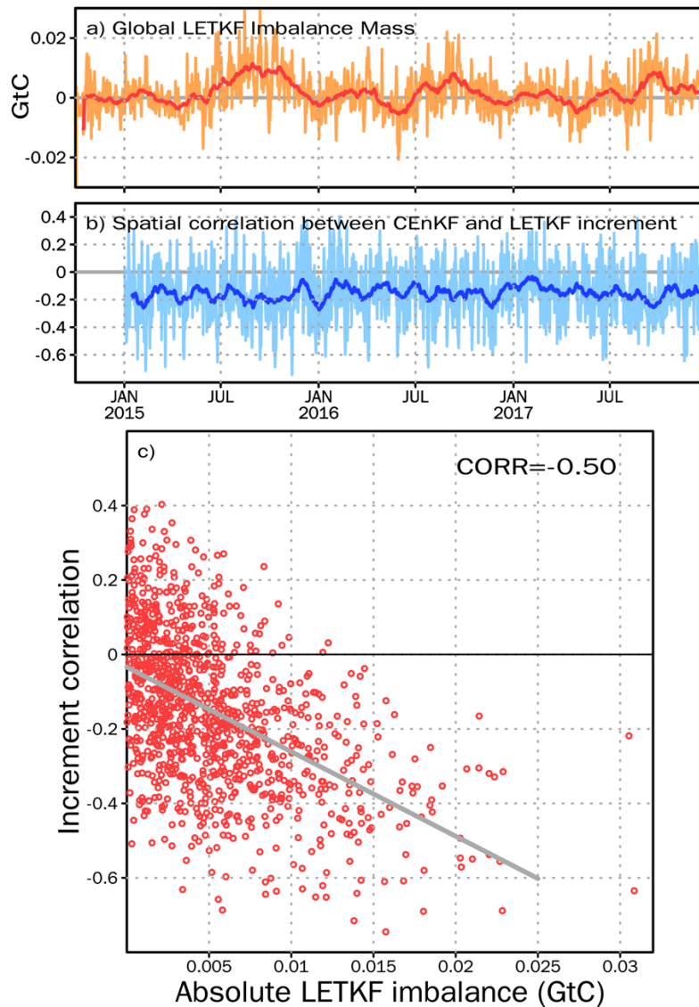
415 Figure 13: (a) The global mass imbalance caused by LETKF. The orange line is the ensemble mean of the global mass imbalance. The red line is calculated from the orange line using the 30-day moving average method. (b) The sky-blue line is the surface spatial correlation between the CEnKF increment and the LETKF increment at each assimilation time. The blue line is calculated from the sky-blue line using the 30-day moving average method. Note that during the spin-up period, the CEnKF is not applied. Thus, there are no correlations. (c) The red dots indicate the relationship between the increment correlation (sky-blue line in (b)) and the absolute LETKF imbalance (orange line in (a)) at each assimilation time. The gray line is the linear least squares regression fits to the scatter dots. The correlation is shown in the upper right corner.
