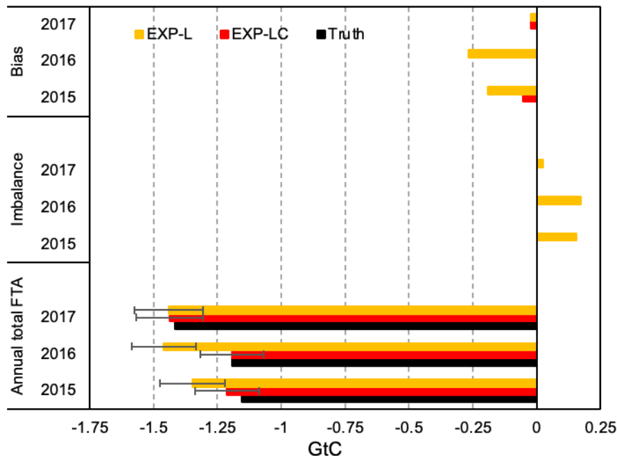
365 Figure 9: The global annual total FTA, imbalance, and bias of EXP-LC (red) and EXP-L (orange) compared with the truth (black) in 2015, 2016, and 2017. The imbalance is the mass loss for each year. The bias is the analysis of EXP-L and EXP-LC compared with the truth for each year. Note that there is no imbalance problem for EXP-LC. The error bar of the annual total is the uncertainty.
