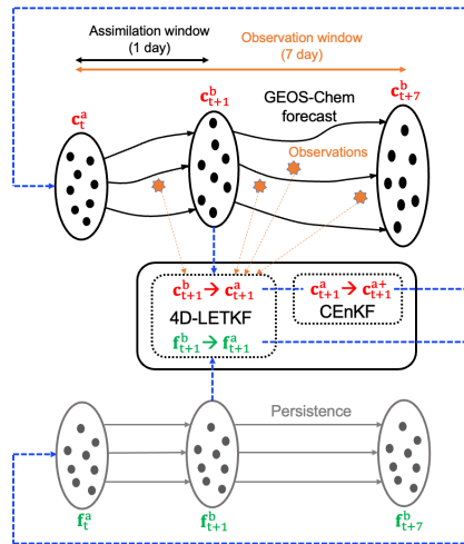
Figure 1: Flowchart of the COLA system.
