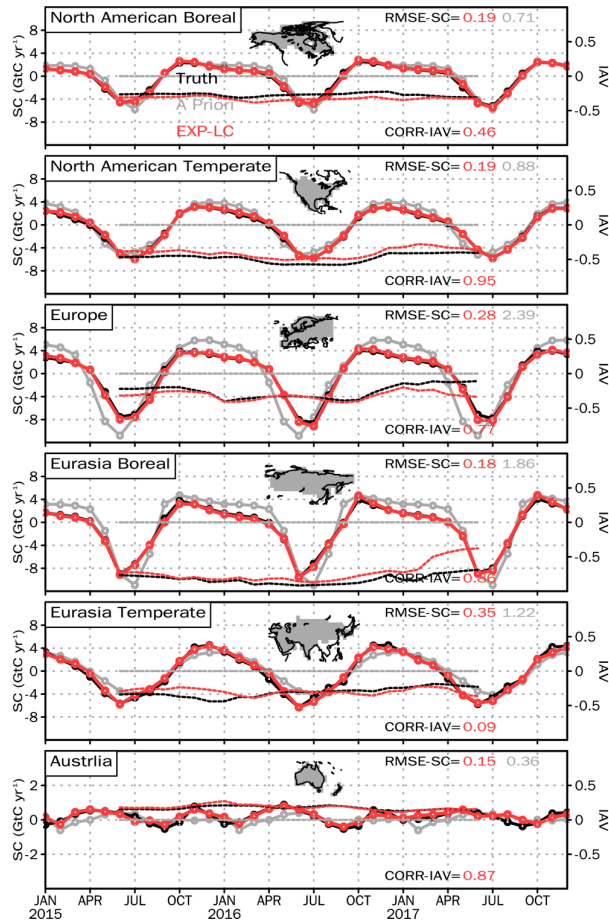
350 Figure 6: The FTA seasonal cycle (SC) and interannual variation (IAV) in truth (black), a priori (gray), and analysis of EXP-LC (red) over the Northern Hemisphere regions and Australia. The solid lines marked with open circles are the SC. The dashed lines are the IAV calculated from the original SC using a 12-month moving average method. The RMSE in the right-up corner is the SC root-mean-square error of the analysis (red) and the a priori (gray) calculated based on Eq. 12. The correlation (CORR) in the right-bottom corner is the IAV correlation between the analysis and the truth (the red dashed line and the black dashed line). Note that there is no IAV in the a priori. Thus, there is no IAV correlation between the a priori and the truth.
