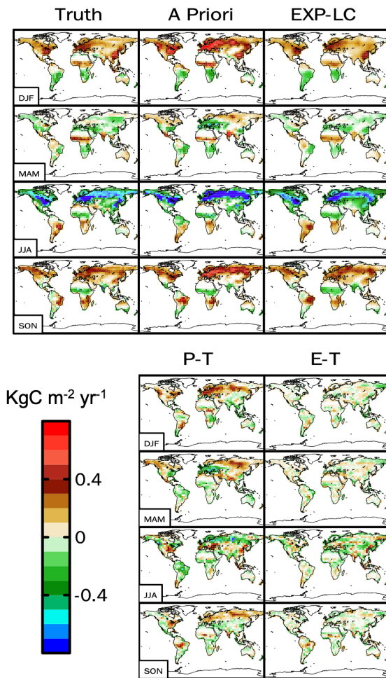
360 Figure 8: The top three columns are the FTA climatological seasonal cycle of the truth, a priori, and EXP-LC from December to February (DJF), March to May (MAM), June to August (JJA), and September to November (SON). The bottom two columns are the difference between the a priori and truth (P-T) and between the EXP-LC and truth (E-T).
