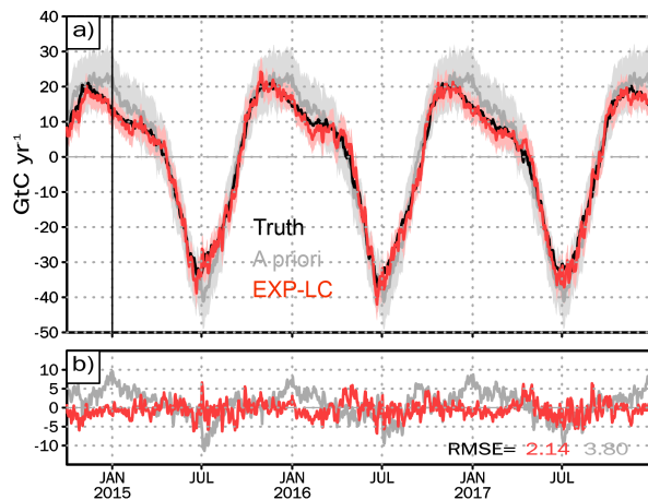
340 Figure 5: a) The global daily FTA of truth (black), a priori (gray), and analysis of EXP-LC (red). The vertical line on 1 January 2015 indicates the start of assimilation. Before 1 January 2015, the system spin-up lasted for three months. The pale gray and pale red shadings are the ensemble spread of the a priori and analysis, respectively. b) The difference compared with the truth. The RMSE at the right-bottom corner is the root-mean-square error of the analysis (red) and the a priori (gray) calculated based on Eq. 12.
