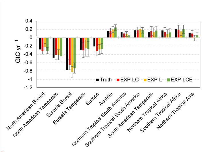
390 Figure 10: The total regional FTA of EXP-LC, EXP-L, EXP-LCE, and the truth from January 2015 to December 2017. The error bar of EXP-LC, EXP-L, and EXP-LCE is the uncertainty.
