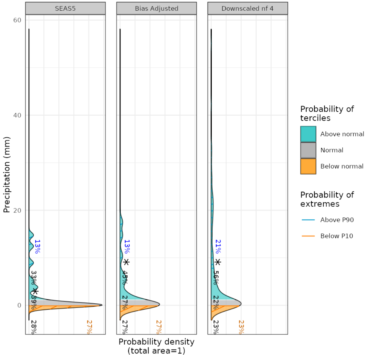
Figure A1: From left to right, PDF for the original, the bias-corrected by quantile mapping and the downscaled precipitation data (for refinement factor 4) SEAS5 for a grid point corresponding to a observational site in the Alps on the 11th of December 1993. For each PDF, three categories of equal size are shown: terciles above normal (blue), normal (grey) and below normal (orange), defined according to the area average of ERA5 reanalysis for the period 1993-2018. Percentages represent the forecast probabilities of each tercile, the most likely tercile is highlighted with a star and the blue and orange percentages represent the probabilities for P10 and P90 (hatched areas), respectively.
