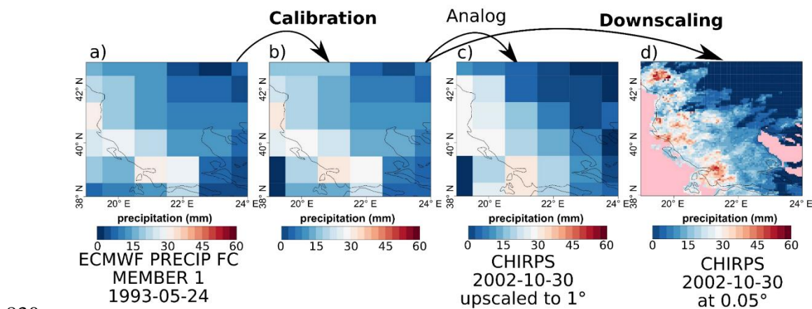
830 Figure 14: Comparison of the original forecast (a), bias-adjusted forecast (b), the analog (c) and the downscaled (d) forecast over Greece for SEAS5 for the 24th of May 1993.
