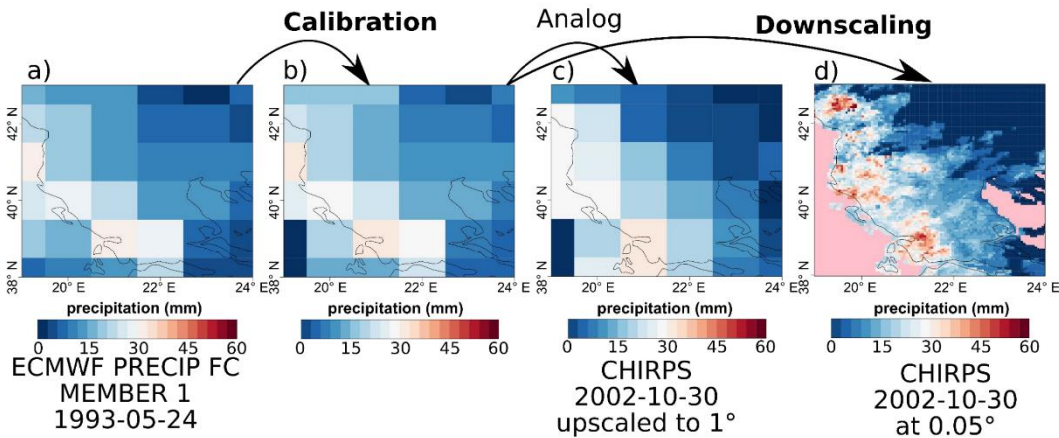
Figure 14: Comparison of the original forecast (a), bias-adjusted forecast (b), the analog (c) and the downscaled (d) forecast over Greece for SEAS5 for the 24th of May 1993.
