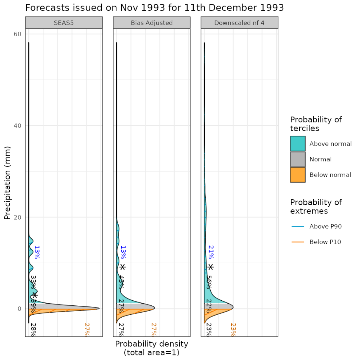
Figure A1: From left to right, PDF for the original, the bias-corrected by quantile mapping and the downscaled precipitation data (for refinement factor 4) SEAS5 for a grid point corresponding to a observational site in the Alps on the 11th of December 1993. For each PDF, three categories of equal size are shown: terciles above normal (blue), normal (grey) and below normal (orange), defined according to the area average of ERA5 reanalysis for the period 1993-2018. Percentages represent the forecast probabilities of each tercile, the most likely tercile is highlighted with a star and the blue and orange percentages represent the probabilities for P10 and P90 (hatched areas), respectively.
