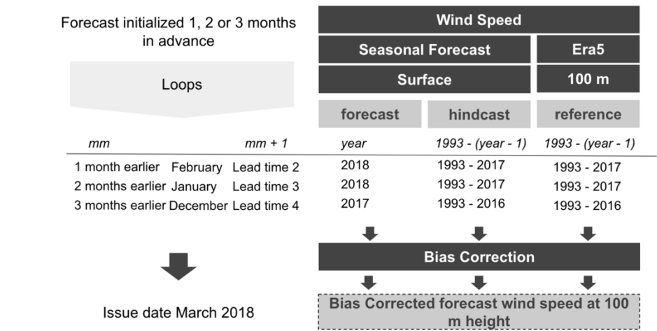
Figure 7: Scheme of the methodology applied. Grey boxes indicate the data, methods and results. The required parameters to analyse the March 2018 event are specified for the simulations initialized one, two and three month(s) in advance on white background.
