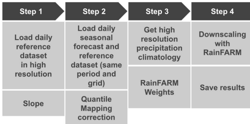
635 Figure 10: Scheme of the steps that need to be carried out to obtain and save a downscaled precipitation dataset. These steps are explained in detail in the text of the manuscript.
