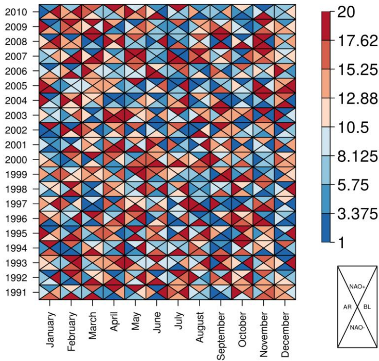
430 Figure 6: Example of the PlotTriangles4Categories using 4 different categories.
