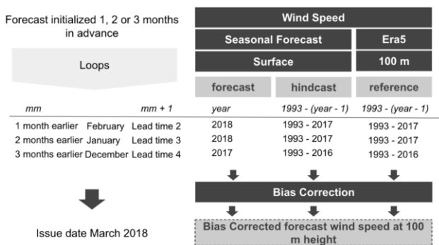
475 Figure 7: Scheme of the methodology applied. Grey boxes indicate the data, methods and results. The required parameters to analyse the March 2018 event are specified for the simulations initialized one, two and three month(s) in advance on white background.
