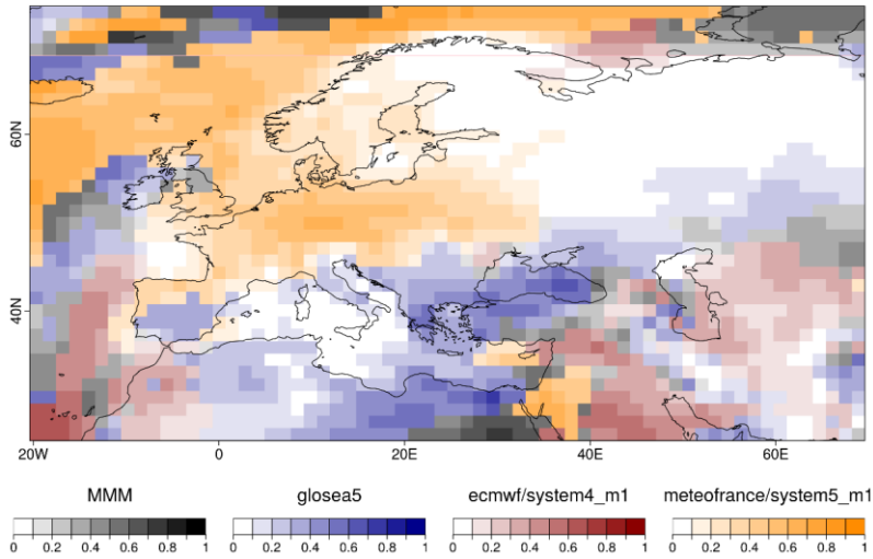
395 Figure 2: Example of Plot Combined Map result over Europe comparing different forecasts systems and the multi-model mean by colours and the highest correlation value in each grid point by colour intensity.
