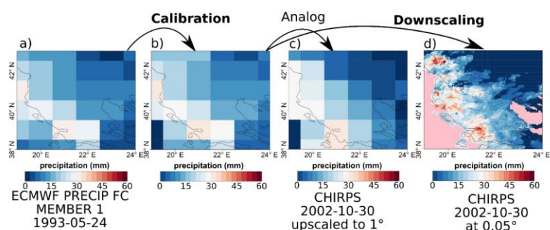
835 Figure 14: Comparison of the original forecast (a), bias-adjusted forecast (b), the analog (c) and the downscaled (d) forecast over Greece for SEAS5 for the 24th of May 1993.
