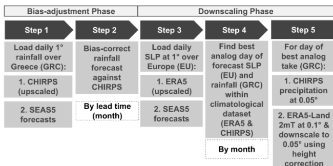
820 Figure 13: Scheme of the necessary steps to obtain bias adjusted and downscaled input. The abbreviations used are SLP, SEAS5, EU (Europe) and GRC (Greece).
