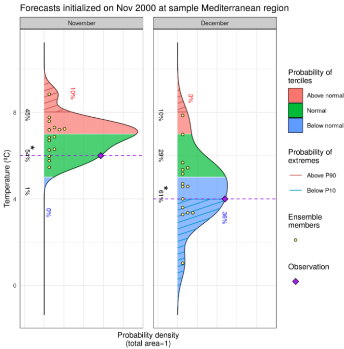
415 Figure 4: Example of PlotForecastPDF result using the lonlat_data sample provided along with CStools showing a possible comparison of two different lead times for a given forecast in a specific location. The individual ensembles (yellow dots), the corresponding observation (purple diamond), the probability of each tercile, i.e.: above normal (pink), normal (green) and below normal (blue); are annotated and the one with highest probability is marked with an asterisk and the extreme limits, i.e. above 90 percentile (red) and below 10 percentile (blue) correspond to the hatched areas and are also annotated.
