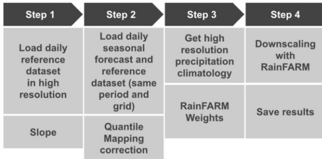
670 Figure 10: Scheme of the steps that need to be carried out to obtain and save a downscaled precipitation dataset. These steps are explained in detail in the text of the manuscript.
