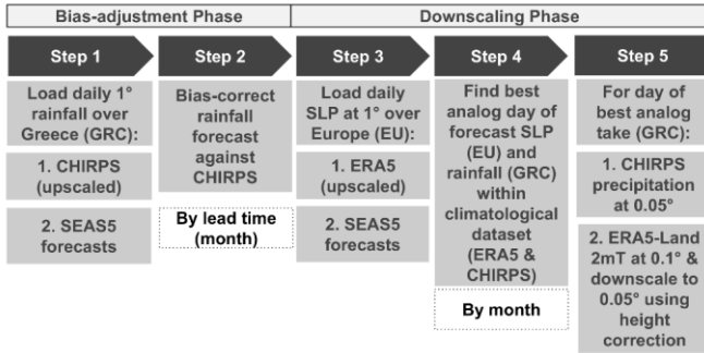
855 Figure 13: Scheme of the necessary steps to obtain bias adjusted and downscaled input. The abbreviations used are SLP, SEAS5, EU (Europe) and GRC (Greece).
